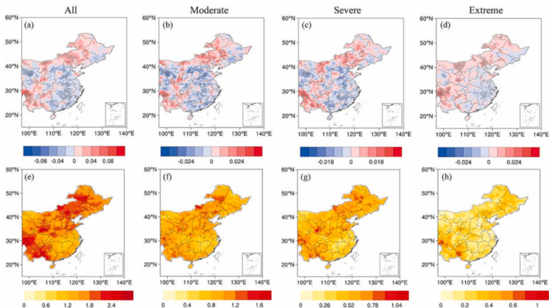
Fig. 6. Spatial distribution of trend (Units: times / year, gray shaded areas indicate grids with statistical significance at 95% confidence level) and multi-year average (Units: times) of CDHEs frequency in warm season from 1961 to 2018.
