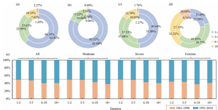
Fig. 10. The percentage of CDHEs with different durations to the total CDHEs in eastern China for (a) all severity, (b) moderate, (c) severe and (d) extreme CDHEs. (The inner circle of the pie chart represents the period of 1961–1990 and the outer circle represents the period of 1991–2018) (e) The ratio of the multi-year average frequency of CDHEs over the two time periods to the sum of the two time periods.
