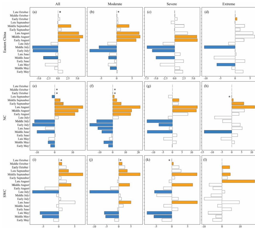
Fig. 11. Trend in five-year running mean of occurrence probabilities of CDHES in each ten days from May to October (histogram values are trends (value \times 10,000 / year), coloured and asterisked bars indicate the statistical significance of the trends at 95% confidence level).
