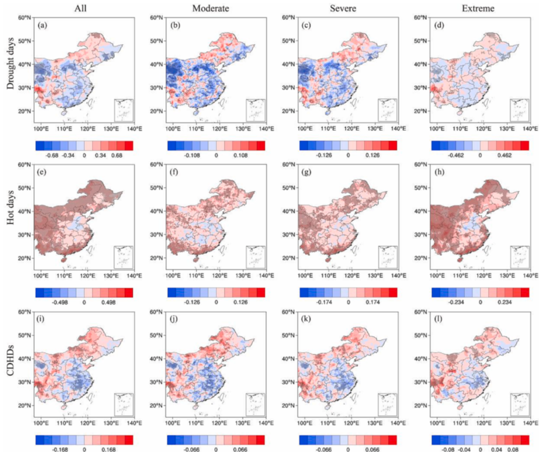
Fig. 2. Spatial distribution of trend in the number of drought days, hot days and CDHDs for the warm season from 1961 to 2018. (Units: days / year, gray shaded areas indicate grids with statistical significance at 95% confidence level).
