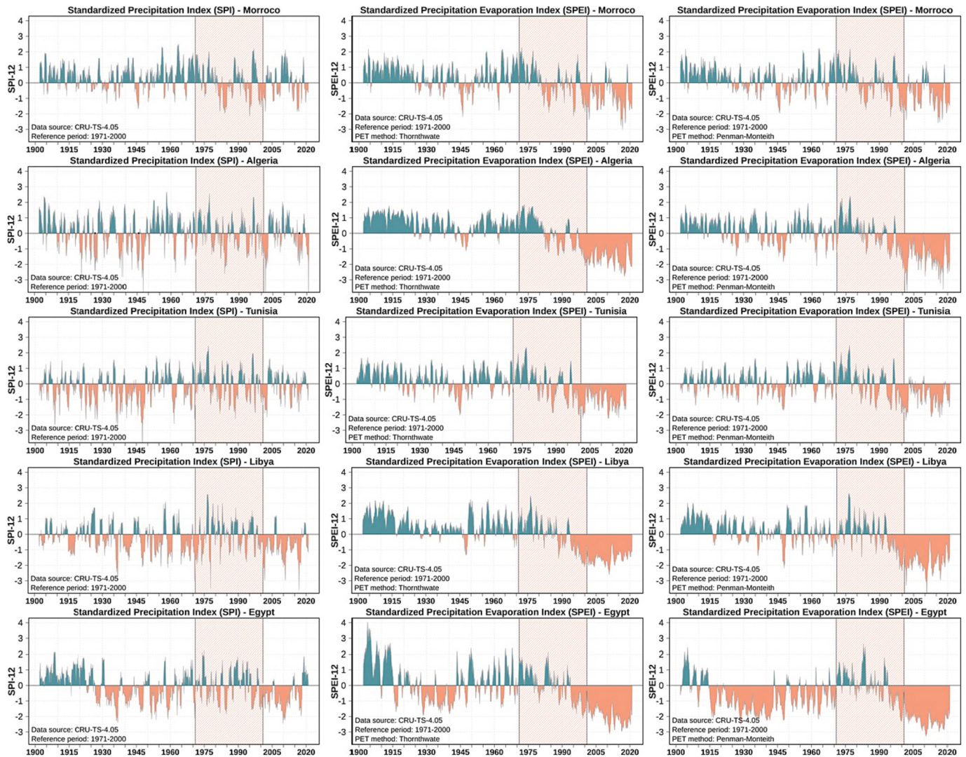
Fig. 4. Observed time series of the Standardized Precipitation Index (SPI-12 – left panels) and the Standardized Precipitation Evapotranspiration Index (SPEI-12 – middle and right panels) at 12-month accumulation periods for five North Africa countries. The SPEI-12 has been calculated using the Thornthwaite (middle panels) and Penman-Monteith methods (right panels).
