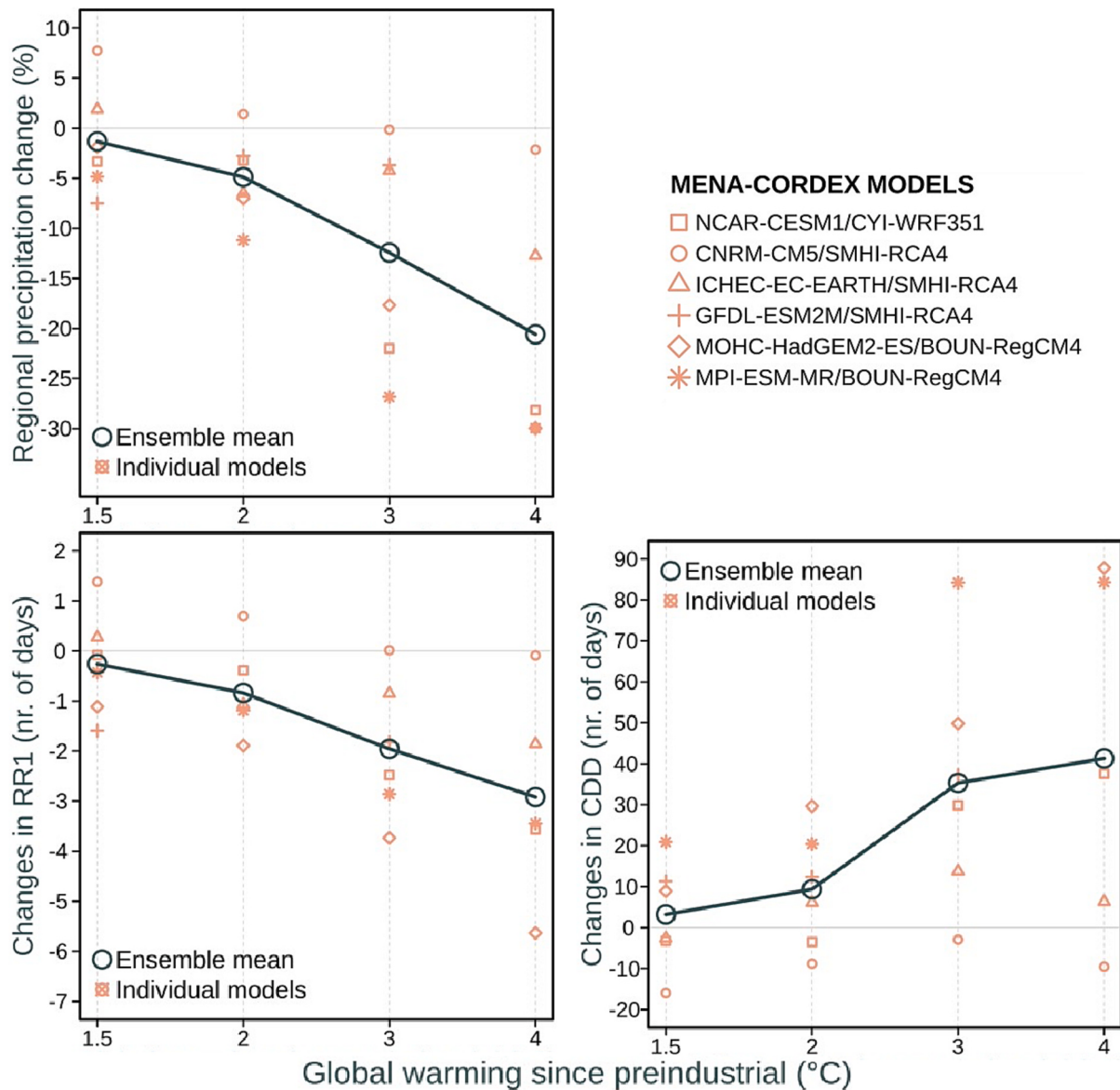
Fig. 5. Precipitation (top panel), RR1 (rainy day per year) changes and Consecutive dry days CDD (with respect to the 1971–2000 reference period) over NAF for various global warming levels.
