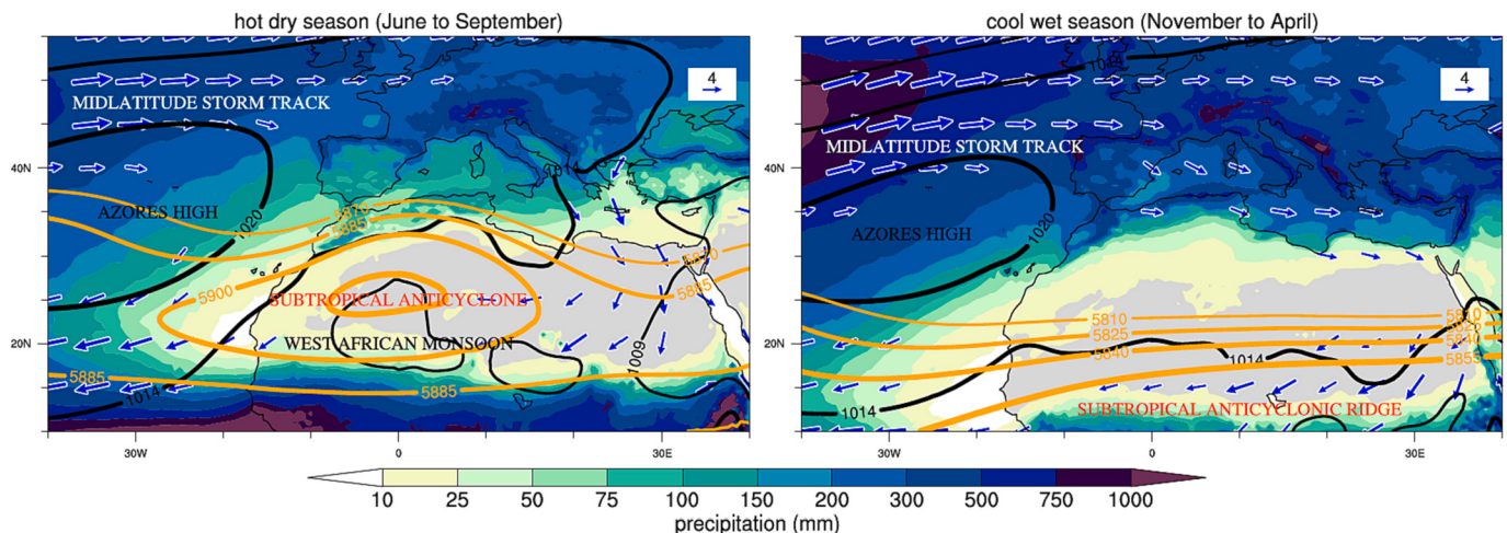
Fig. 3. Precipitation and the atmospheric circulation over NAF during (left) the hot dry summer season, June–September, and (right) the cool wet season, November – April. The data is based on monthly means from ERA5 for the period 1979–2021 and shows accumulated precipitation (mm; shading) and the average monthly means of sea level pressure (hPa; black contours), 500-hPa geopotential height (gpm; orange contours), and the 850-hPa horizontal wind ( \text{m s}^{-1} ; blue vectors where its magnitude >4 \text{ m s}^{-1} ). The atmospheric circulation patterns noted in the figure are discussed in the text. (For interpretation of the references to color in this figure legend, the reader is referred to the web version of this article.)
