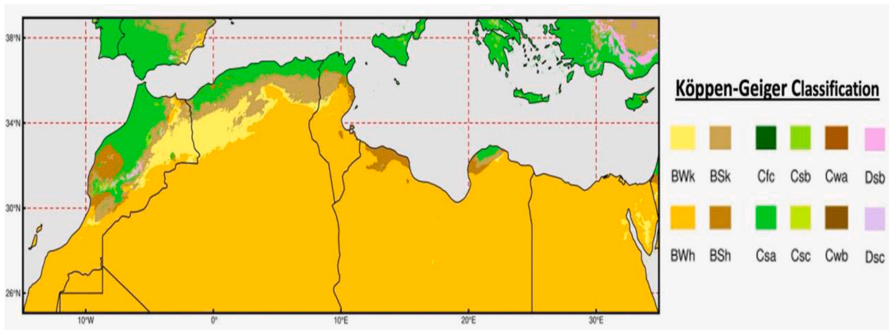
Fig. 1. Climate types over North Africa based on the Köppen–Geiger climate classification system, 1980–2016 (Data source: Beck et al., 2018).
