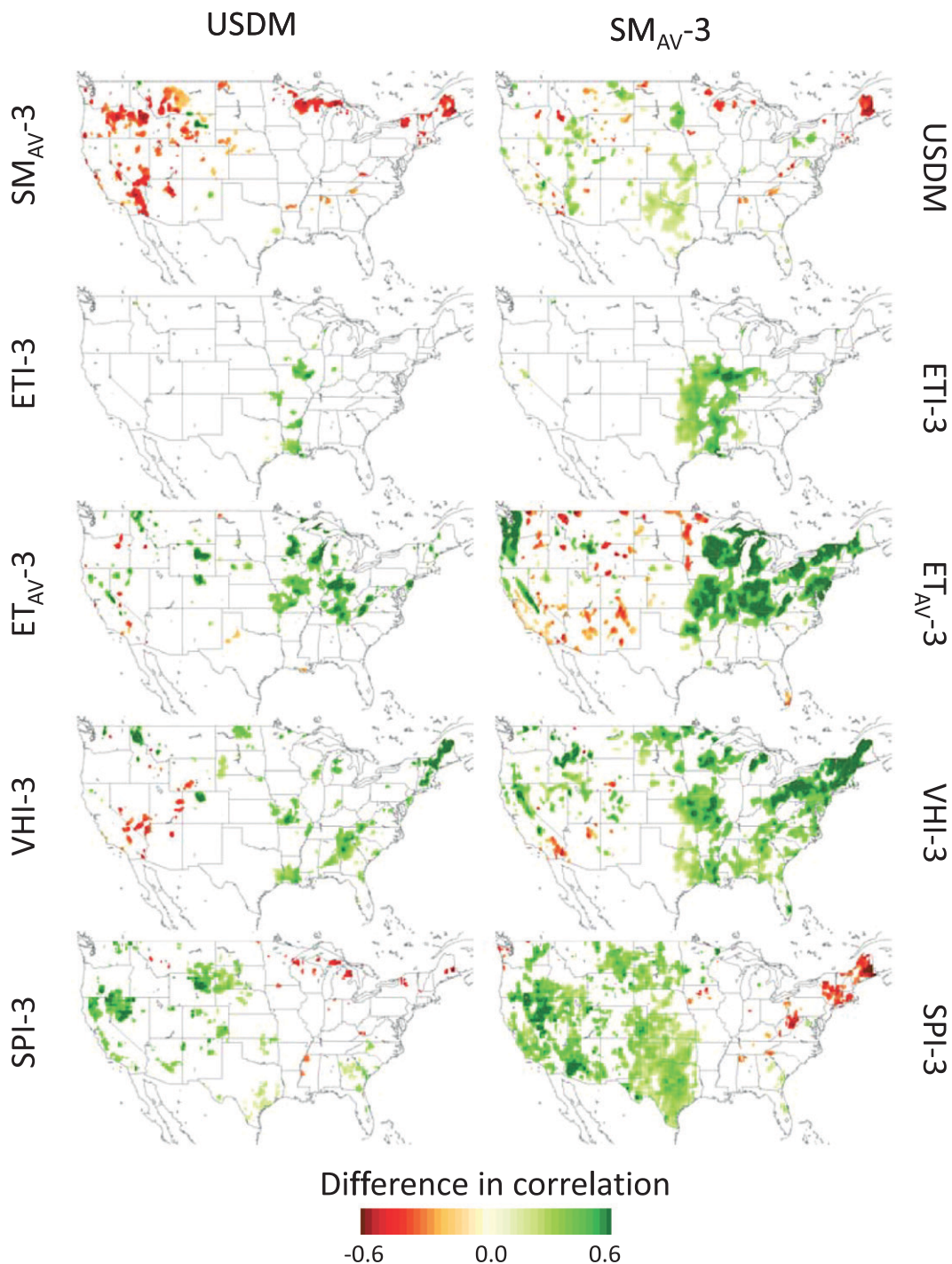
FIG. 8. Difference in interindex temporal correlation computed as r(\text{ESI-3}) - r(x) , where r(\text{ESI-3}) is the temporal correlation between ESI-3 and (left) USDM or (right) SM AV-3 and r(x) is the correlation between index x and USDM or SM AV-3 . Comparison indices x include (second row) ETI-3, (third row) ET AV-3 , (fourth row) VHI-3, and (bottom row) SPI-3. Green shading indicates r(\text{ESI-3}) > r(x) . Only pixels with significant ( p < 0.05 ) correlation differences are displayed.
