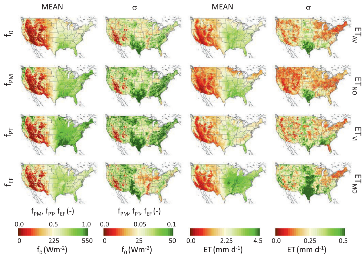
FIG. 4. (left two columns) Climatological mean and standard deviation maps for several ALEXI [ f_0 ( \text{W m}^{-2} ) and f_{\text{PM}} , f_{\text{PT}} , and f_{\text{EF}} (unitless)] and (right two columns) NLDAS ET-related indicators ( \text{mm d}^{-1} ) included in the intercomparison, computed from 26-week (April–September) composites over the period 2000–11.
