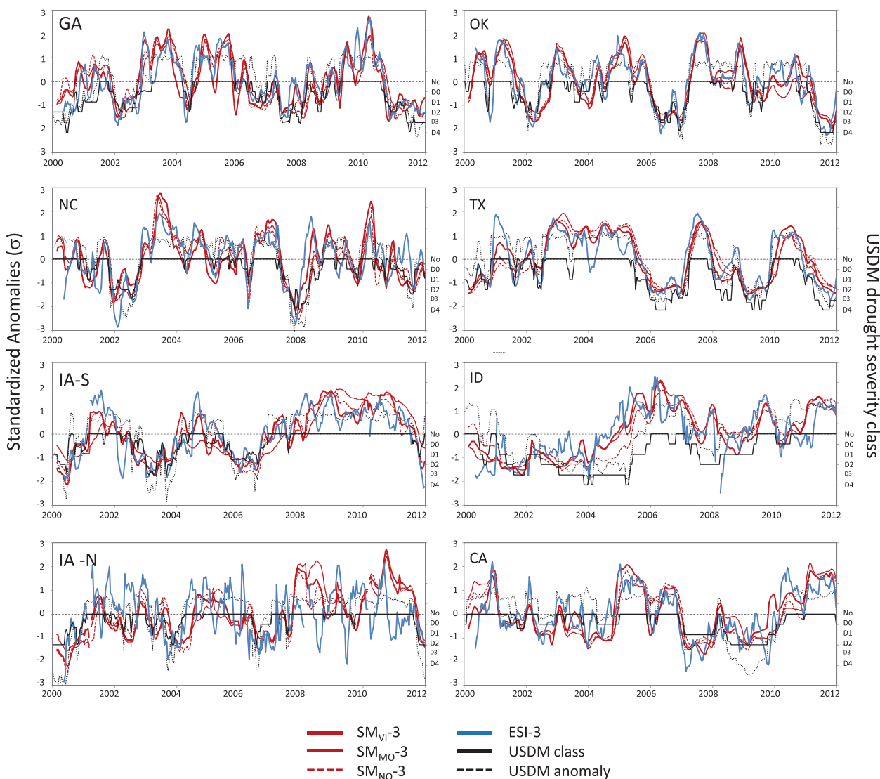
FIG. 10. Time series of ESI-3; anomalies in SM NO -3, SM MO -3, and SM VI -3; and USDMS drought classes and anomaly values for several sites across CONUS (Fig. 2), averaged over 50 \text{ km} \times 50 \text{ km} boxes. In each panel, standardized anomalies are associated with the left vertical axis (in units of \sigma ), and USDMS class with the right vertical axis.
