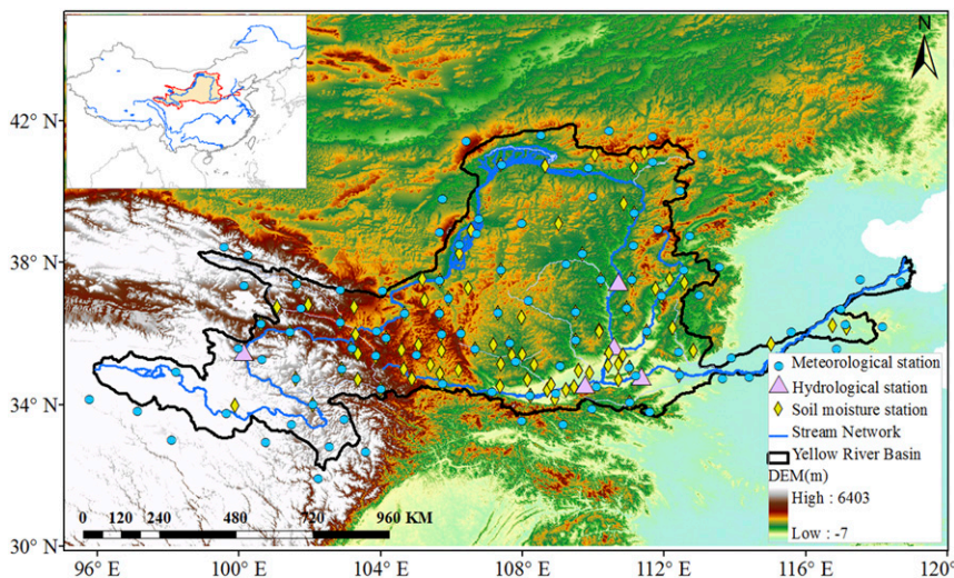
FIG. 1. Spatial distribution of national meteorological stations, soil moisture observation sites, and hydrological stations over the Yellow River basin (YRB).
