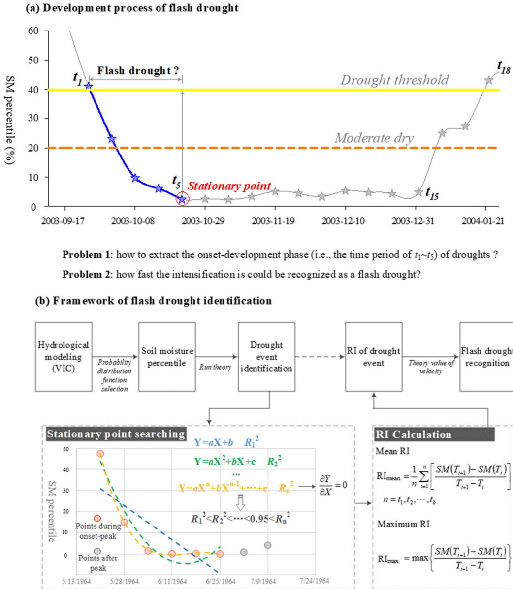
FIG. 2. (a) Schematic overview of the evolution process of flash drought indicated by soil moisture percentile; t_1 represents the onset time; t_5 denotes the stationary point where rapid depletion of soil moisture ends; the period from t_6 to t_{18} represents the recovery stage where soil moisture increases gradually then returns to the normal condition. (b) Generalized flowchart of identifying flash drought based on intensification rate. The left dashed rectangle shows how find the stationary point with the polynomial fitting method. The left rectangle gives the formulas for calculating the rate of intensification.
