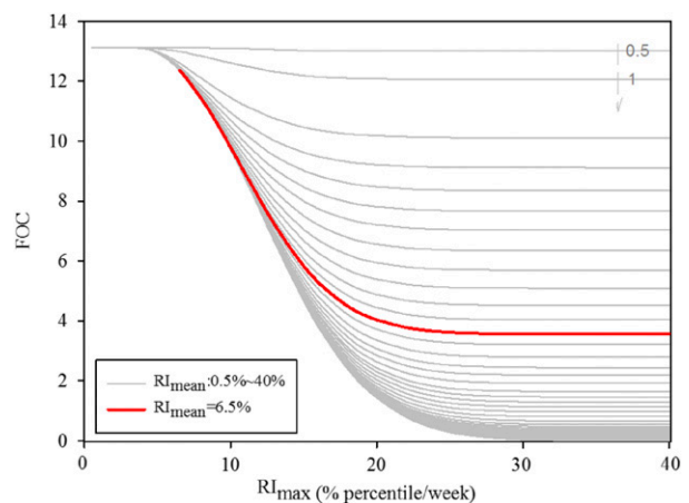
FIG. 4. Sensitivity analysis on the frequency of occurrence (FOC) of flash droughts to varied RI_{\text{mean}} and RI_{\text{max}} . The gray solid lines show the relationship between RI_{\text{max}} and FOC under different values of RI_{\text{mean}} (increasing gradually from 0.5 to 40 percentile per week). Likewise, the red solid line gives the case when RI_{\text{mean}} = 6.5 percentile per week.
