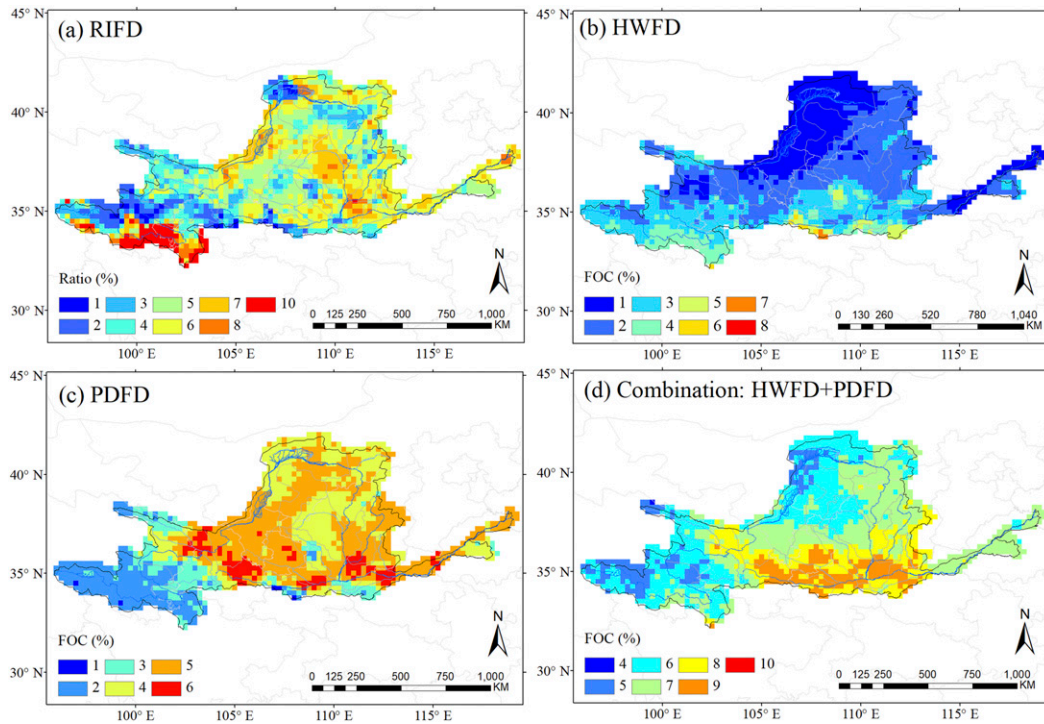
FIG. 8. Spatial distribution of the FOC for flash droughts indicated by (a) RIFD, (b) HWFD, (c) PDFD, and (d) sum of HWFD and PDFD (i.e., events of HWFD and PDFD were merged into a new sample for calculating FOC).
