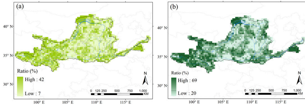
FIG. 5. (a) The ratio of nondrought events (viz., for an identified flash drought event, the soil moisture values at each week are all higher than the 30th percentile) to all events identified by HWFD and PDFD. (b) As in (a), but for the ratio of nonmoderate drought events (higher than the 20th percentile) to all events.
