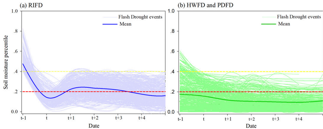
FIG. 6. Variation of soil moisture percentile for major flash drought events (light colored lines; excludes drought duration less than 4 weeks) of all grids in the study region identified by (a) RIFD and (b) HWFD and PDFD. The dark color line represents the ensemble-mean of all flash drought events. The t represents the time when the flash droughts occur. The t - 2 and t - 1 denote the 1 week and 2 weeks prior to t , while t + 1 – t + 4 represent the lagged 1–4 weeks of t , respectively.
