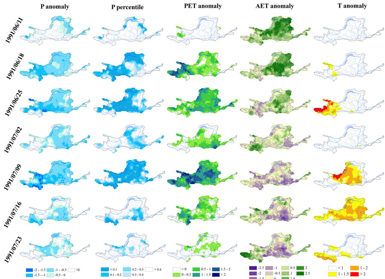
FIG. 11. Spatial anomalies of related meteorological variables for the 1991 flash drought.
