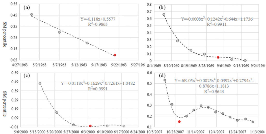
FIG. 3. Four typical examples of the attenuation process of soil moisture percentile (from the onset time to the peak of drought intensity) under drought. Based on the trajectories of soil moisture percentile, we use different order polynomials to fit these samples, and the red circles can be derived as the stationary point (when the partial derivative of the fitted polynomial equation is 0) of the established polynomial. When a linear regression function is employed, the peak of drought intensity is the stationary point.
