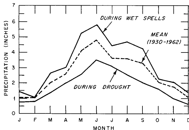
FIGURE 5.—Mean monthly precipitation in central Iowa.
