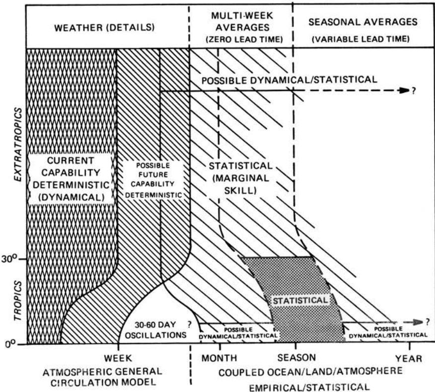
Fig. 3 Schematic representation of the nature of atmospheric predictability (suggested by Winn Neilsen, Vatican City, 1986).
