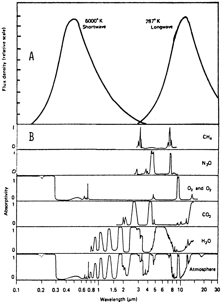
Fig. 2 (a) Spectra of solar and terrestrial radiation scaled to their maximum flux densities; (b) absorption spectra for important constituent gases of the atmosphere. Note the log-scale of the common abscissa (adapted from Reifsnnyder and Lull, 1965; and Fleagle and Businger, 1963).
