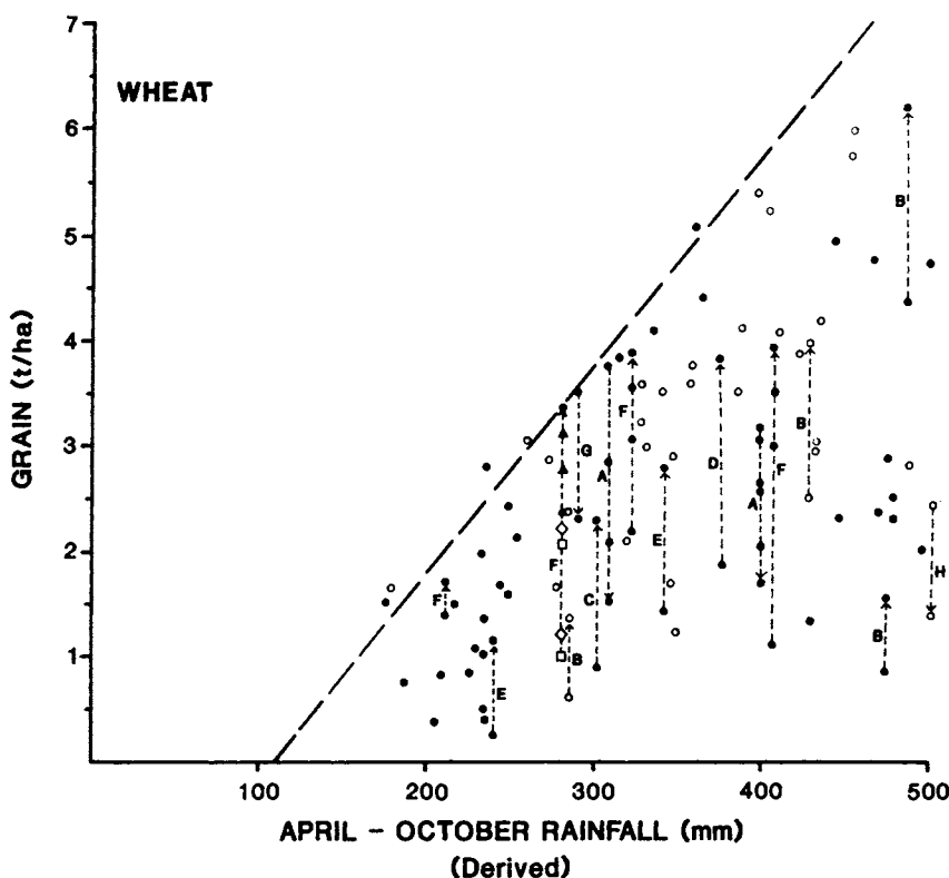
Fig. 5 The relation between grain yield of wheat and the estimate of water use. The black dots are results from experiments, the open circles from farmers' fields. Yield increases were obtained from the application of nitrogen (points linked by a B line), phosphorus (C line), copper (D line), control of eelworms (E line), and multifactors (F line). Yield decreased because of delayed time of sowing (A line), weeds (G line), and waterlogging (H line) (from French and Schultz, 1984b).
