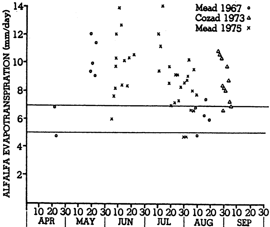
Fig. 9 Daily total of evapotranspiration (ET) by alfalfa well supplied with water. The band indicates the range of daily ET that can be attributed to net radiation. The excess is attributable to sensible heat advection (from Rosenberg, 1982).
