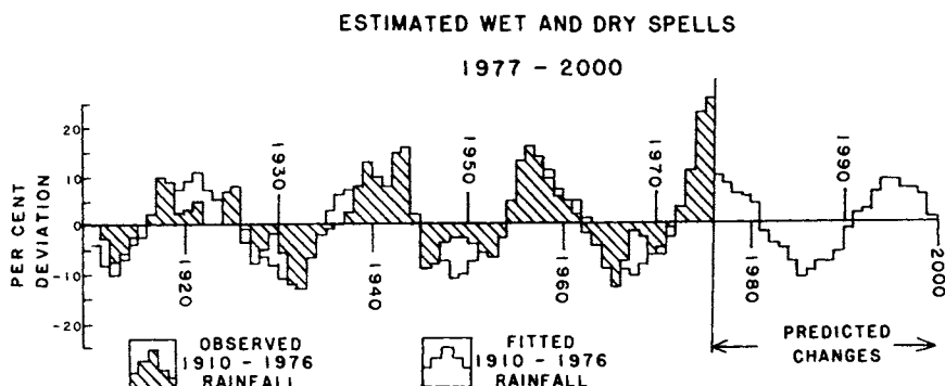
Fig. 5 Possible future extended wet and dry spells over the summer rainfall region of southern Africa (after Tyson and Dyer, 1978).
