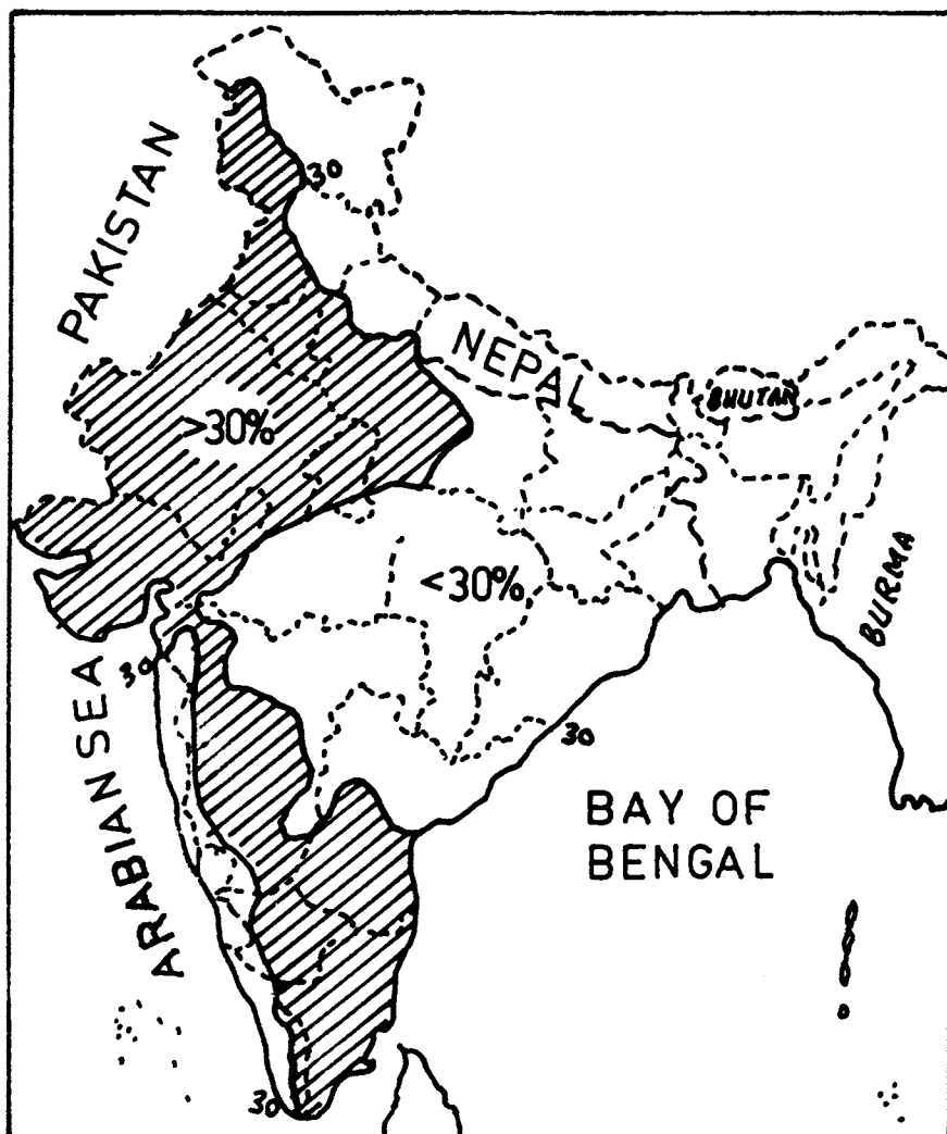
Fig. 1 Drought-prone areas in India (from Sarkar, 1979).
