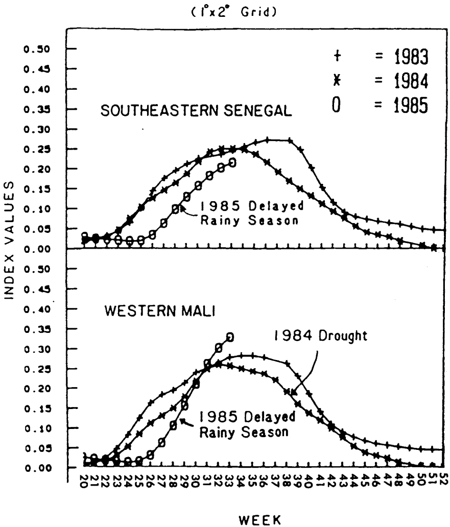
Fig. 6 The smoothed normalized vegetation index for southeastern Senegal and western Mali in 1983, 1984, and 1985. Note the reduced vegetation for 1984 and the delayed 1985 rainy season.
