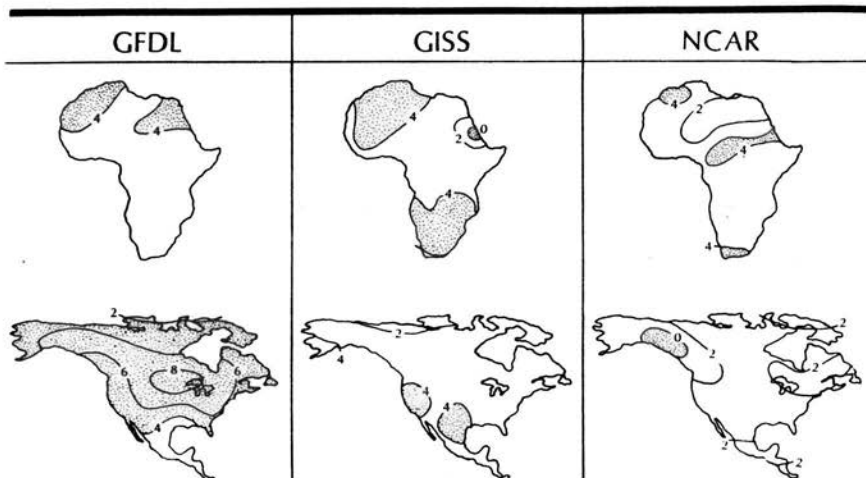
Fig. 3 The distribution of surface air temperature change ( ^{\circ}\text{C} ) for a doubling of atmospheric carbon dioxide concentration for June, July, and August, simulated by the global climatic models of GFDL (left), GISS (center), and NCAR (right). Stipple indicates temperature increases greater than 4^{\circ}\text{C} (redrawn from Fig. 4.39 of Schlesinger and Mitchell, 1985).
