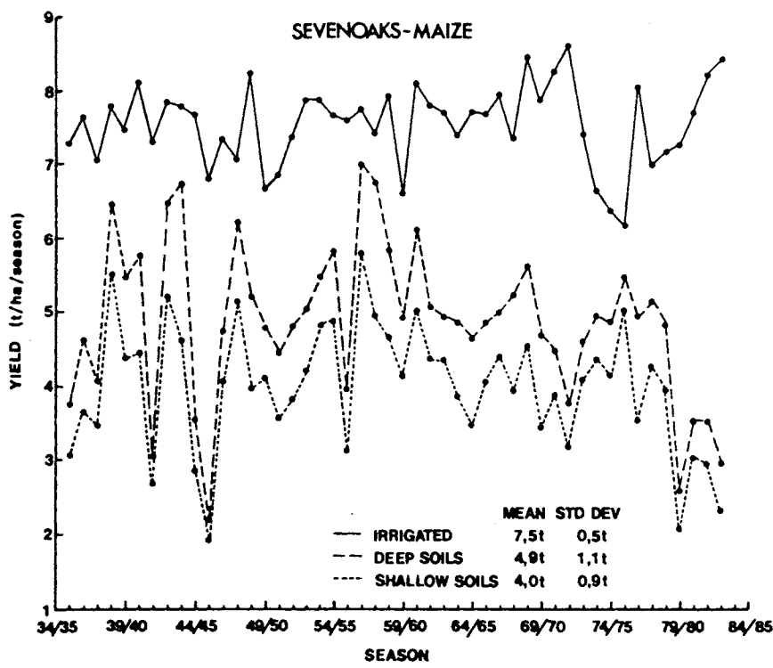
Fig. 3 Maize yield simulations under different conditions at Sevenoaks, Natal (Schulze, 1986).
