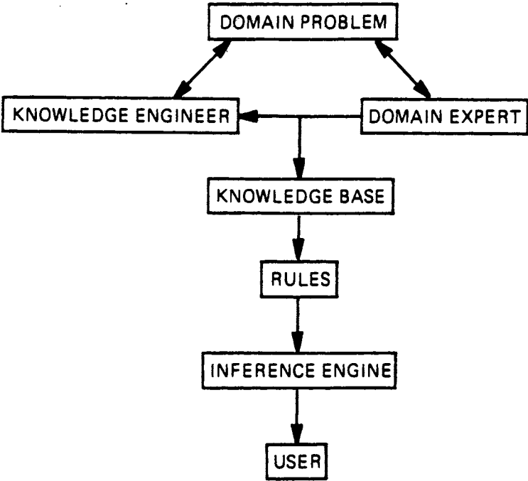
Fig. 1 Typical expert system architecture.
