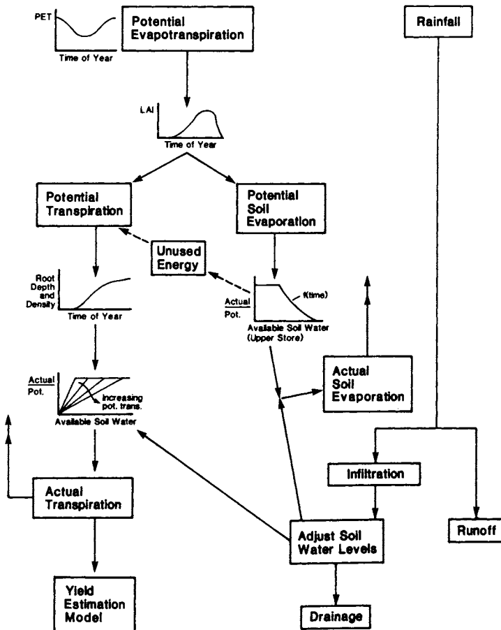
Fig. 1 Schematic of Water Balance (WETBAL) Model.
