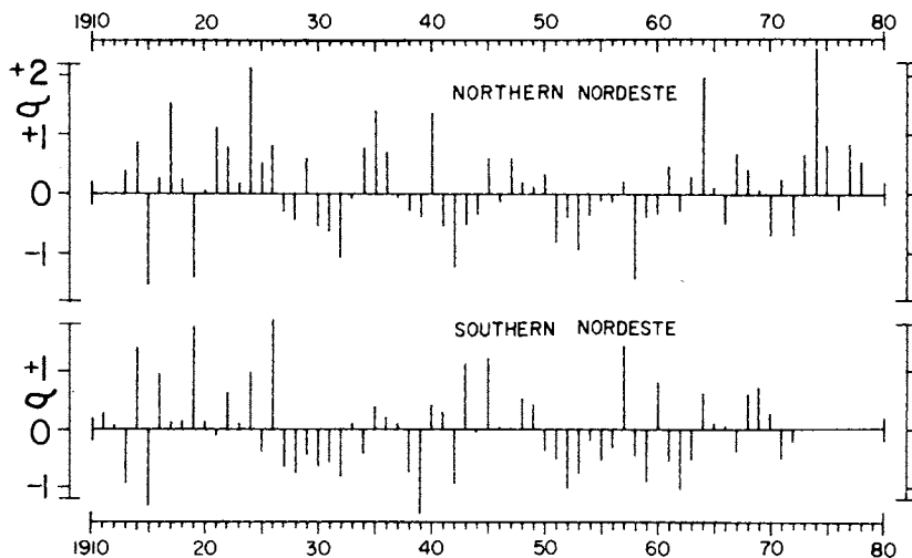
Fig. 4 Average of normalized departure of annual rainfall for all stations in the northern and southern Nordeste.
