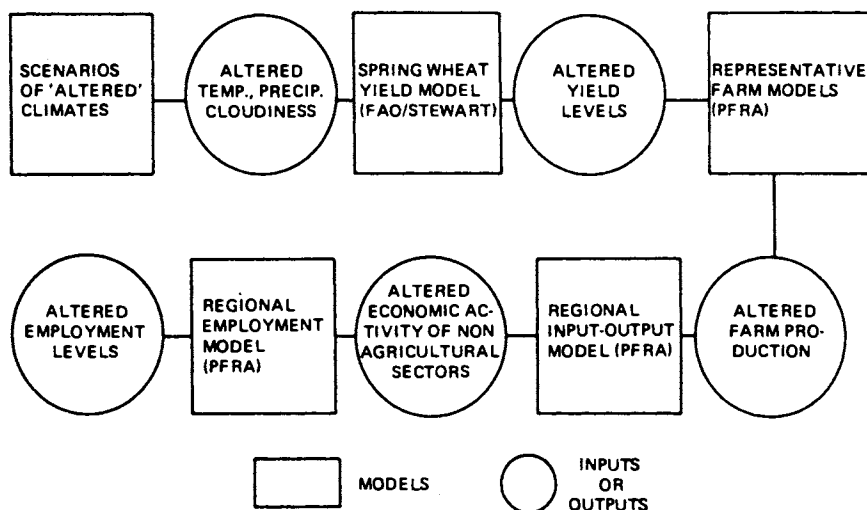
Fig. 13 Hierarchy of models for assessing impacts of climatic change in Saskatchewan (after Williams, et al., 1987).
