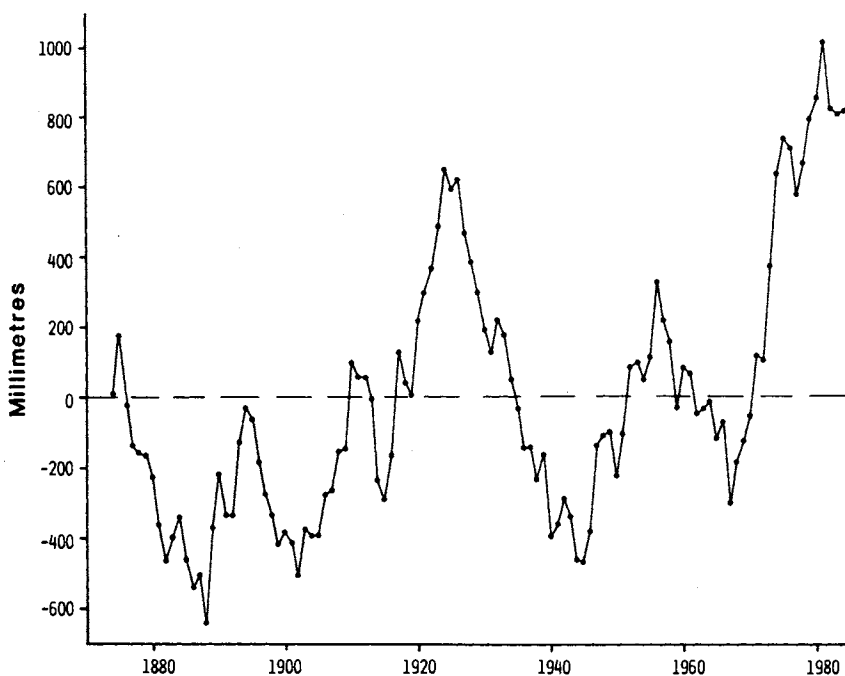
Fig. 2 The cumulative sum of the deviations of the monthly rainfall from the long-term mean for each month for Georgetown. The point for each year is the December value.
