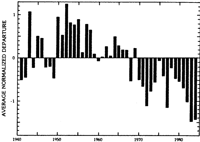
Fig. 1 Departures from normal rainfall in sub-Saharan Africa, 1941-85 (Lamb, 1982, 1983; updates shown in Glantz, 1986).
