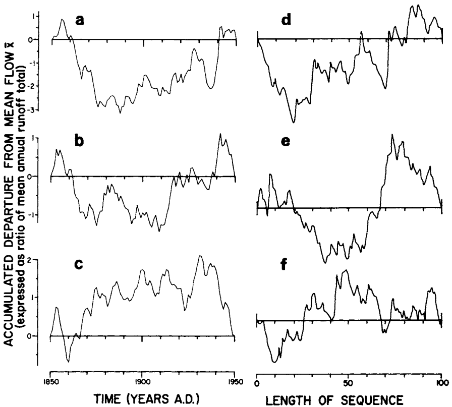
Fig. 2 Residual mass curves of three 100-year series of mean annual flows and of three samples of 100 random numbers: a—Elbe River, Děčín, Czechoslovakia; b—Danube River, Orsova, Romania; c—Gota River, Vanersborg, Sweden (from Klemeš, 1982a); d, e, f—random samples.
