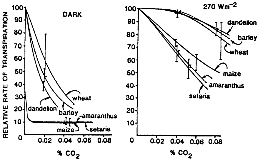
Fig. 13 Effect of CO 2 concentration on transpiration of C 3 and C 4 species in light and darkness (after Akita and Moss, 1972).
