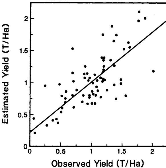
Fig. 3 Grain yield analysis using data from an area of 4,000 km 2 in the Gunnedah region, 1896-1970.
