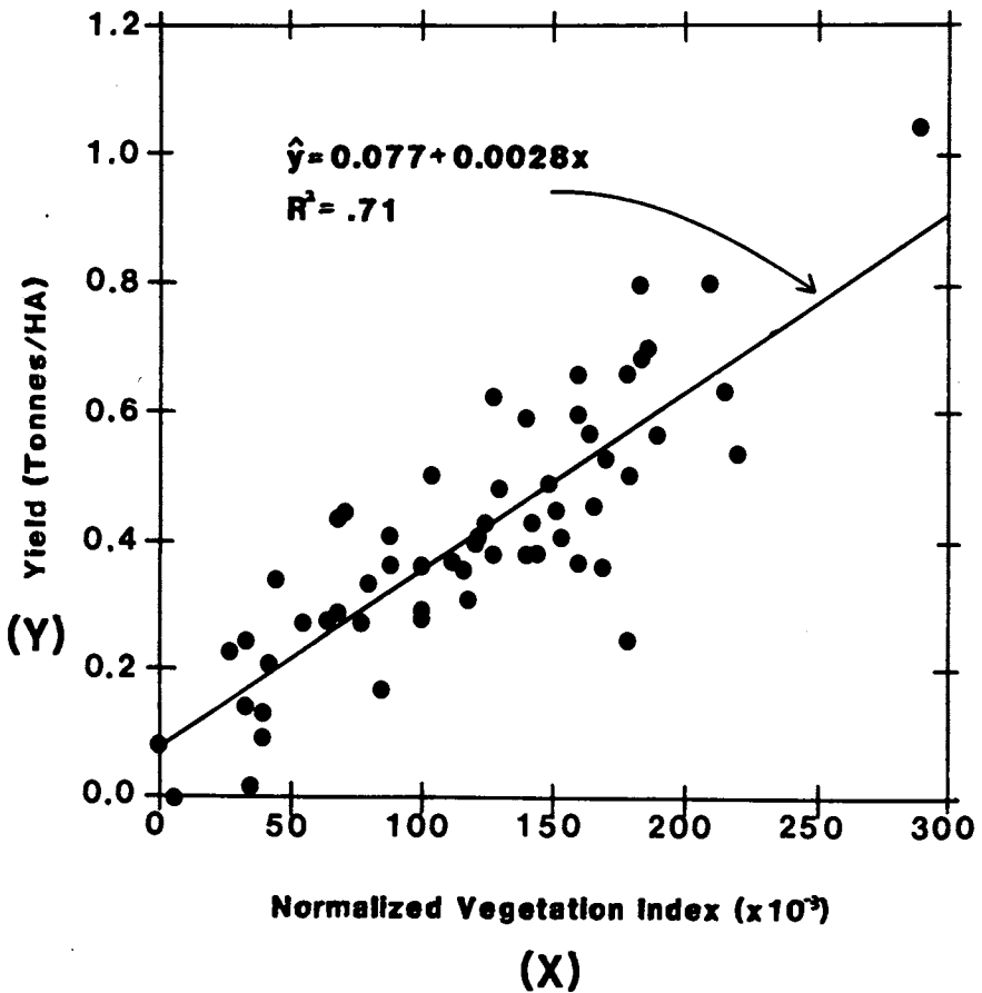
Fig. 8 Sahel millet yield model as a function of normalized vegetation index.
