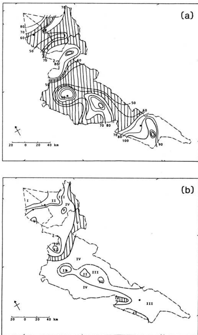
Fig. 4 (a) Rainfall as a percentage of normal in October-December 1976. (b) Agroclimatic zones in October-December 1976.
