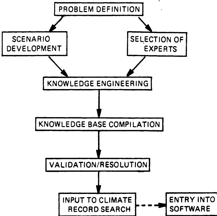
Fig. 2 CLIMPAX expert system approach.
