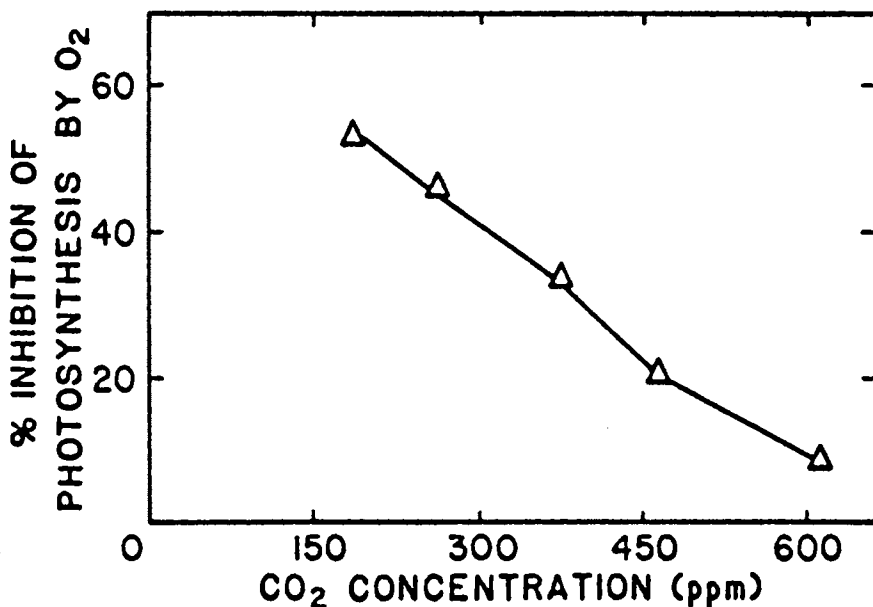
Fig. 11 Inhibition of photosynthesis in potato leaves by 21% (air) at increasing CO 2 levels (from Lemon, 1983, Chap. 2).
