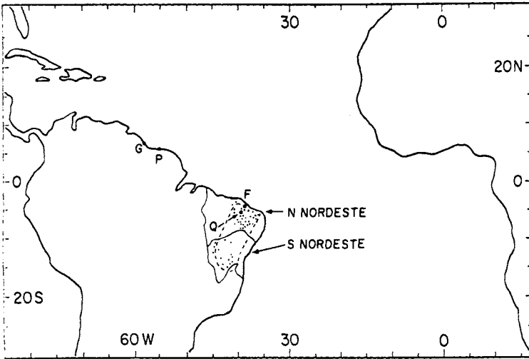
Fig. 2 Orientation map showing northern and southern Nordeste and stations Fortaleza (F) and Quixeramobim (Q).
