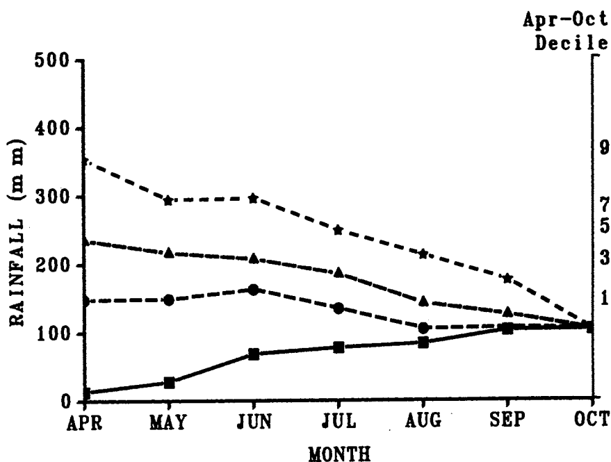
Fig. 3 A method for predicting the trend in rainfall during the growing season (April-October) at Kimba, South Australia. The actual rainfall to the end of each month is added separately to the rainfall for deciles 9, 5, and 1 for the remaining months of the growing season.
