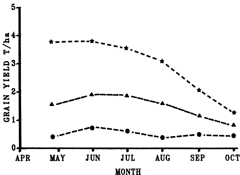
Fig. 4 The estimate of wheat yield, using a simple growth model and the updated rainfall estimates outlined in Fig. 3.
