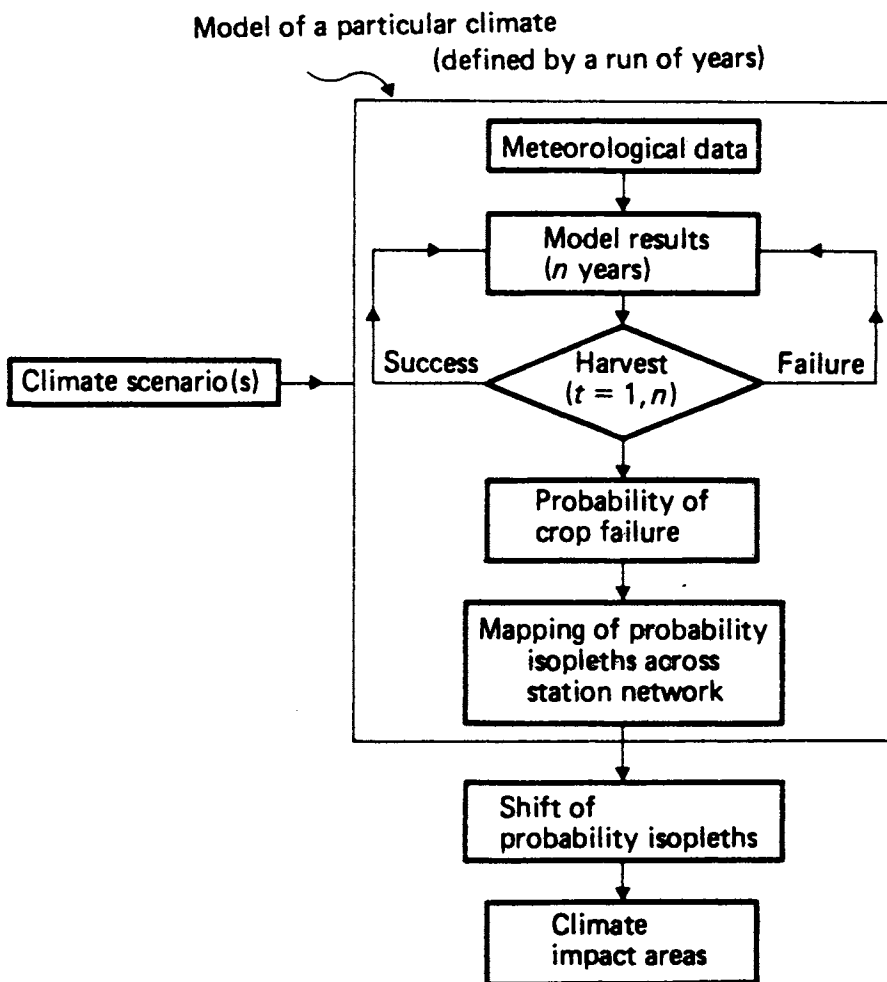
Fig. 9 Steps in the identification of climate impact areas. The weather for a particular year, described by a set of meteorological data, is translated into a measure of annual return on an activity (e.g., harvest failure or success) using an appropriate model. Over a period of years, the frequency (probability) of loss or benefit can be assessed at each of a number of locations and mapped geographically as isopleths. Scenarios of changing climates can then be used as inputs to the model and the probability isopleths can be remapped. The geographical shifts of the isopleths thus delimit areas of specific climate impact (Parry and Carter, 1984).
