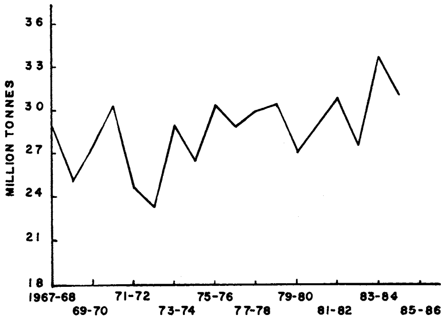
Fig. 4 Coarse cereals production (D E & S, Government of India).
