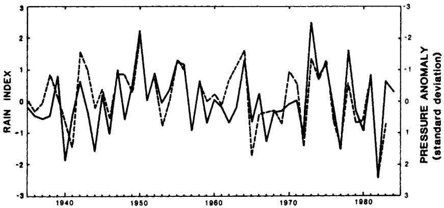
Fig. 5 Time series of east Australian winter-spring rain index (full line) and winter-spring mean sea-level pressure anomalies at Darwin (broken line, scale reversed).
