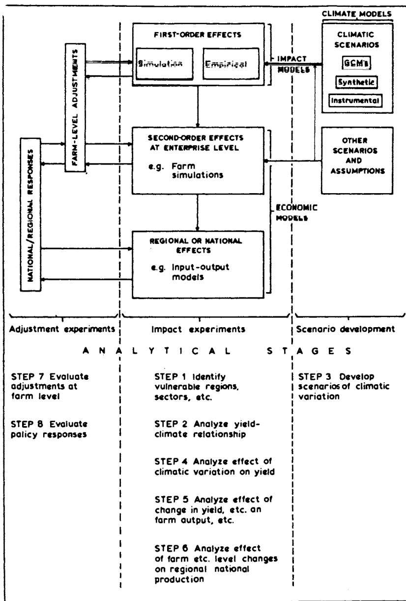
Fig. 8 Conceptual framework and stages of analysis adopted in the IIASA/UNEP project (Parry and Carter, 1987).
