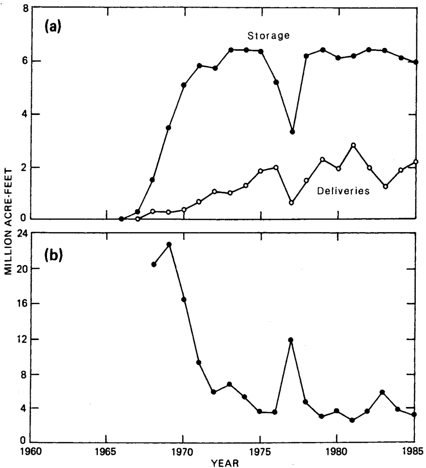
Fig. 7 State Water Project (a) maximum annual storage and total deliveries and (b) ratio of storage to deliveries.
