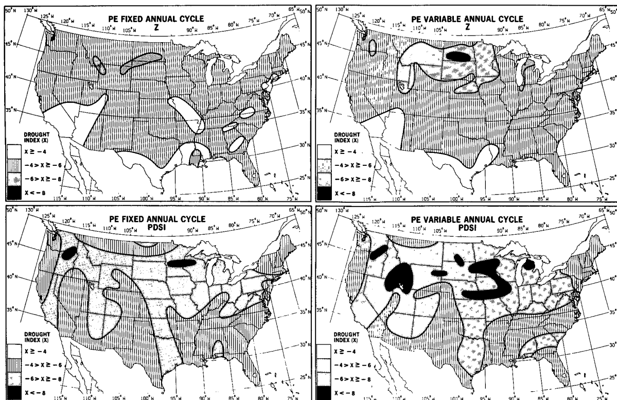
FIG. 3. Lowest PDSI and Z-index when the annual cycle of PE is artificially held constant from year-to-year vs a variable annual cycle of PE.
