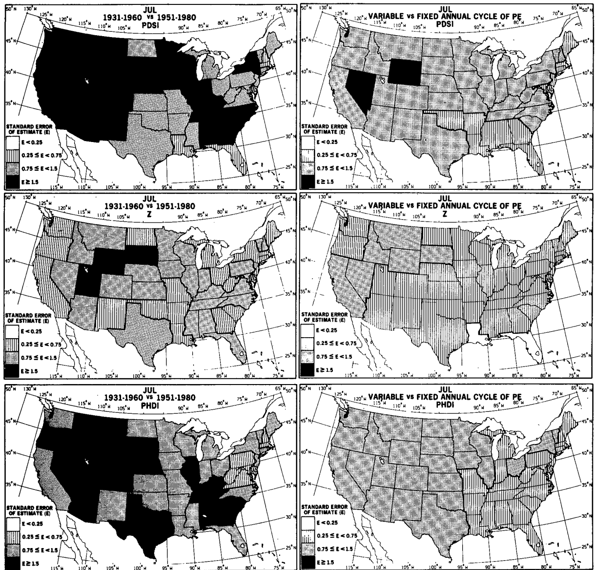
FIG. 4. Statewide averages of the standard errors of estimate between the PDSI, PHDI, and the Z-index for two different calibration periods, and when the annual cycle of PE is artificially held constant from year-to-year vs a variable annual cycle of PE.
