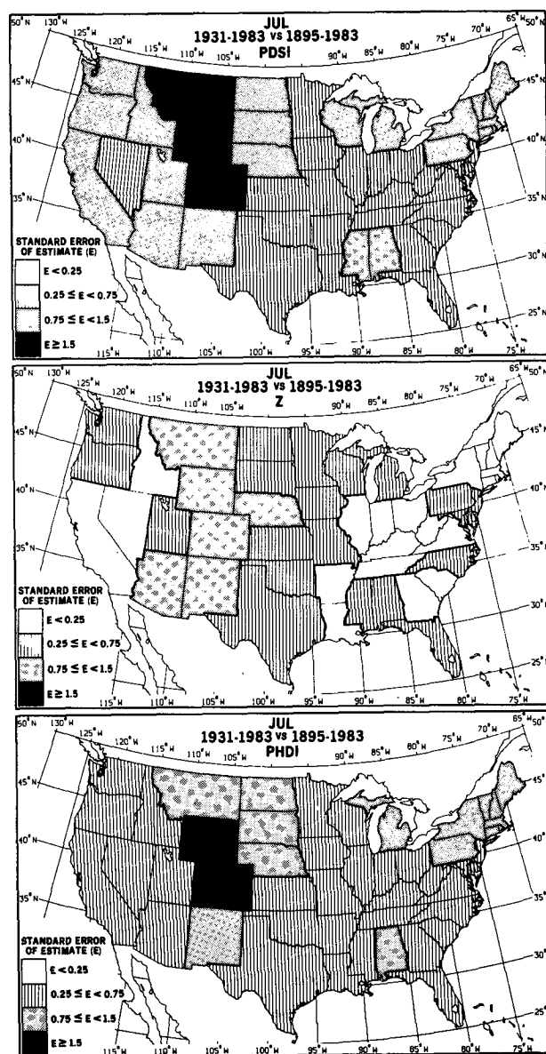
FIG. 5. Statewide averages of the standard errors of estimate between the PDSI, PHDI, and the Z-index for two different calibration periods.
