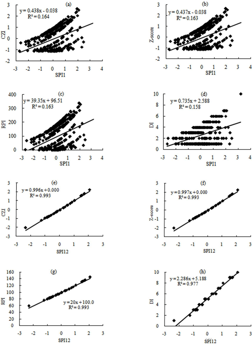
Figure 5. Scatter diagrams of the SPI and precipitation-based drought indices (CZI,Z-score,RPI,DI) (a),(b),(c) and (d) on 1-month time scale; (e),(f),(g) and (h) on 12-month time scale 149x200mm (600 x 600 DPI)
