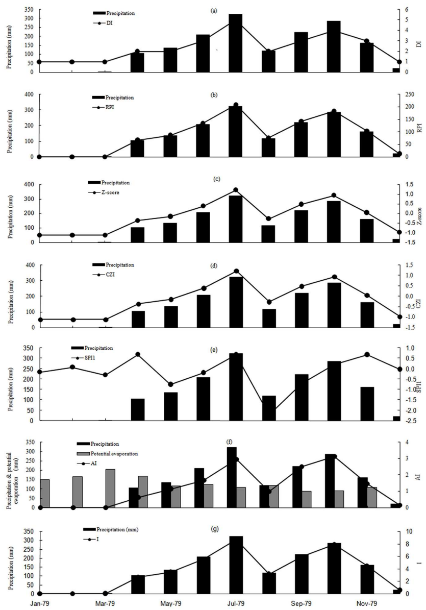
Figure 3. Seven drought indices and precipitation and potential evaporation on 1-month time scale in 1979 in Tay Ninh station 179x253mm (600 x 600 DPI)
