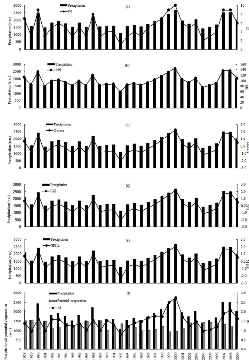
Figure 4. Six drought indices and precipitation and potential evaporation on 12-month time scale in Bien Hoa station 182x259mm (600 x 600 DPI)
