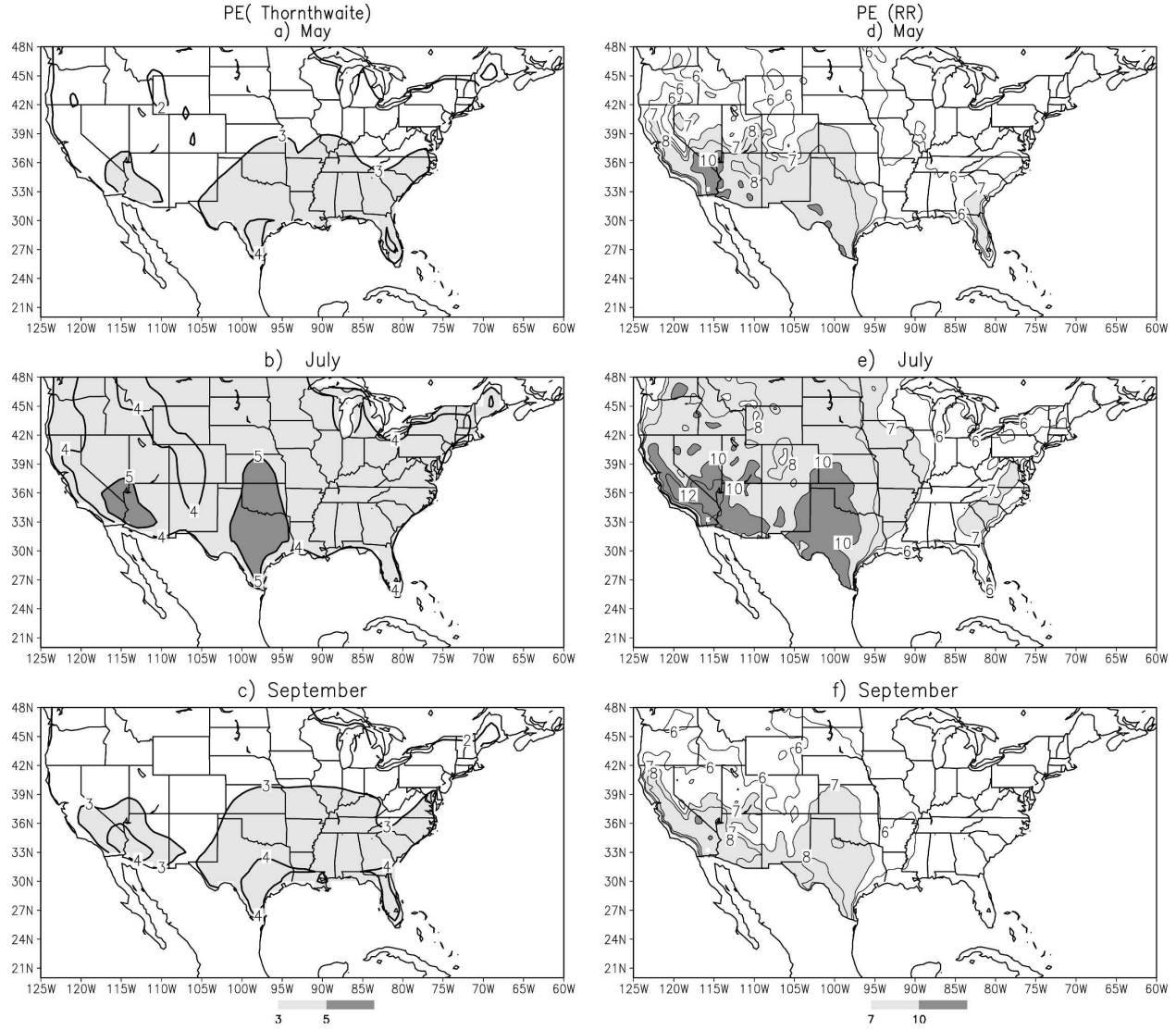
FIG. 1. The evapotranspiration (PE) for (a) May, (b) July, and (c) September averaged for the period of 1979–2004 based on the Thornthwaite formula. Contour interval is 1 mm day -1 . Values greater than 3 (5) mm day -1 are shaded light (dark), (d)–(f) Same as (a)–(c), but from the RR. Values greater than 7 (10) mm day -1 are shaded light (dark).
