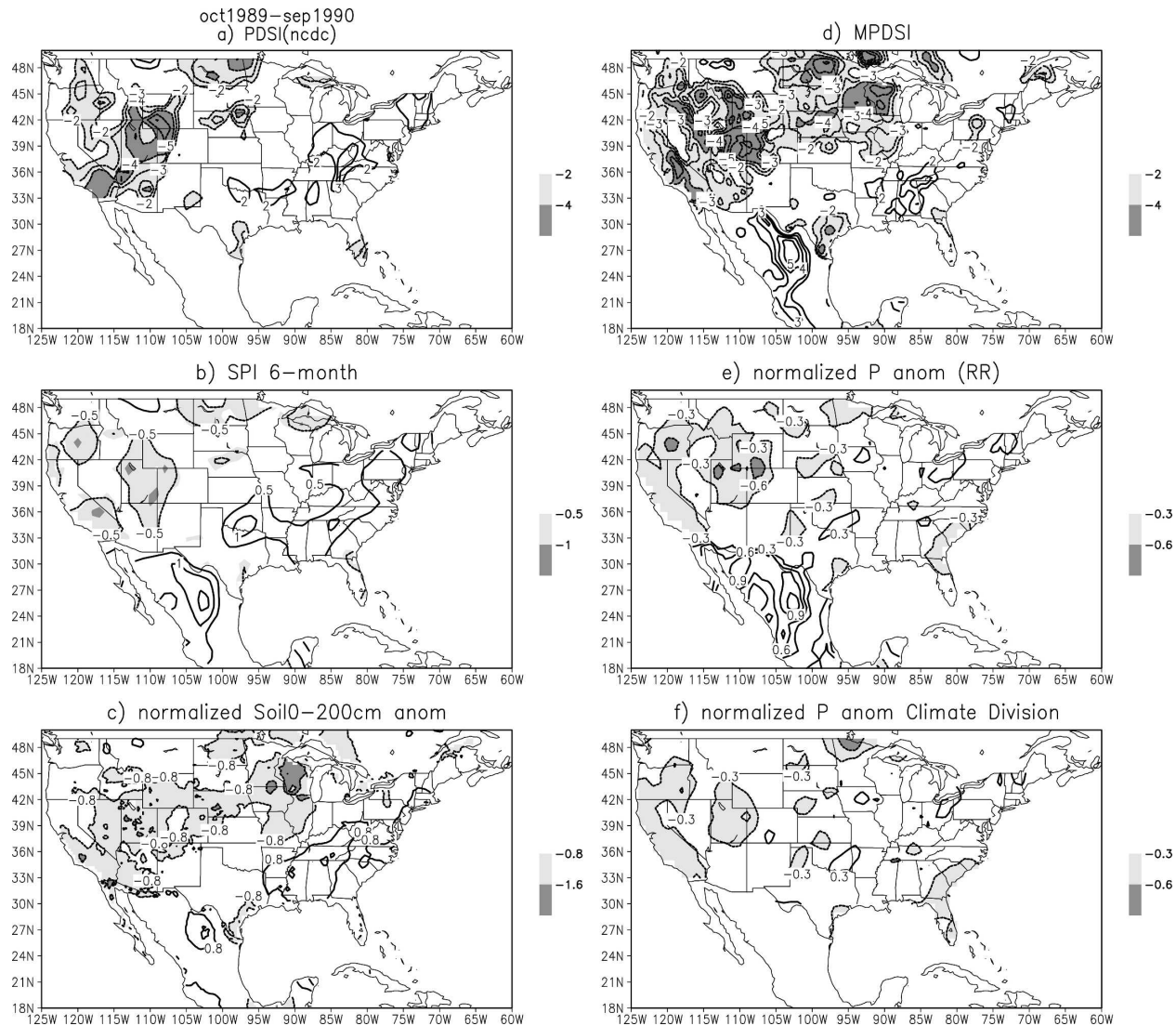
FIG. 7. (a) PDSI(ncdc) averaged for October 1989–September 1990. Contour interval is 1, with the 0, 1, and -1 contours omitted. Values less than -2 ( -4 ) are shaded light (dark). (b) Same as (a), but for SPI6. Contour interval is 0.5. Values less than -0.5 ( -1 ) are shaded light (dark). (c) Same as (b), but for normalized soil moisture anomaly from 0 to 200 cm. Contour interval is 0.8. Values less than -0.8 ( -1.6 ) are shaded light (dark). (d) Same as (a), but for the MPDSI. (e) Same as (c), but for normalized precipitation anomaly from the RR. Contour interval is 0.3. Values less than -0.3 ( -0.6 ) are shaded light (dark). (f) Same as (e), but for the normalized P anomaly from the climate-division data.
