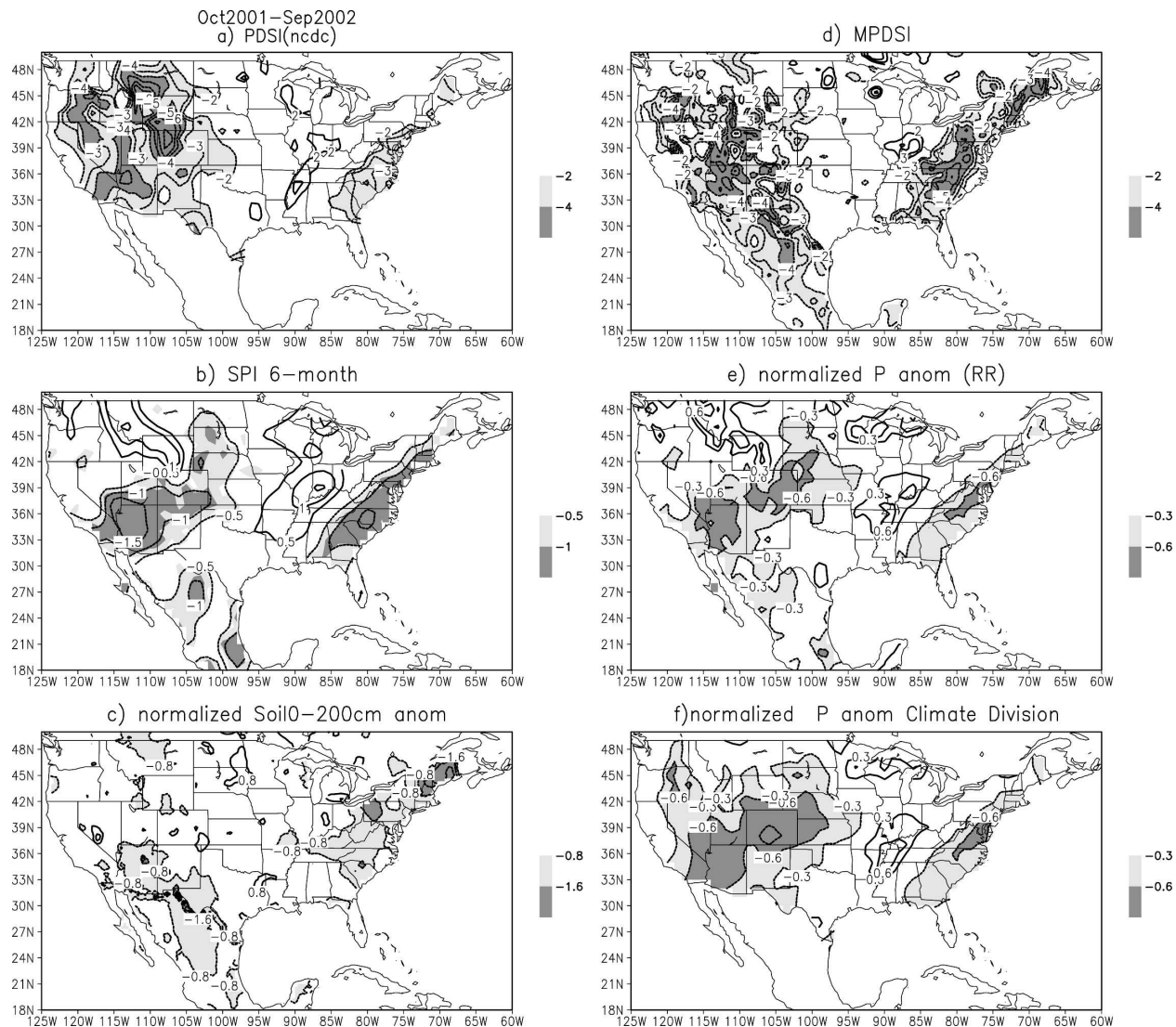
FIG. 8. Same as Fig. 7, but from October 2001 to September 2002.
