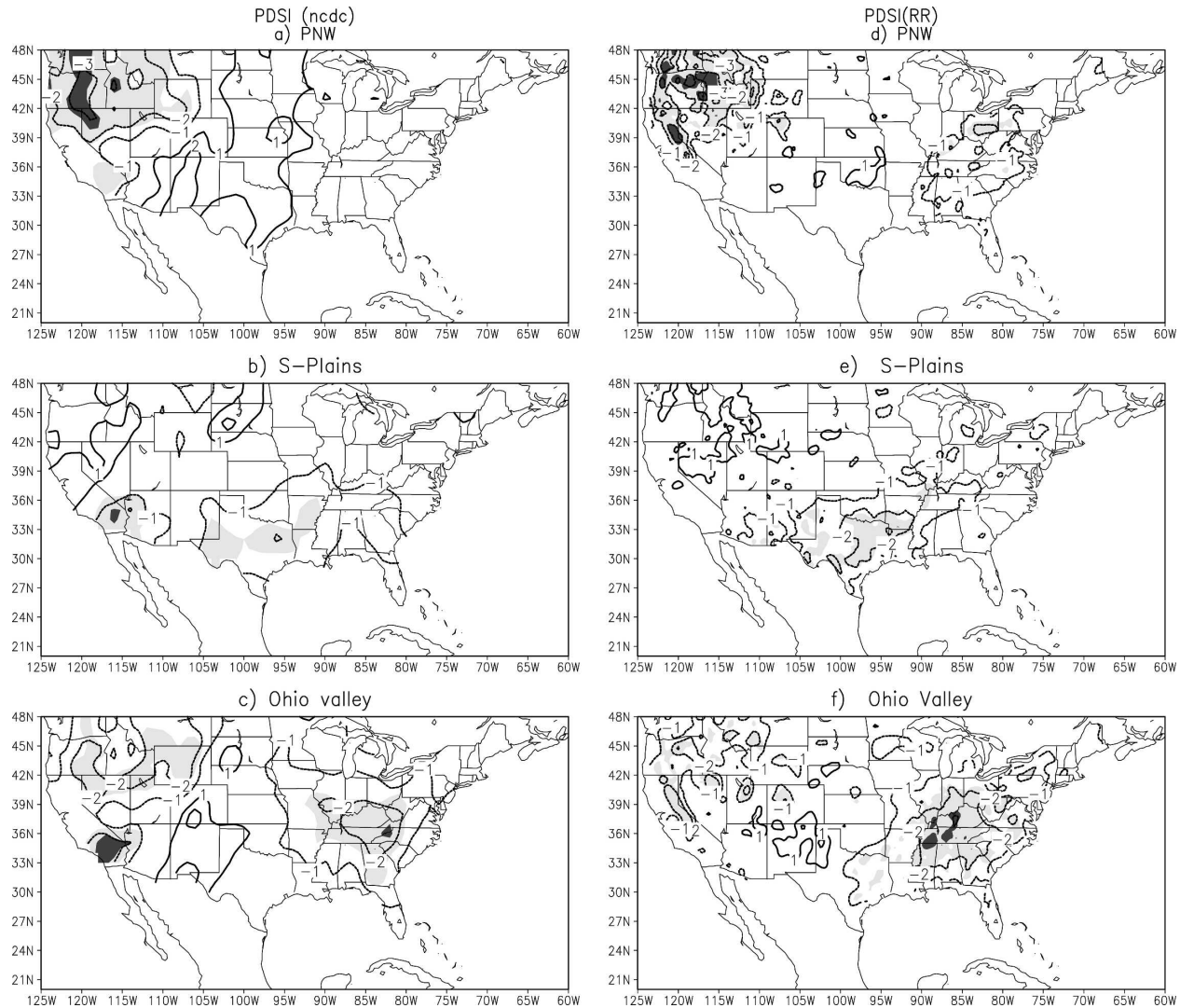
FIG. 6. Composite of the PDSI(ncdc) over drought conditions indicated by SPI6 for the (a) PNW, (b) southern plains, and (c) Ohio Valley. Contour interval is 1, with the zero contour omitted. Light (dark) shading indicates that there are more than 50% (70%) of the cases in the composite for which both the PDSI(ncdc) and the SPI6 indicate drought. (d)–(f) Same as (a)–(c), but for the MPDSI.
