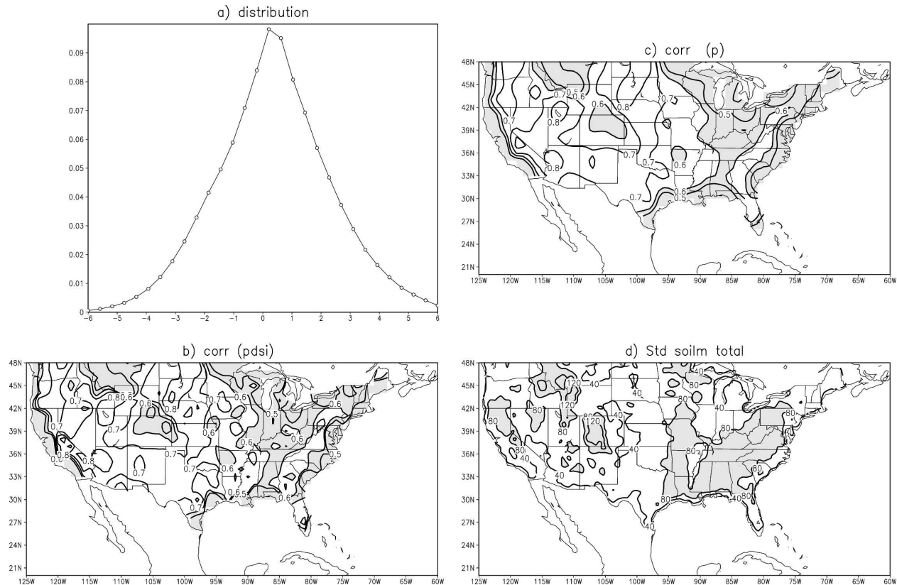
FIG. 4. (a) Distribution function of the MPDSI with all data pooled together. (b) Correlation between the MPDSI and PDSI(ncdc) for the period of 1979–2004. Contour interval is 0.1. Values less than 0.6 are shaded. (c) Same as (b), but for the correlation between P from the RR and P from the climate divisions. (d) Standard deviation of the total soil moisture. Contour interval is 40 mm. Values greater than 80 mm are shaded.
