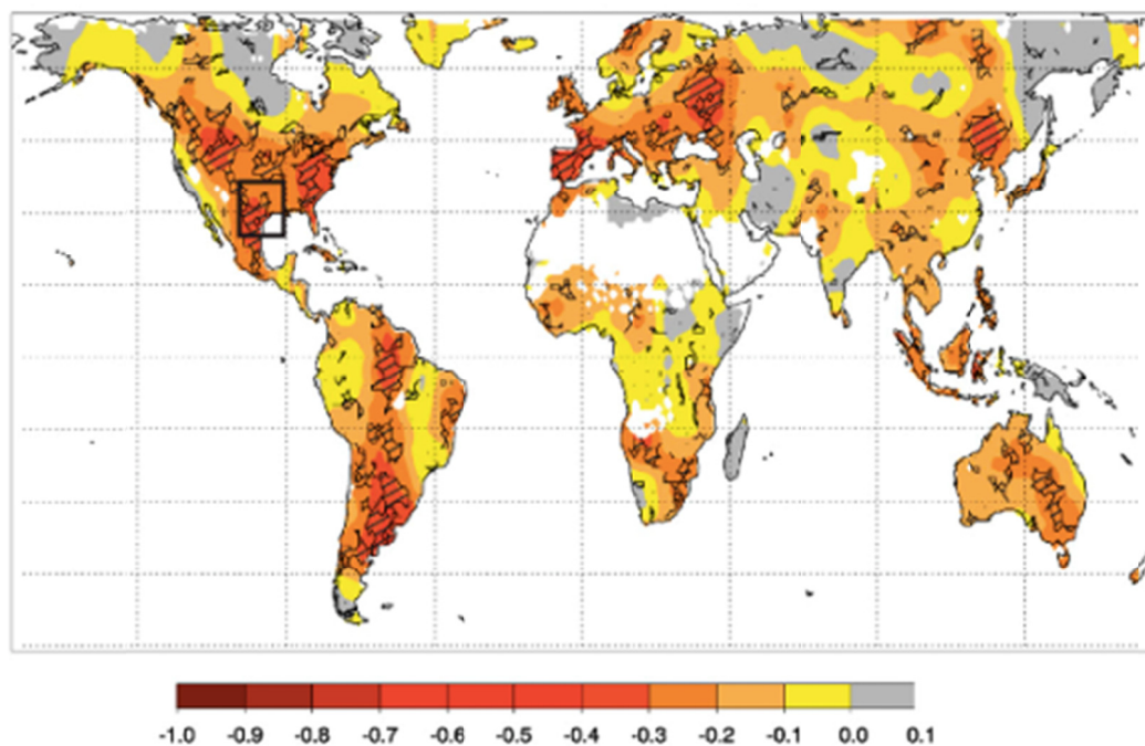
FIGURE 4.6 Correlation between number of hot days in the hottest month of each year and preceding three months precipitation deficits. Red areas indicate where dry periods from preceding three months correspond with more hot days. SOURCE: Mueller and Seneviratne, 2012.
