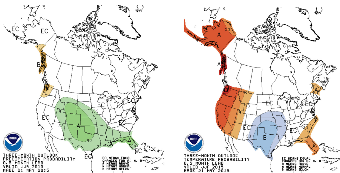
FIGURE 3.2 Three-month outlooks issued by the NOAA Climate Prediction Center for June-July-August 2015, issued 21 May 2015 (0.5 month lead time). Contours indicate probability of above (A) or below (B) normal precipitation (left) and temperature (right). EC indicates equal chances, where probability is evenly distributed across the three categories (above, normal, or below). SOURCE: NOAA.
