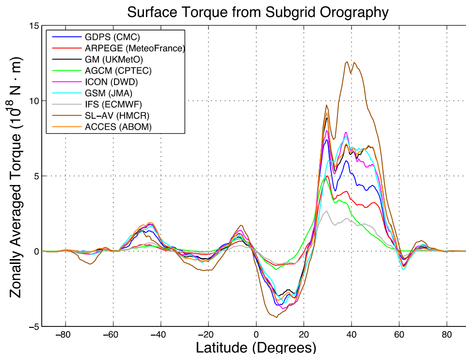
FIGURE 5.10 Zonally averaged subgrid orographic torque from a number of global NWP models for January 2012. SOURCE: Ayrton Zadra.
