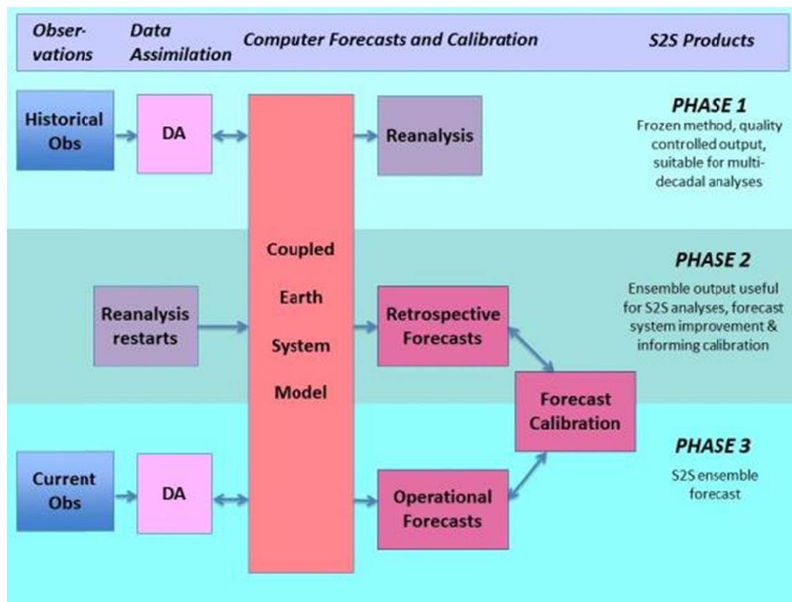
FIGURE 5.1 The production of calibrated subseasonal and seasonal forecasts involves three separate processes. In the first phase, historical observations over a period of two or more decades are combined with data assimilation (DA) and Earth system dynamics in a coupled Earth system computer model (coupled ESM) to produce a reanalysis that is a detailed history of a wide variety of atmospheric, oceanic, land, and cryospheric variables. In the second phase, the reanalysis data is used as the initial conditions for a set of retrospective ESM S2S forecasts over the same two decades or more. The comparison of the retrospective forecasts with an appropriate set of verification data (perhaps the reanalysis) is then used to develop quantitative information for correcting biases and ensemble variance of the forecasts to be applied subsequently to operational forecasts. In the third phase, the current observations processed with data assimilation (which may be equivalent to the latest reanalysis if the forecast system is unchanged since the last reanalysis was run) serve as the initial conditions for a set of operational forecasts that are then calibrated in the S2S probability prediction system and turned into S2S forecast products. Dutton et al. (2013) describe the operation and results of this process, as implemented in a commercial S2S system.
