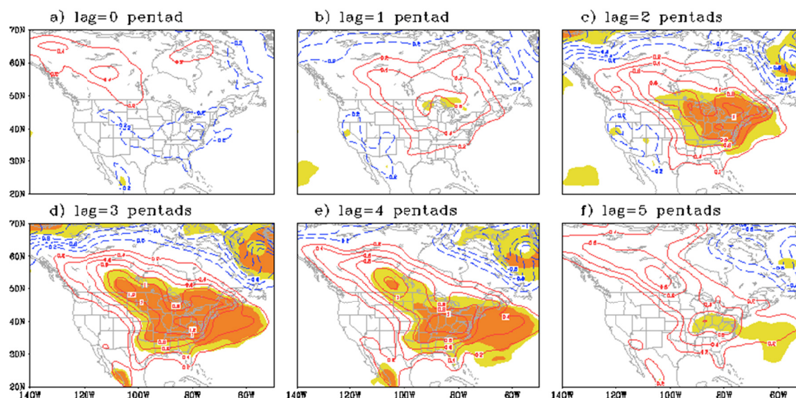
FIGURE 4.5 Lagged regressions of surface air temperature (SAT) in the North American region onto -RMM2 . Lag n means that the SAT anomaly lags -RMM2 by n pentads (5-days). The sign of RMM2 is reversed so that it represents enhanced convection in the Indian Ocean and corresponds to MJO phases 2-3. The magnitude corresponds to one standard deviation of the RMM2 . Yellow (orange) areas represent those where the regression is statistically significant at a 0.05 (0.01) level according to a Student-t test. Contour interval is 0.2^{\circ}K . The zero contour is not plotted, and contours with positive and negative values are in solid red and dashed blue, respectively. RMM2 is the second component of RMM , which corresponds to anomalous convection activity in the tropical Indian Ocean. SOURCE: Figure courtesy of Hai Lin.
