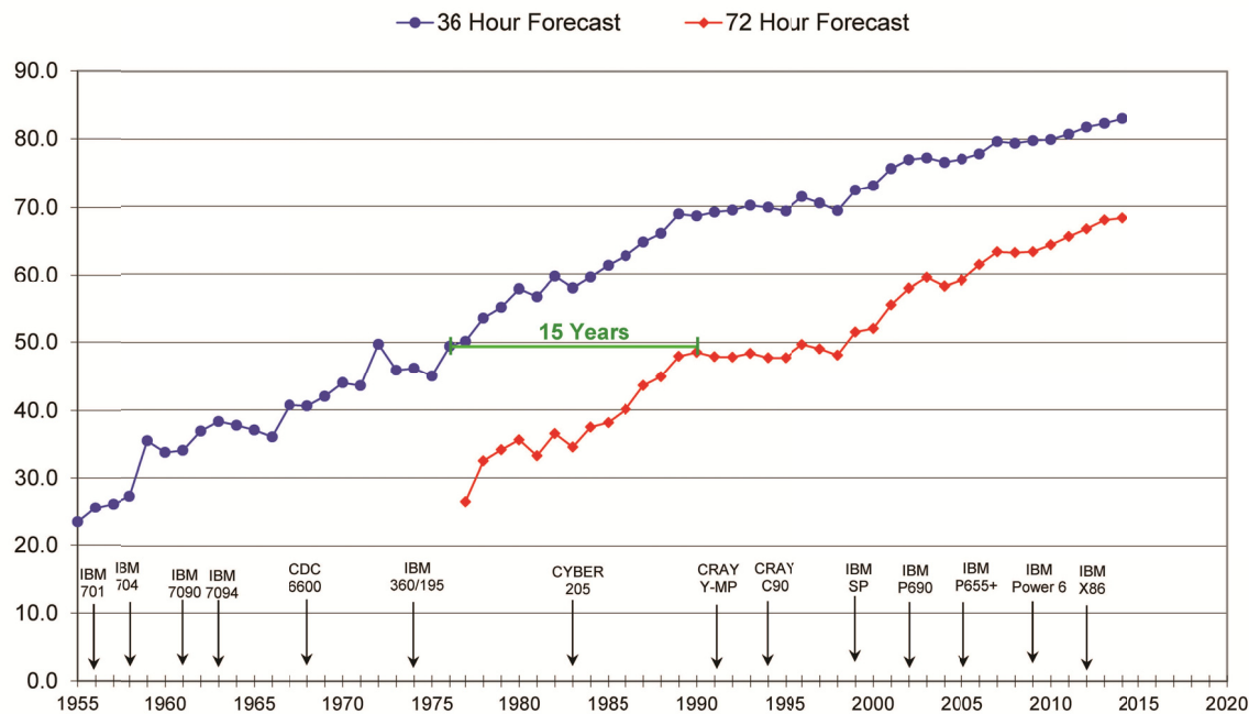
FIGURE 2.1 Forecast verification for 36 and 72-hour forecasts for the Global Forecast System (GFS) model. The skill ( S1 ) is based on the mean error of the 500 mb heights in the forecasts relative to radiosonde measurements over North America. This quantity is shown as 100*(1-S1/70) . A perfect forecast is 100. Dates of computer hardware upgrades are shown with arrows along the x-axis. SOURCE: National Center for Environmental Prediction, http://www.nco.ncep.noaa.gov/sib/verification/s1_scores/s1_scores.pdf , accessed July 20, 2015.
