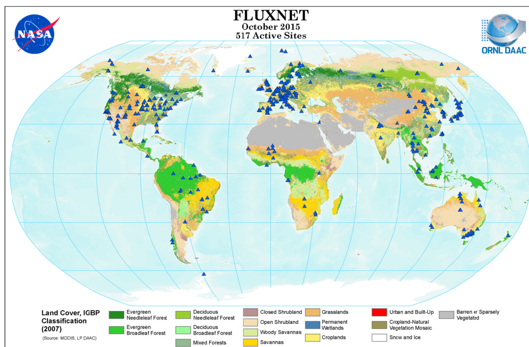
FIGURE 5.5 Distribution of 517 active flux tower sites within global Fluxnet network, as of October 2015. These towers measure exchanges of carbon dioxide, water vapor, and energy between the atmosphere and terrestrial ecosystem. SOURCE: Oak Ridge National Laboratory Distributed Active Archive Center (ORNL DAAC). 2013. FLUXNET Maps & Graphics Web Page. Available online [ http://fluxnet.ornl.gov/maps-graphics ] from ORNL DAAC, Oak Ridge, Tennessee, USA, accessed February 22, 2016
