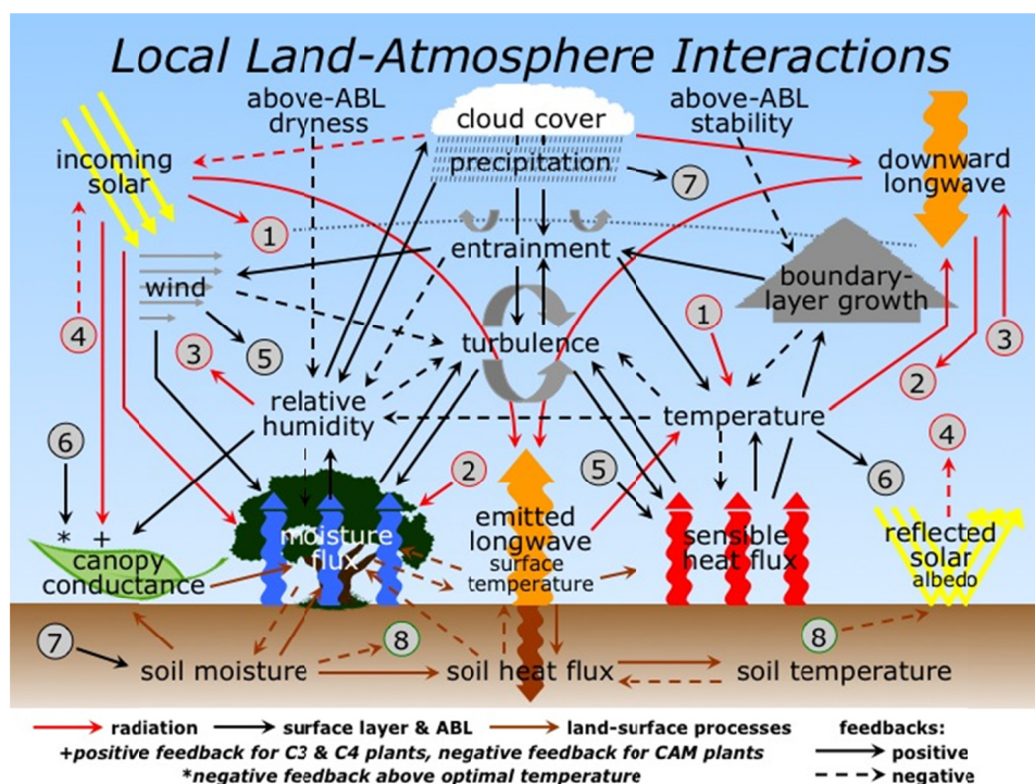
FIGURE 5.12 , Schematic showing the many interactive processes in the land surface and atmospheric boundary layer (ABL). SOURCE: Mike Ek, adapted from Ek and Holtslag (2004).
