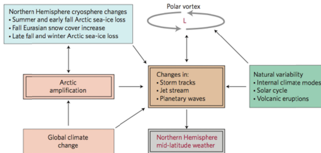
FIGURE 4.8: Schematic of ways to influence Northern Hemisphere mid-latitude weather. Three major dynamical features for changing Northern Hemisphere mid-latitude weather—changes in the storm tracks, the position and structure of the jet stream, and planetary wave activity—can be altered in several ways. Arctic amplification directly (by changing the meridional temperature gradient) and/or indirectly (through feedbacks with changes in the cryosphere) alters tropospheric wave activity and the jet stream in the mid- and high latitudes. Two other causes of changes in the storm tracks, jet stream and wave activity that do not involve Arctic amplification, are also presented: (1) natural modes of variability and (2) the direct influence of global climate change (that is, including influences outside the Arctic) on the general circulation. The last two causes together present the current null hypothesis in the state of the science against which the influence of Arctic amplification on mid-latitude weather is tested in both observational and modelling studies. Bidirectional arrows in the figure denote feedbacks (positive or negative) between adjacent elements. Stratospheric polar vortex is represented by ‘L’ with anticlockwise flow. SOURCE: Figure and caption from Cohen et al., 2014.
