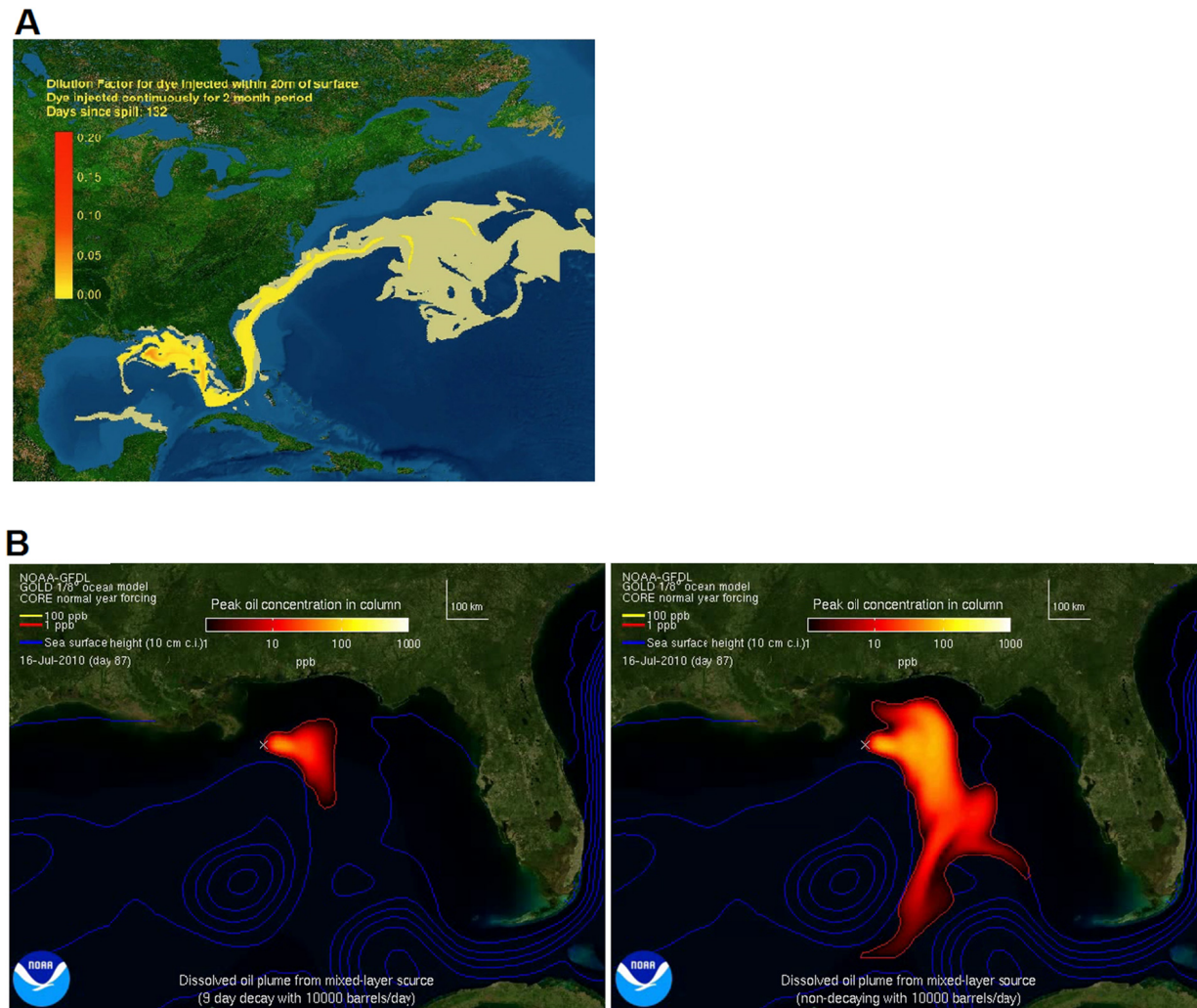
FIGURE 3.6 (A) A frame from a June 3, 2010 animation depicting the dilution and transport after 132 days of a dye released at the location of the Deepwater Horizon oil spill. This animation was widely shown on national television (Maltrud et al., 2010). SOURCE: https://www2.ucar.edu/atmosnews/news/2154/ocean-currents-likely-carry-oil-along-atlantic-coast , accessed January 27, 2016. (B) A frame from a NOAA animation of dissolved oil concentrations that include (left) or omit (right) the biological consumption of oil and only contour the oil concentrations that exceed EPA limits in drinking water to avoid creating misleading interpretations (Adcroft et al., 2010). Although this animation was available in June, 2010, while the DWH was near its peak flow, NOAA only released it publicly after the paper describing it had gone through peer review and been accepted for publication in early August, 2010, two weeks after the well had already been capped off. SOURCE: NOAA.
