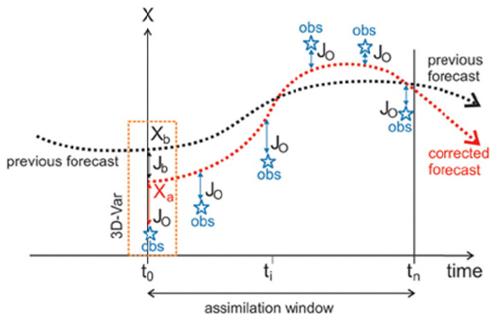
FIGURE 5.7 Schematic diagram illustrating 4D-Var data assimilation. Over the period of the assimilation window, 4D-Var is performed to assimilate the most recent observations (obs, marked as blue stars), using a segment of the previous forecast as the background (black dotted line—the background state, X_b ). This updates the initial model trajectory for the subsequent forecast (red dotted line), using the analysis X_a as the initial condition. The yellow dotted box to the left identifies the special case of 3D-Var. J_o represents the misfit of the observations to the analysis trajectory and J_b represents the misfit between the analysis and original background at the initial time t_0 . SOURCE: Figure and caption adapted from Lahoz and Schneider (2014).
