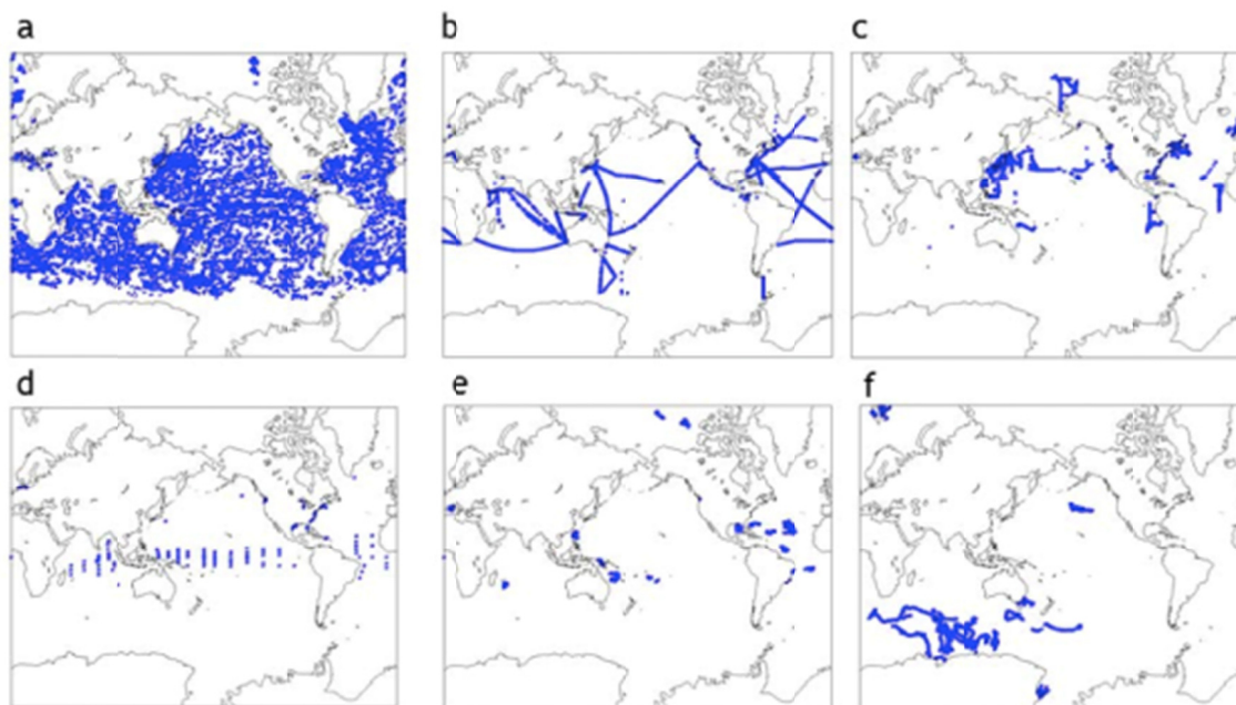
FIGURE 5.4 Ocean data coverage for September through November in 2012 from (a) Argo floats, (b) Expendable Bathythermographs (XBTs), (c) sondes (CTDs) and ocean gliders, (d) fixed buoys, (e) drifting buoys, (f) animal borne sensors. SOURCE: Fairall et al., 2013.
