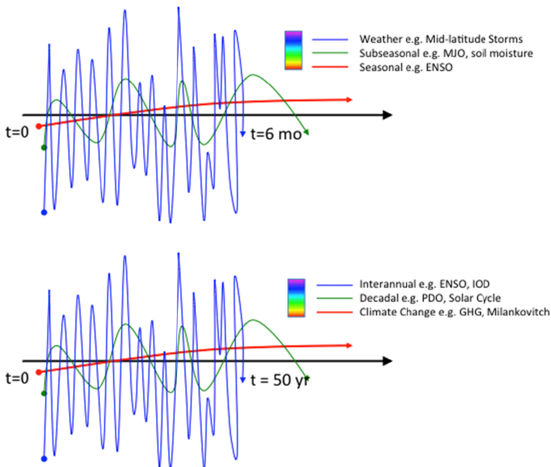
FIGURE 4.1 Schematic illustration of time series depicting variations in an arbitrary quantity relevant to weather/climate with variations typical of (top) weather (blue), subseasonal variability (green) and seasonal variability (red) over a 6 month period starting from t=0 . The bottom panel is similar to the top, but for interannual, decadal, and longer-term century scale variations. The line colors and spectrum of colors from which they are drawn are meant to illustrate that there are a continuum of phenomena/processes across these indicated timescales (i.e., frequencies) with notable peaks in the spectrum highlighting a subset of the continuum that typically are found to be sources of predictability.
