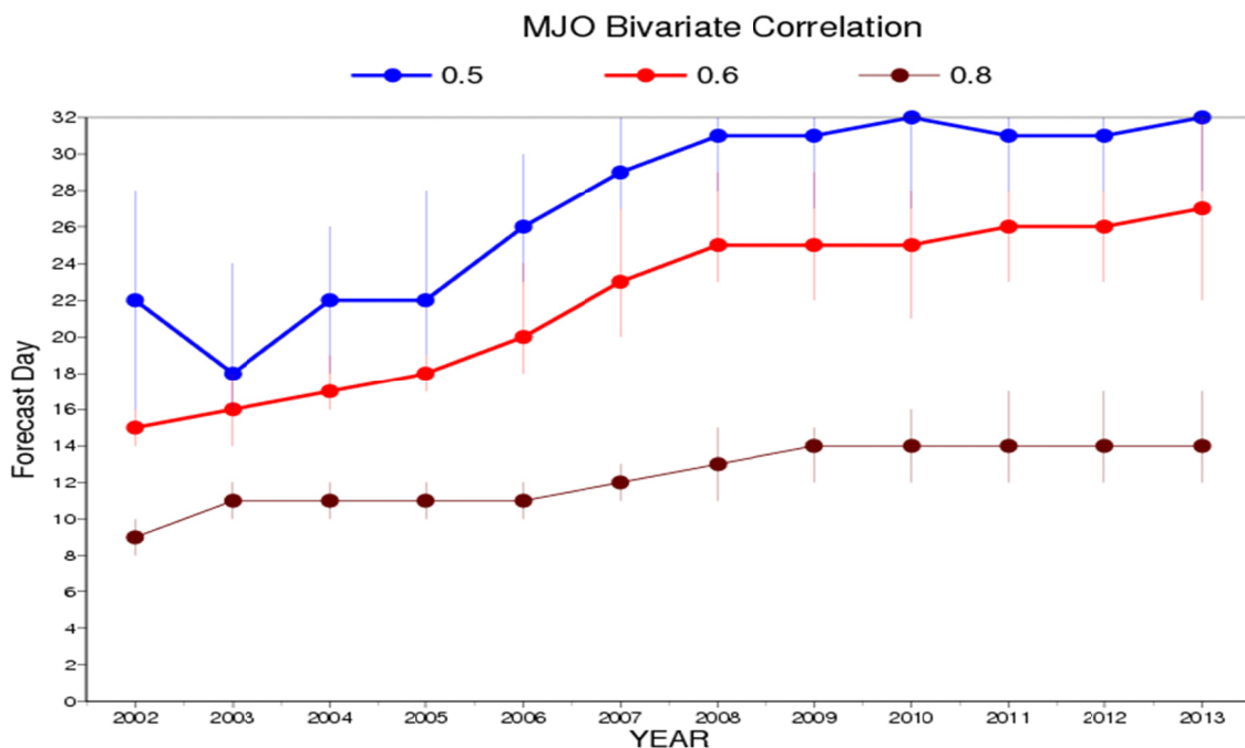
FIGURE 2.3 Evolution of the MJO skill scores since 2002, calculated as bivariate correlations applied to the Real-time Multivariate MJO (RMM) index of Wheeler and Hendon (2004). The MJO skill scores are computed on the ensemble mean of the ECMWF retrospective forecasts produced during a complete year. The blue, red, and brown lines indicate respectively the day when the MJO bivariate correlation skill drops to 0.5, 0.6, and 0.8. SOURCE: Modified from Vitart, 2014.
