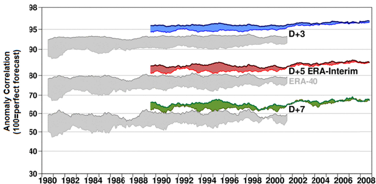
FIGURE 5.6 ECMWF 500-hPa geopotential height anomaly correlations from two different reanalysis systems. Gray: ERA-40 (Uppala et al., 2005) with 3D-Var (ca. 1998); Colors: ERA-Interim (Dee et al., 2011) which uses 4D-Var (ca. 2005). “D+3” corresponds to the 3-day forecast; “D+5” the 5-day forecast; and, “D+7” the 7-day forecast. In each case the top line is the anomaly correlation of the forecasts started from the reanalysis for the Northern Hemisphere, and the bottom line is the corresponding forecast for the Southern Hemisphere. Note the improvement brought about by the improvement of the data assimilation system, which is especially important in the Southern Hemisphere. SOURCE: NRC, 2010b and ECMWF.
