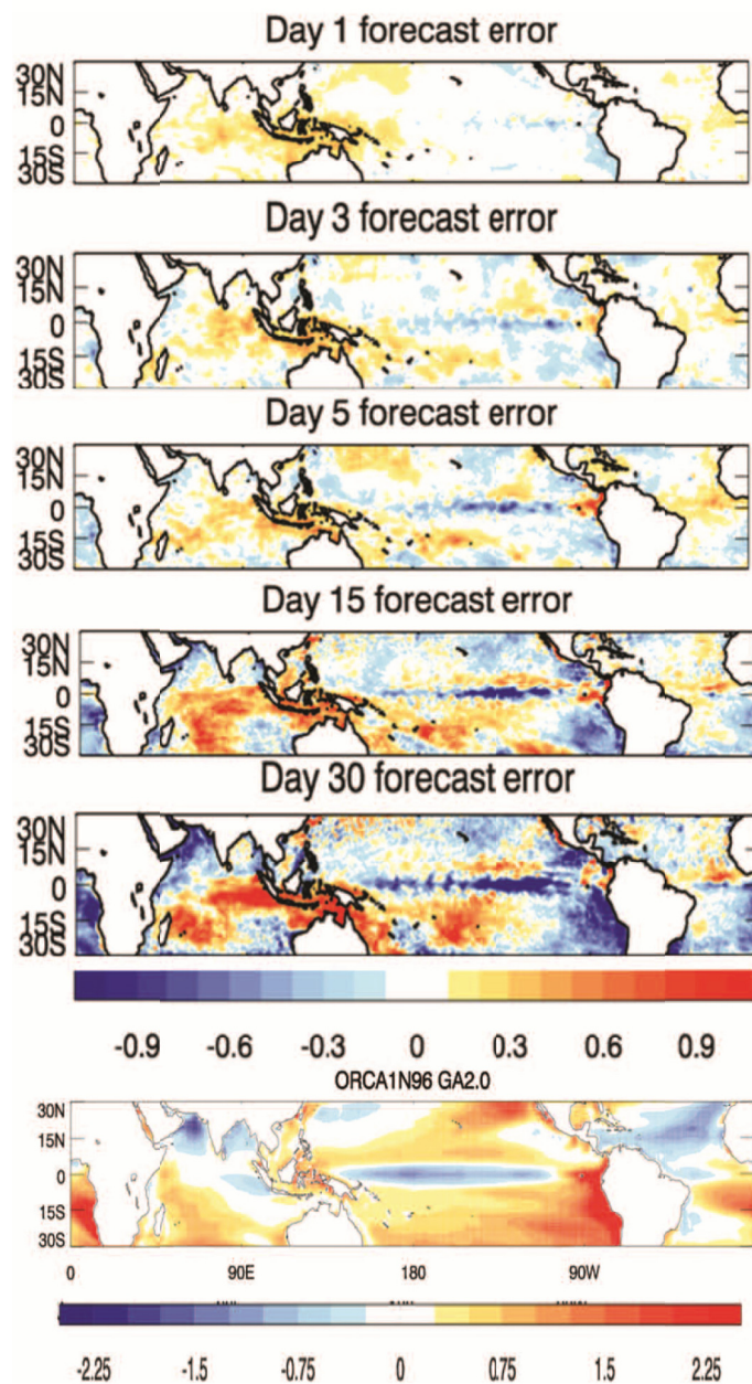
FIGURE 5.9 The drift in coupled model SST as a function of forecast lead time out to 30 days. The bias in a 20-year run from a version (GA2.0) of HadGEM3-AO climate coupled model is shown in the bottom panel. SOURCE: Brown et al. (2012).
