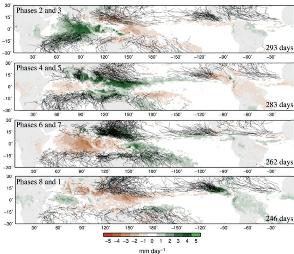
FIGURE 4.10 Composite of tracks of tropical cyclones (1975–2011) and rainfall anomalies (colors) based on Tropical Rainfall Measuring Mission (TRMM) data (1998–2011) for different phases of the MJO represented by the Wheeler and Hendon (2004) Real-time Multi-Variate MJO (RMM) index. Total number of tropical cyclone days in each composite is given at the lower right corners. SOURCE: Zhang, 2013.
