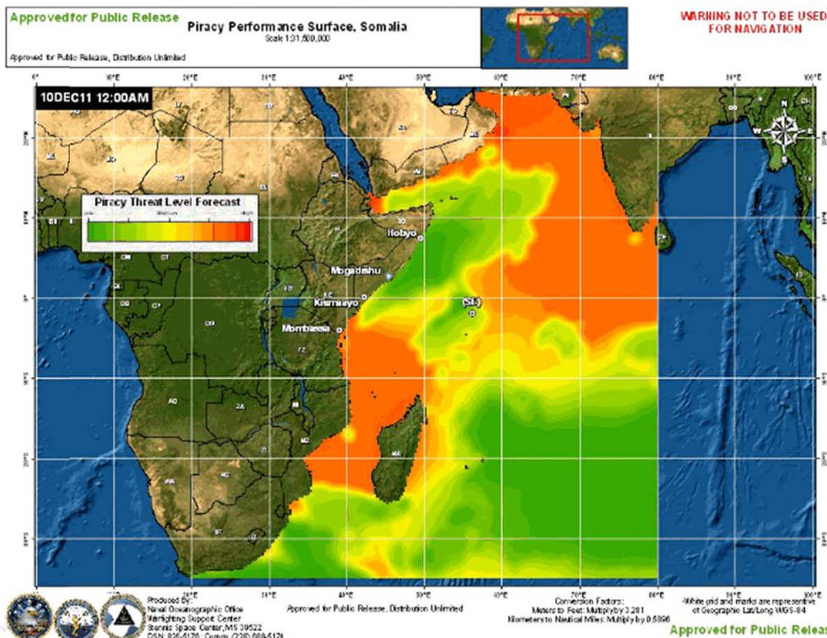
FIGURE 3.5 A piracy threat-level forecast issued by Naval Oceanographic Office, Warfighting Support Center. Real-time parameters—including intelligence information, shipping information, and forecasts of ocean currents, waves, and wind—are combined with historical correlative analysis between environmental conditions and pirate attacks to provide a forecast of pirate threat levels. Warm colors indicate a higher probability of attack. SOURCE: Naval Oceanographic Office, Warfighting Support Center.
