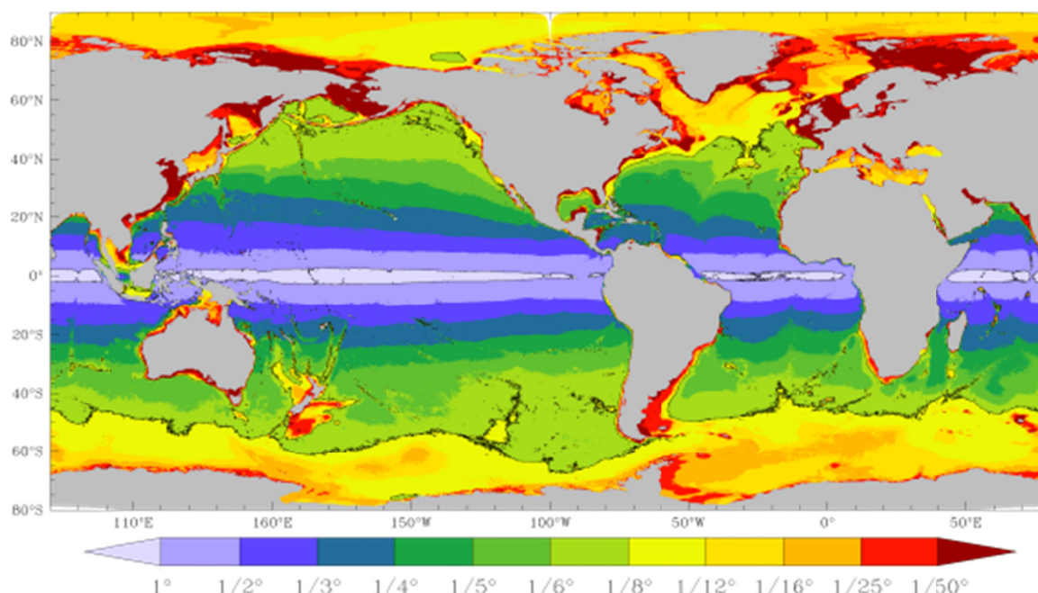
FIGURE 5.11: The horizontal resolution needed to resolve the ocean's first baroclinic deformation radius with two grid points, based on a 1/8^\circ global ocean model on a Mercator grid with a bipolar Arctic cap north of 65^\circ\text{N} . SOURCE: Adapted from Hallberg, 2013.
