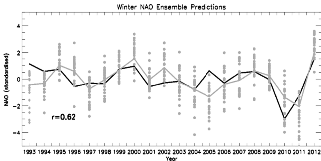
FIGURE 2.2 Predictability of the winter (December–February) NAO in the UKMO seasonal forecast system. Time series of the NAO in observations (black line), ensemble mean forecasts (grey line), and individual ensemble members (grey dots) in winter retrospective forecasts are shown. The correlation score of 0.62 is significant at the 99% level according to a t test and allowing for the small lagged autocorrelation in forecasts and observations. SOURCE: Figure and caption modified from Scaife et al., 2014a.
