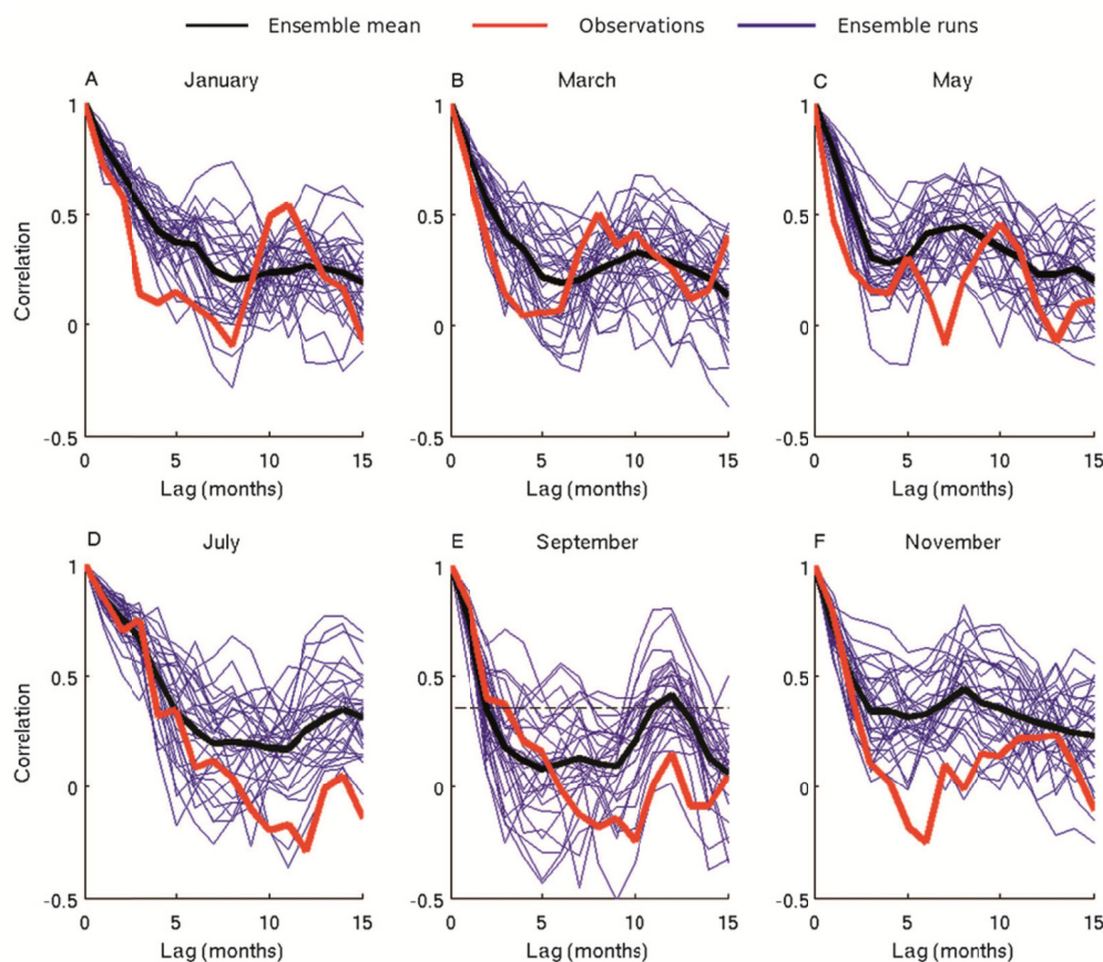
FIGURE 4.7 Monthly lagged correlation of Arctic sea ice area in an ensemble of early 21 st century simulations with the Community System Model Version 3 (blue lines are ensemble members and black lines are ensemble mean) and observations from passive-microwave satellites (red lines). For the first panel, the autocorrelation for January is shown at lag 0, the correlation of January with February is shown at lag 1, and so forth. The figure shows that sea ice extent anomalies initially persist for 2-4 and then, after a period of low correlation, anomalies reemergence at lags of about 6-12 months, depending on the season. The data were detrended by removing the ensemble mean from the model and a linear fit to the observations. SOURCE: Blanchard-Wrigglesworth et al., 2011a.
