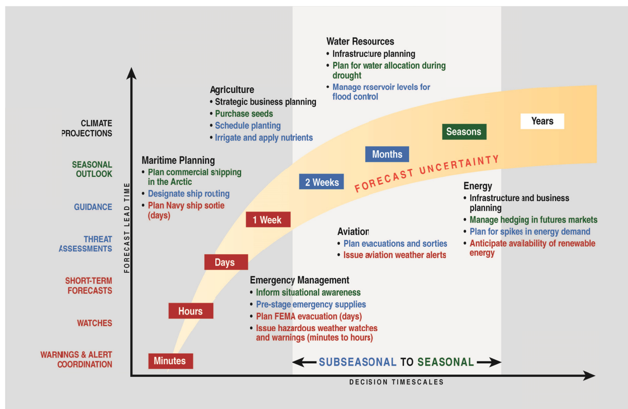
FIGURE 3.1 S2S forecasts (shown in blue and green) fill a gap between short-term weather and ocean forecasts (shown in red) and longer-term Earth system projections (shown in black). They inform critical decisions (also shown in blue and green) across many different sectors by providing information about likely conditions in between these more established prediction times. SOURCE: Modified from the Earth System Prediction Capability Office.
