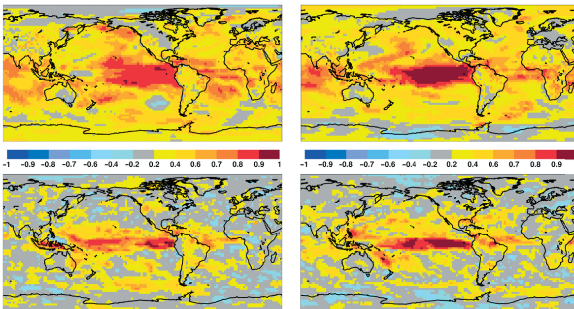
FIGURE 2.4 Correlation of the ensemble mean of one-month lead surface air temperature (top row) and precipitation (bottom row) from the ENSEMBLES multi-model seasonal predictions in boreal summer (June to August, left column) and winter (December to February, right column). The predictions have been performed over the period 1980-2005 with five different forecast systems, each one running nine-member ensembles. The reference data are taken from ERAInterim79 for temperature and GPCP116 for precipitation. SOURCE: Figure and caption from Doblas-Reyes et al., 2013.
