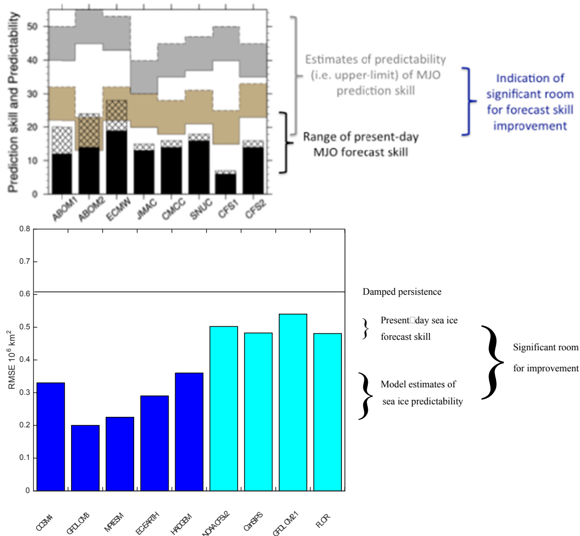
FIGURE 4.2 Prediction skill values versus estimates of predictability—i.e., an estimate of practical present-day skill versus estimates of the potential upper limits of skill—for the MJO (upper) and Arctic September sea ice extent at two-month lead times (lower). For the MJO, predictability is measured in terms of lead time in days. Each bar is based on one of eight ensemble-prediction systems with varying numbers of members depending on the forecast system, or calculated from approximately 20 years of retrospective forecasts. The black bars denote retrospective forecast skill based on single-member forecasts, while the hatched bar shows the improvement based on the ensemble forecast system—i.e., using the ensemble mean of all the forecast system’s members. The tan and gray bars show two different estimates of predictability using the “perfect model” (sometimes called “idealized twin experiment”) approach. For the predictability estimates, one member is designated to represent the “observed” case and another single members (tan bars) or the mean of the remaining members (grey bars) is used to predict it. The sea-ice panel is similar, except error increases with height of the bars, and the dark-blue bars are estimates of predictability and light-blue bars are retrospective forecast skill. SOURCE: Top panel adapted from Neena et al., 2014. Bottom panel based on results in Blanchard-Wrigglesworth (2015).
