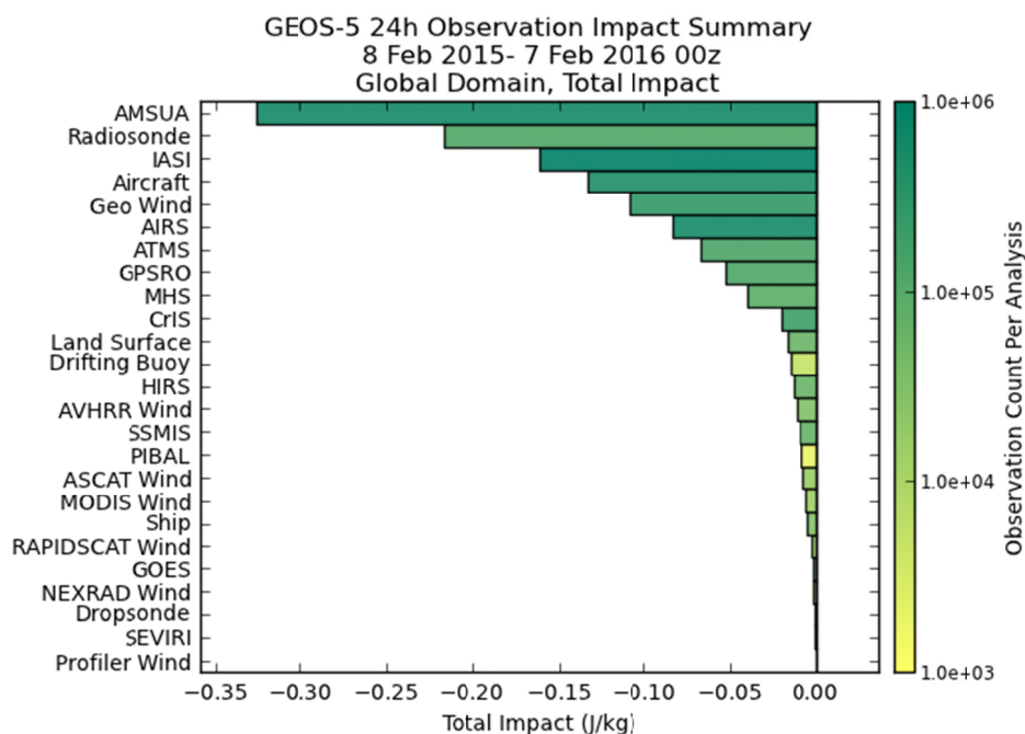
FIGURE 5.3 Adjoint-estimated daily average impacts of various observation types on the 24-h global forecast error (moist total energy, J/kg) calculated for 00 UTC each day for the period covering 08 February 2015 through 07 February 2016 for the NASA GEOS-5 modeling system. The shading corresponds to the average number of observations of each data type that are assimilated into the GEOS-5 system. SOURCE: http://gmao.gsfc.nasa.gov/forecasts/systems/fp/obs_impact , accessed February 15, 2016.
