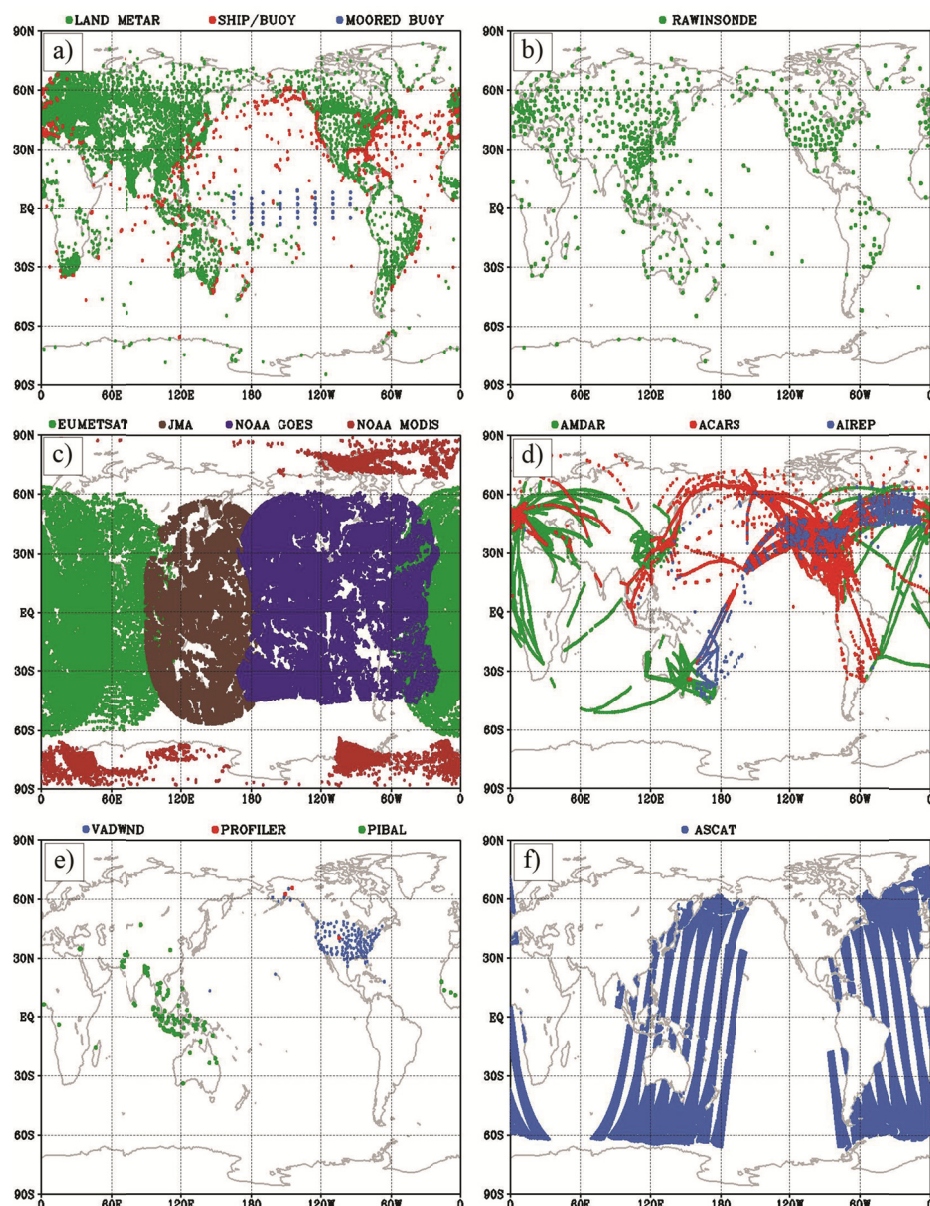
FIGURE 5.2 Spatial distribution for atmospheric observations for the six-hour window centered at 00 UTC 15 April 2015 including (a) surface, (b) rawinsonde, (c) AMVs, (d) aircraft, (e) Velocity Azimuth Display (VAD) winds, lidar wind profilers and pibal balloons, and (f), and Advanced Scatterometer (ASCAT) derived surface wind speeds.
