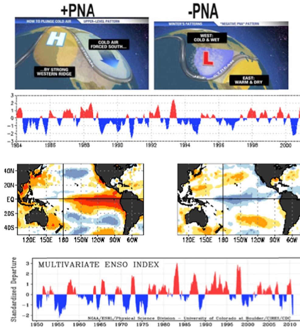
FIGURE 4.4 Two examples of common and impactful “natural modes of variability”. Top panels illustrate the atmospheric circulation anomalies associated with the Pacific North America (PNA) pattern in its positive (left) and negative (right) phases. Bottom panels illustrate the SST anomalies associated with the ENSO phenomenon, showing both El Niño (left) and La Niña (right) phases. SOURCE: From top panel from njweatherblogs.com, other panels from NOAA.
