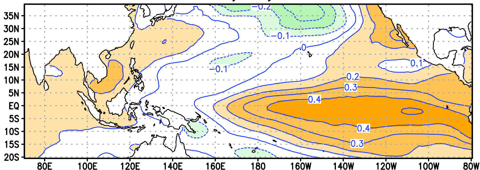
SST anomaly in wet condition
