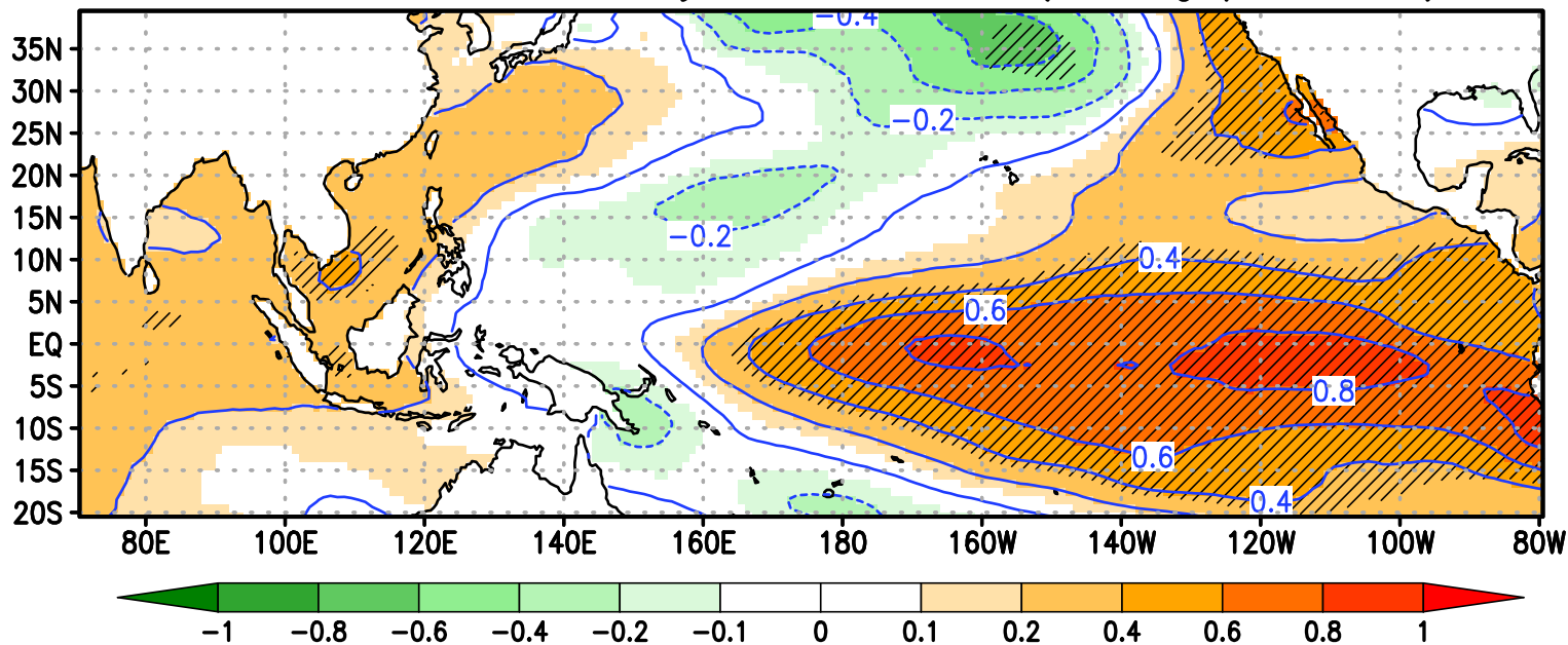
Difference of SST between Dry and Wet condition (Hatching: p -value<5%)
