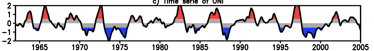
c) Time series of ONI
