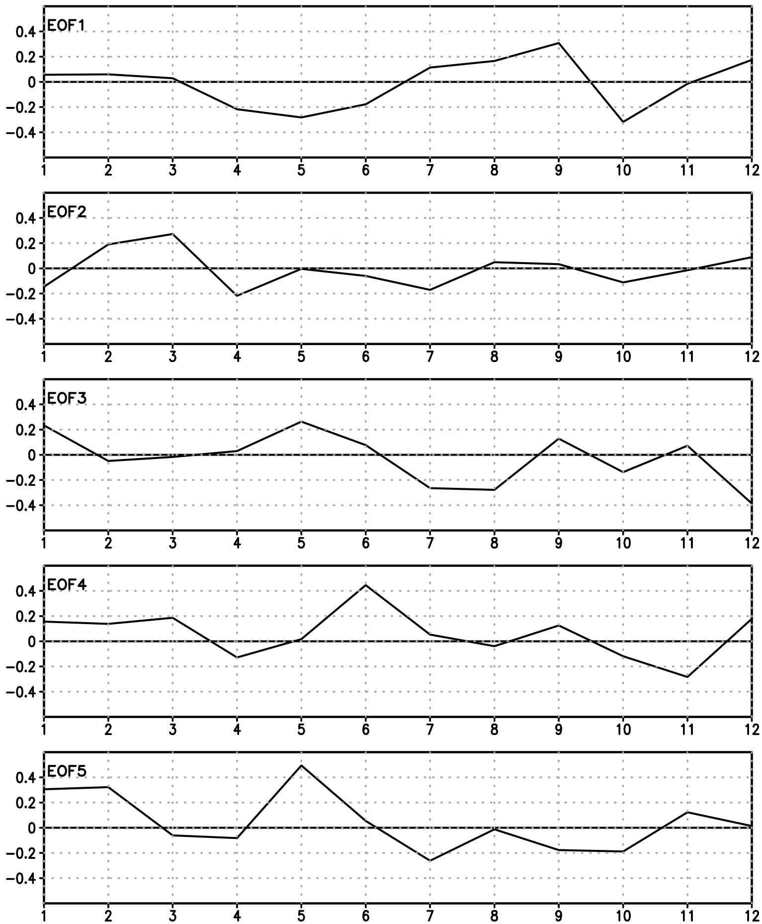
Correlation between TC and EOFs of CFSR prmsl
