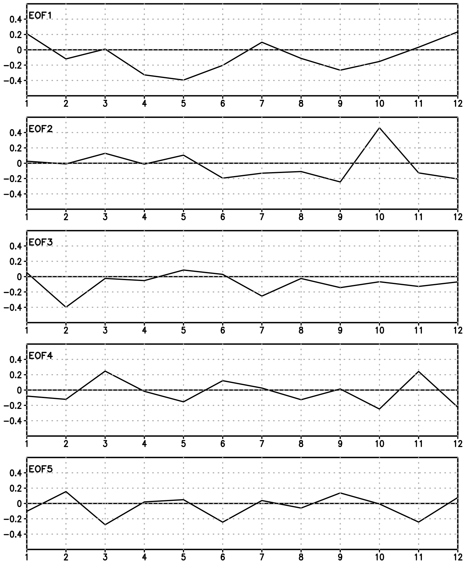
Correlation between TC and EOFs of CFSR sst
