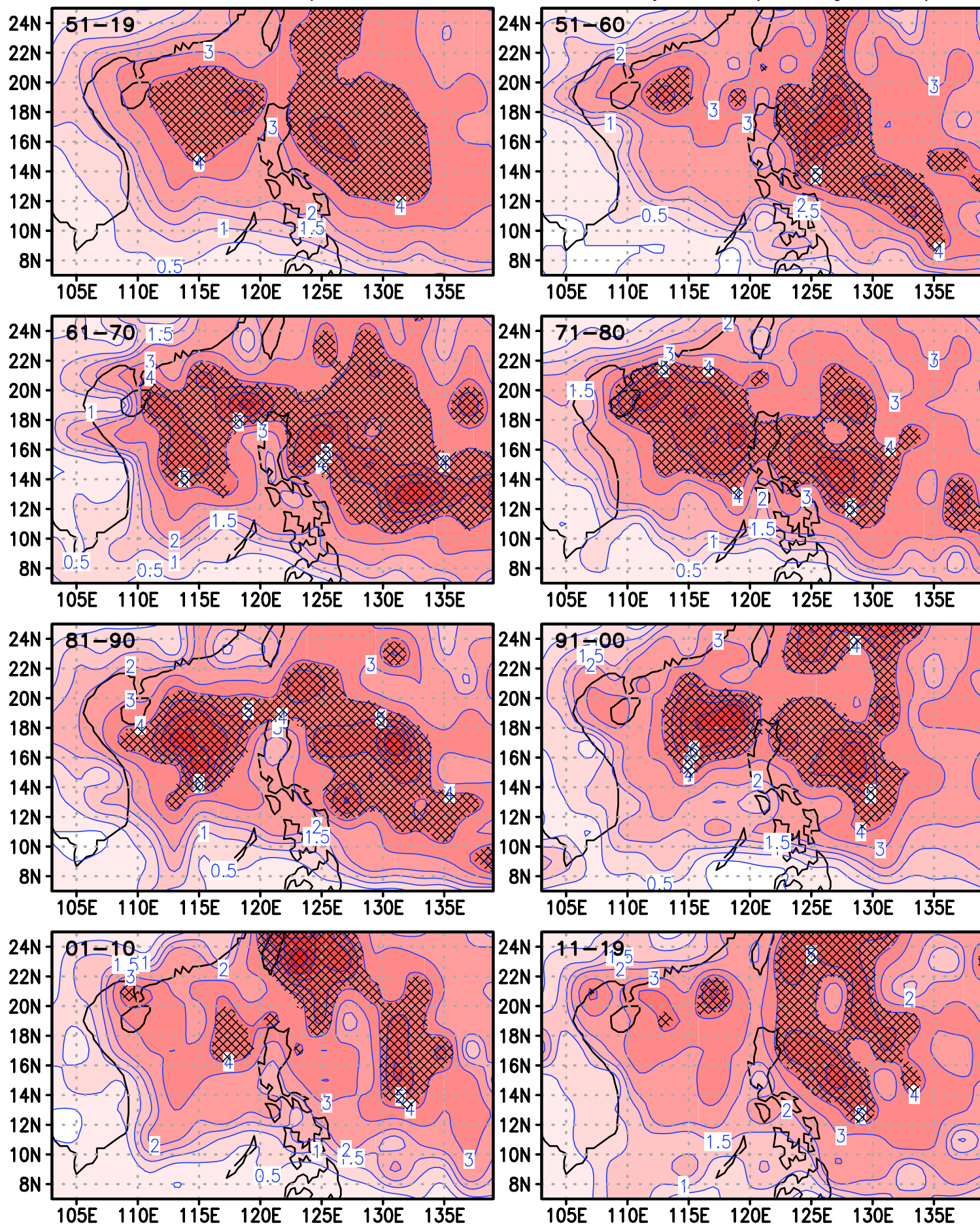
Mean NTC for entire period of 1951–2019 and for every decade (Hatching: TC \geq 4)
