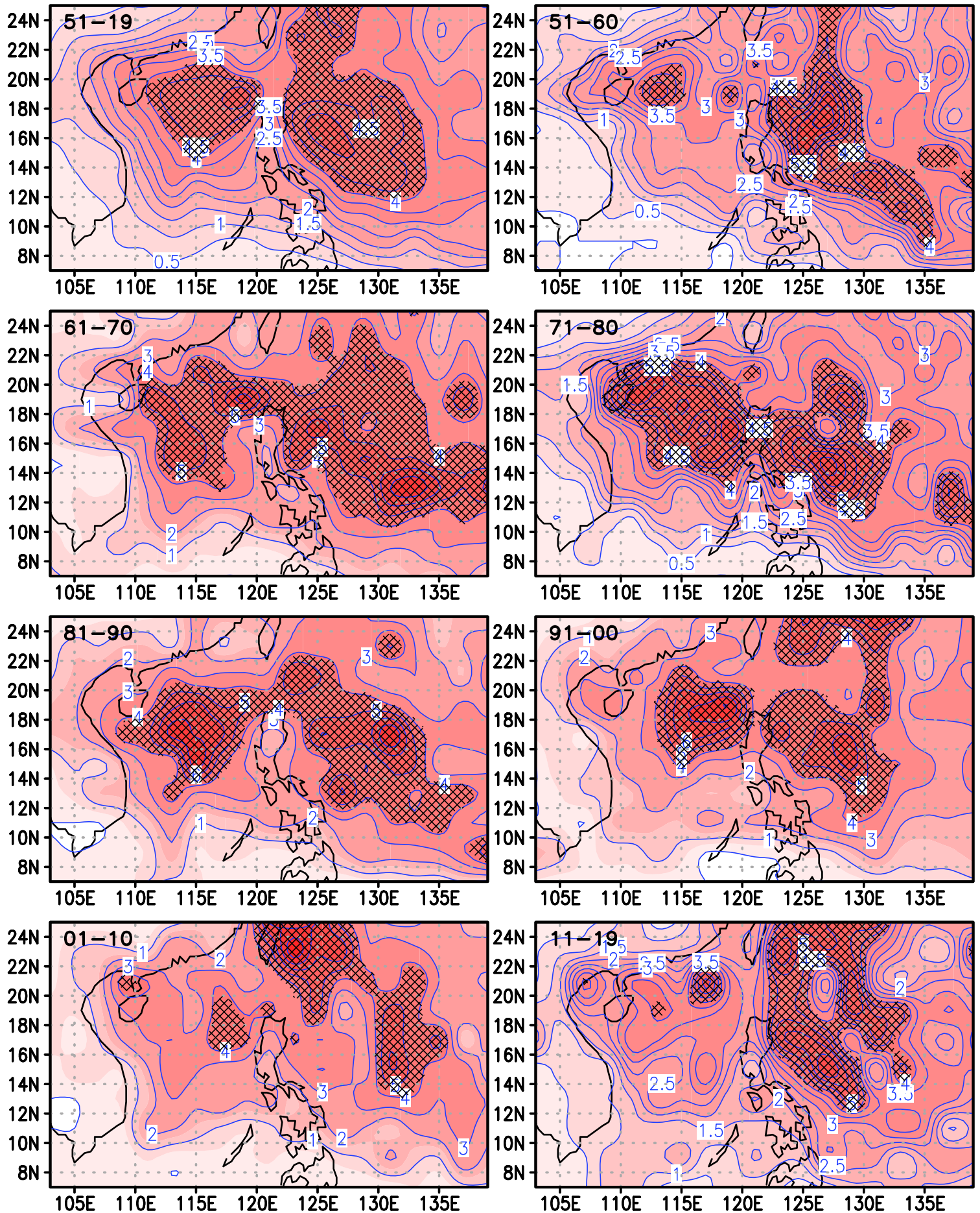
Mean NTC for entire period of 1951–2019 and for every decade (Hatching: NTC \geq 4 )
