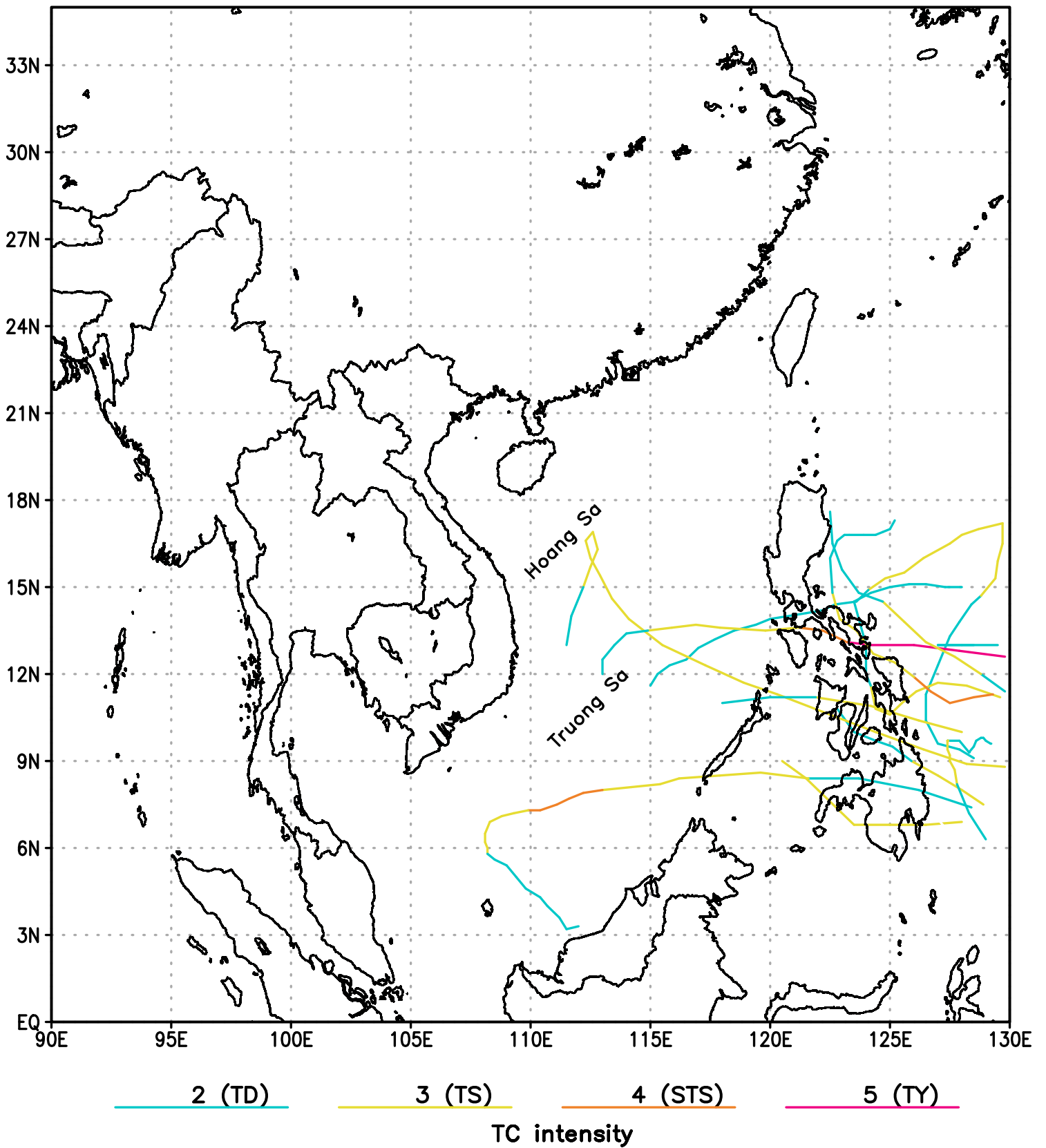
TC tracks of month 1 for period 1951–2019
