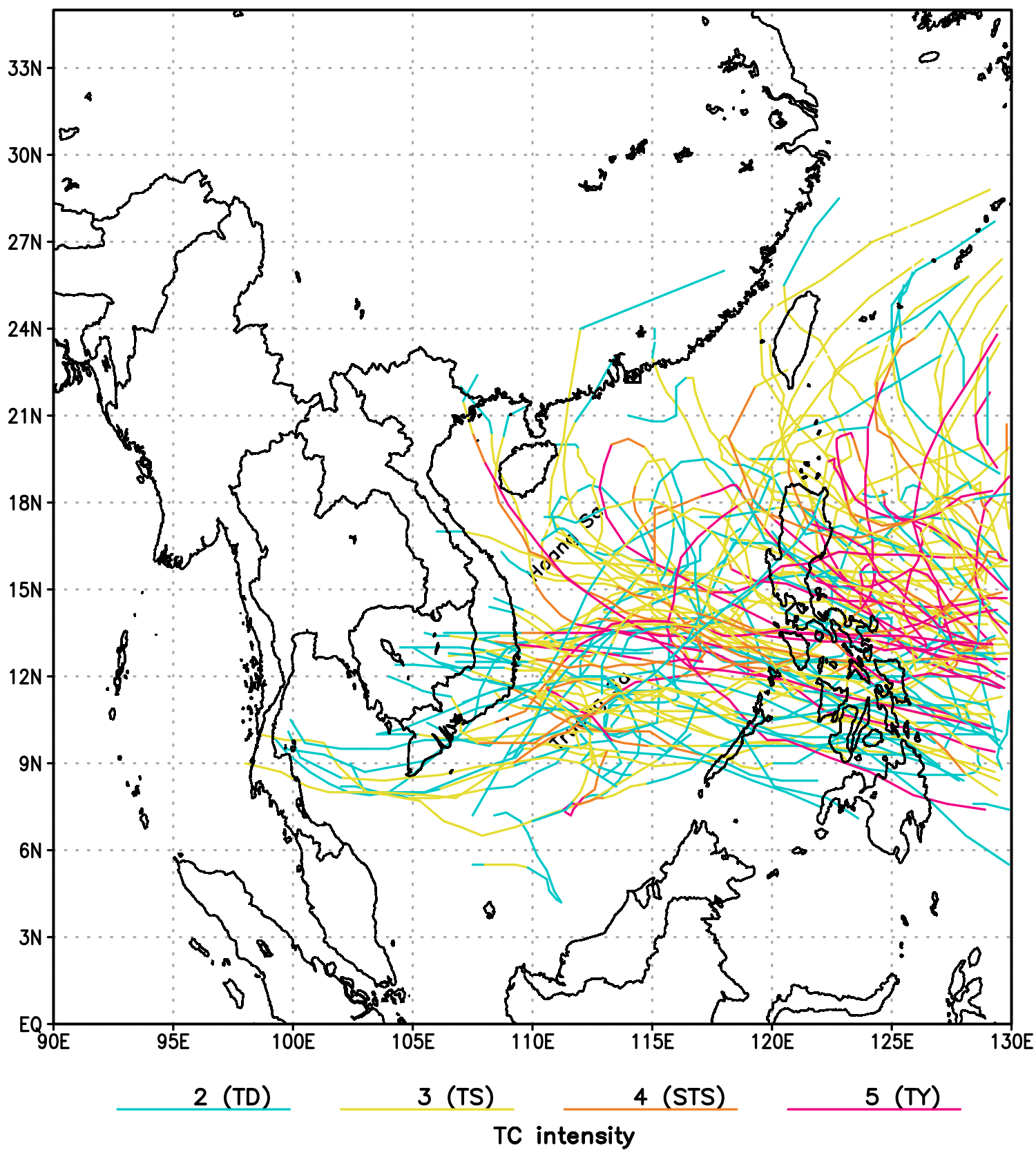
TC tracks of month 11 for period 1951–2019
