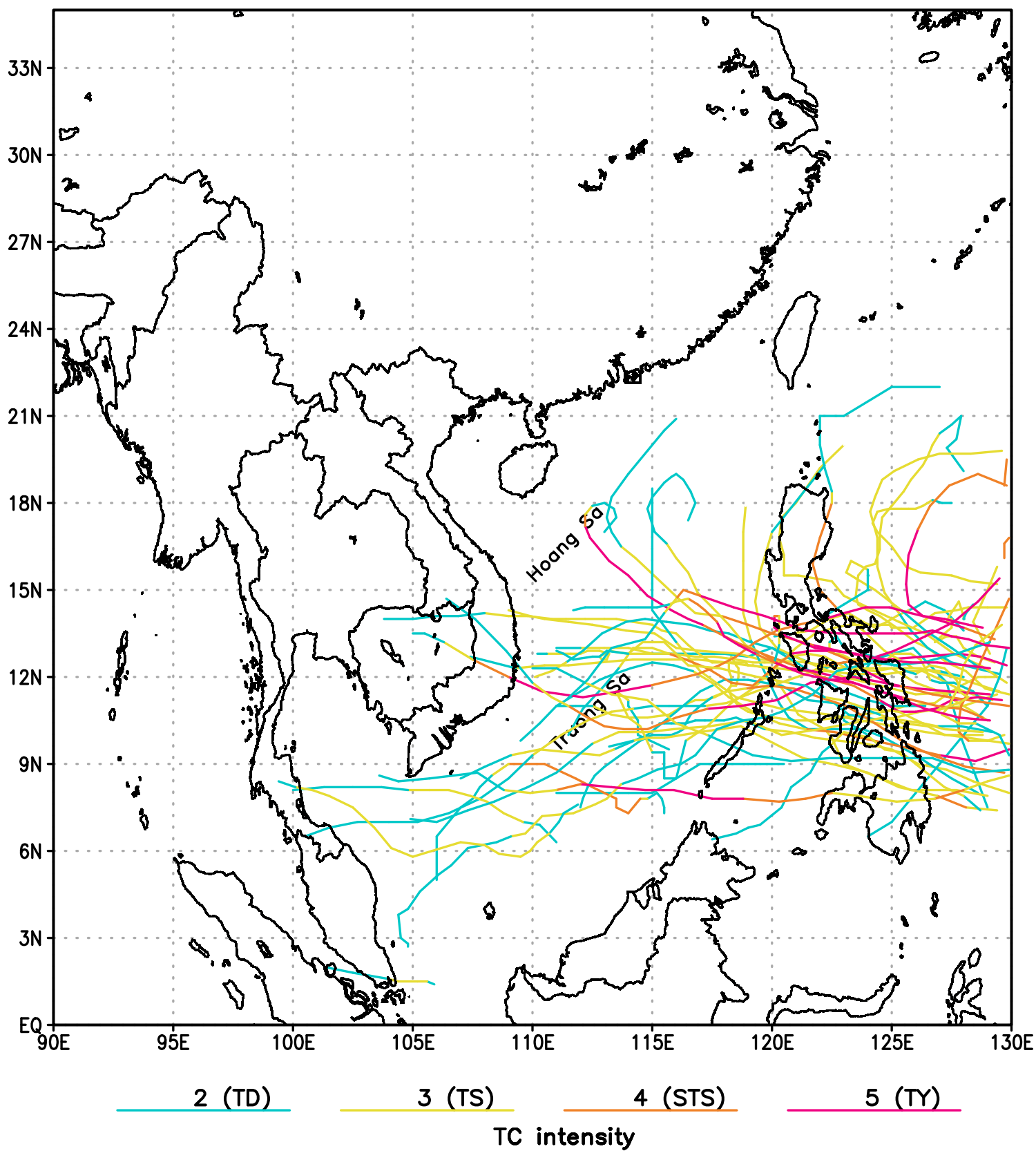
TC tracks of month 12 for period 1951–2019
