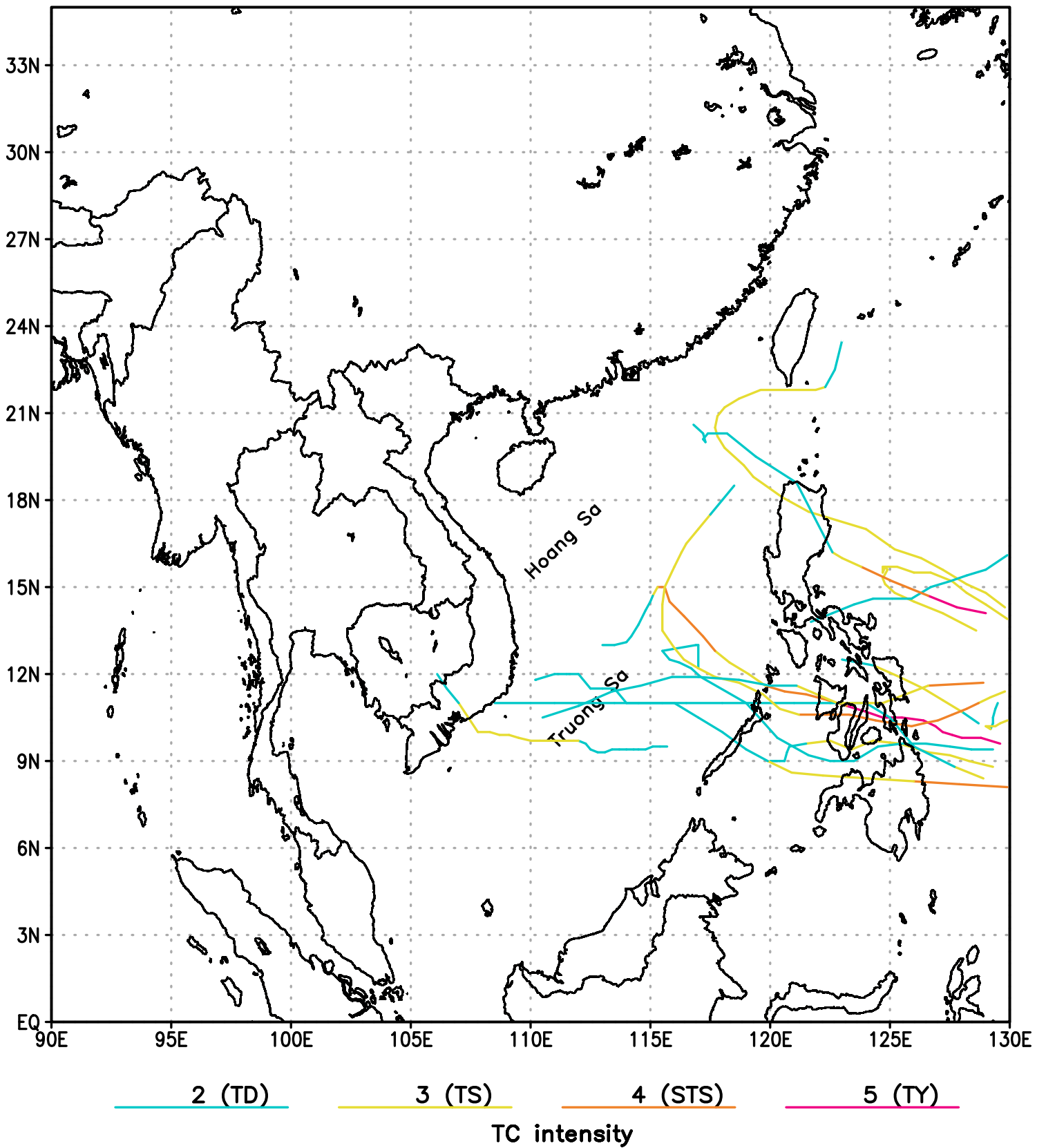
TC tracks of month 3 for period 1951–2019
