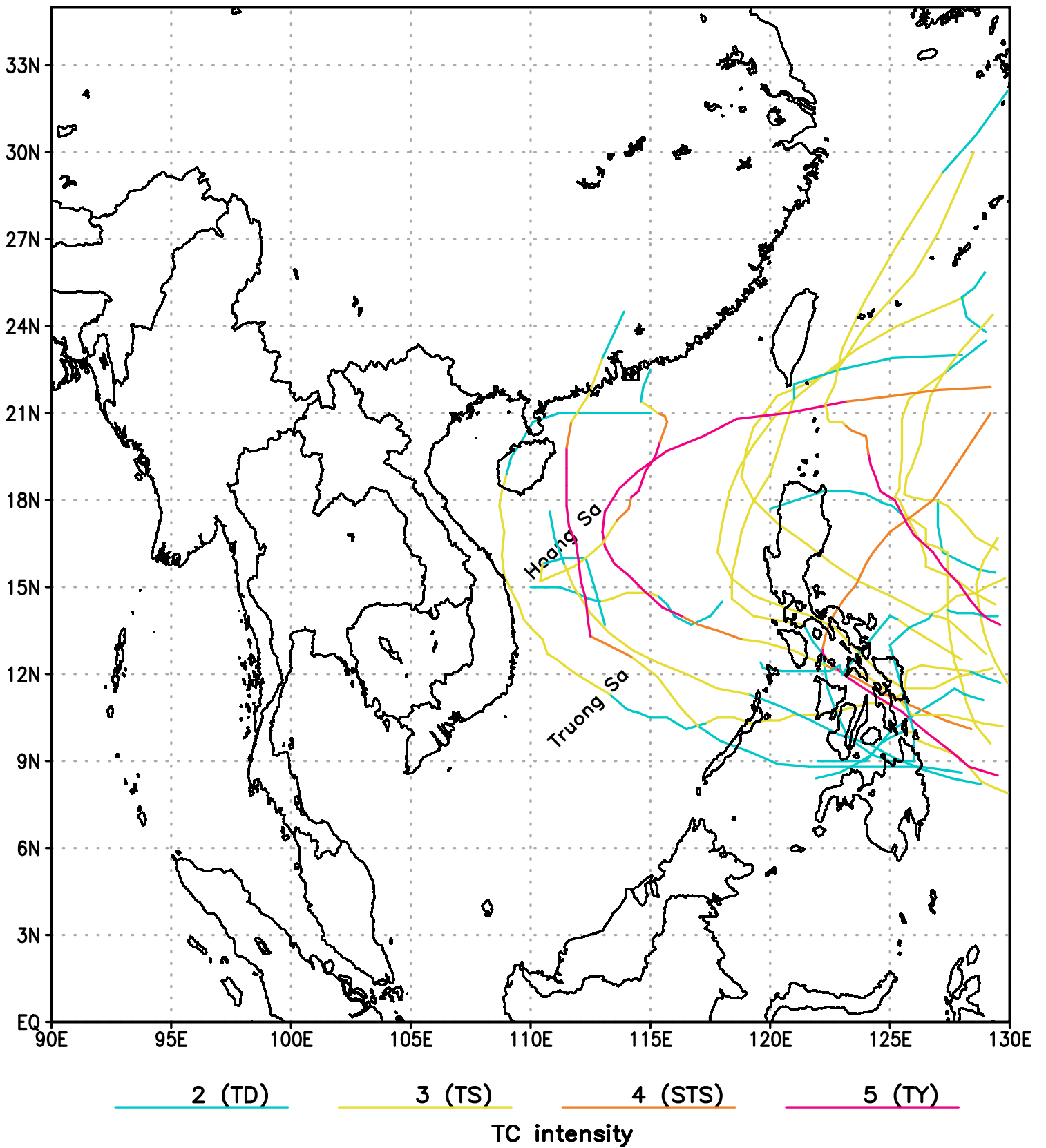
TC tracks of month 4 for period 1951–2019
