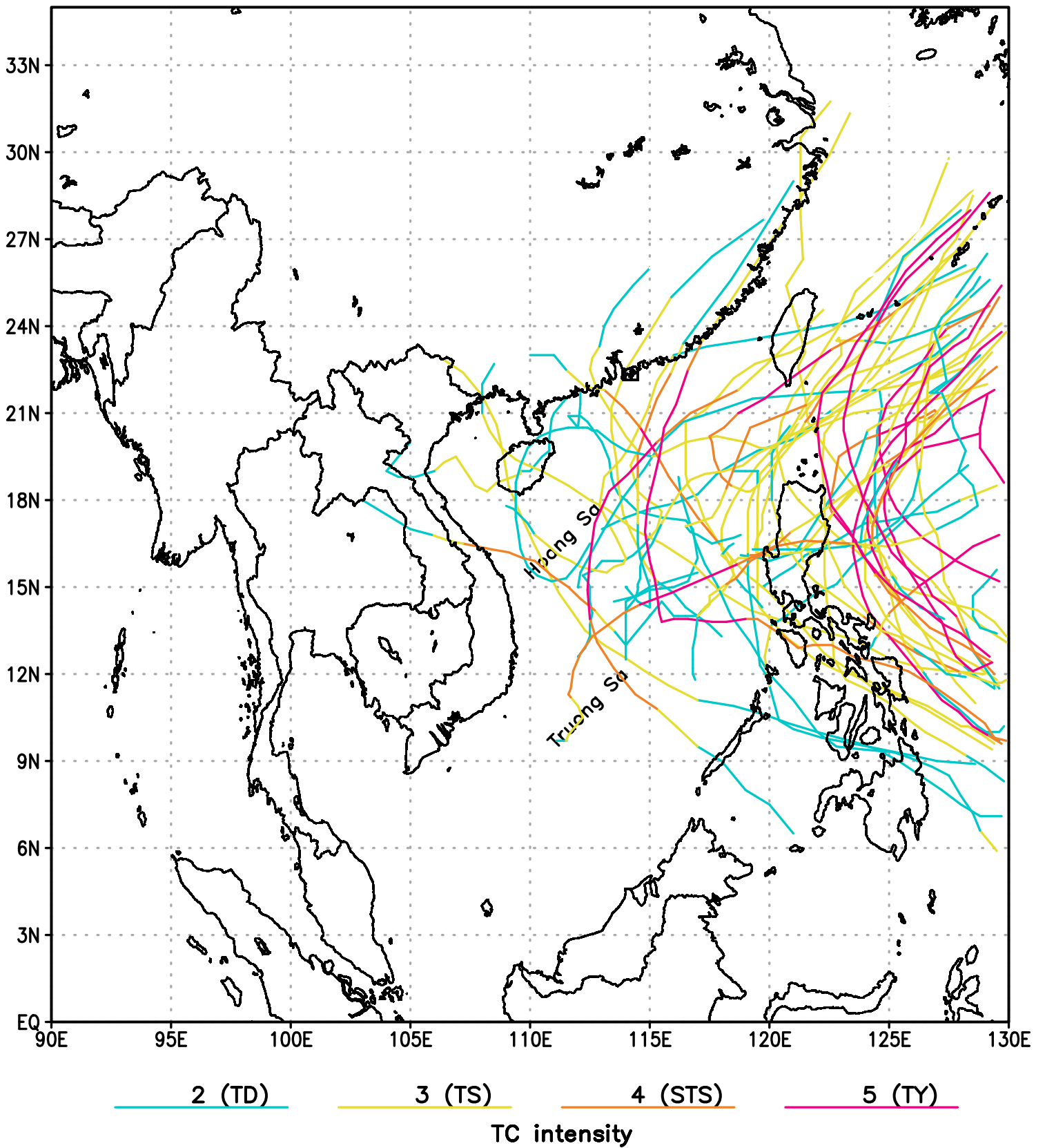
TC tracks of month 5 for period 1951–2019
