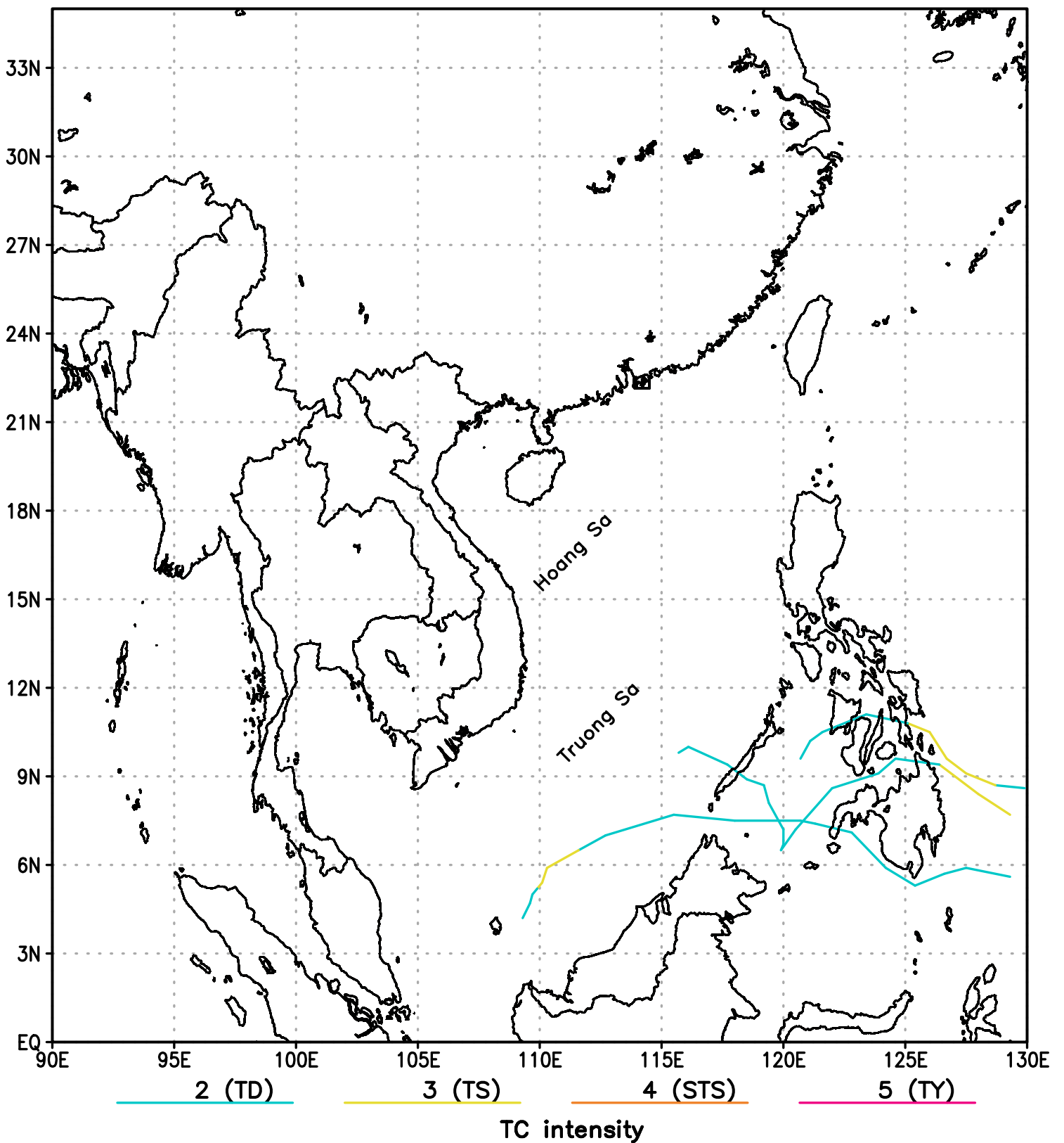
TC tracks of month 2 for period 1971–2018
