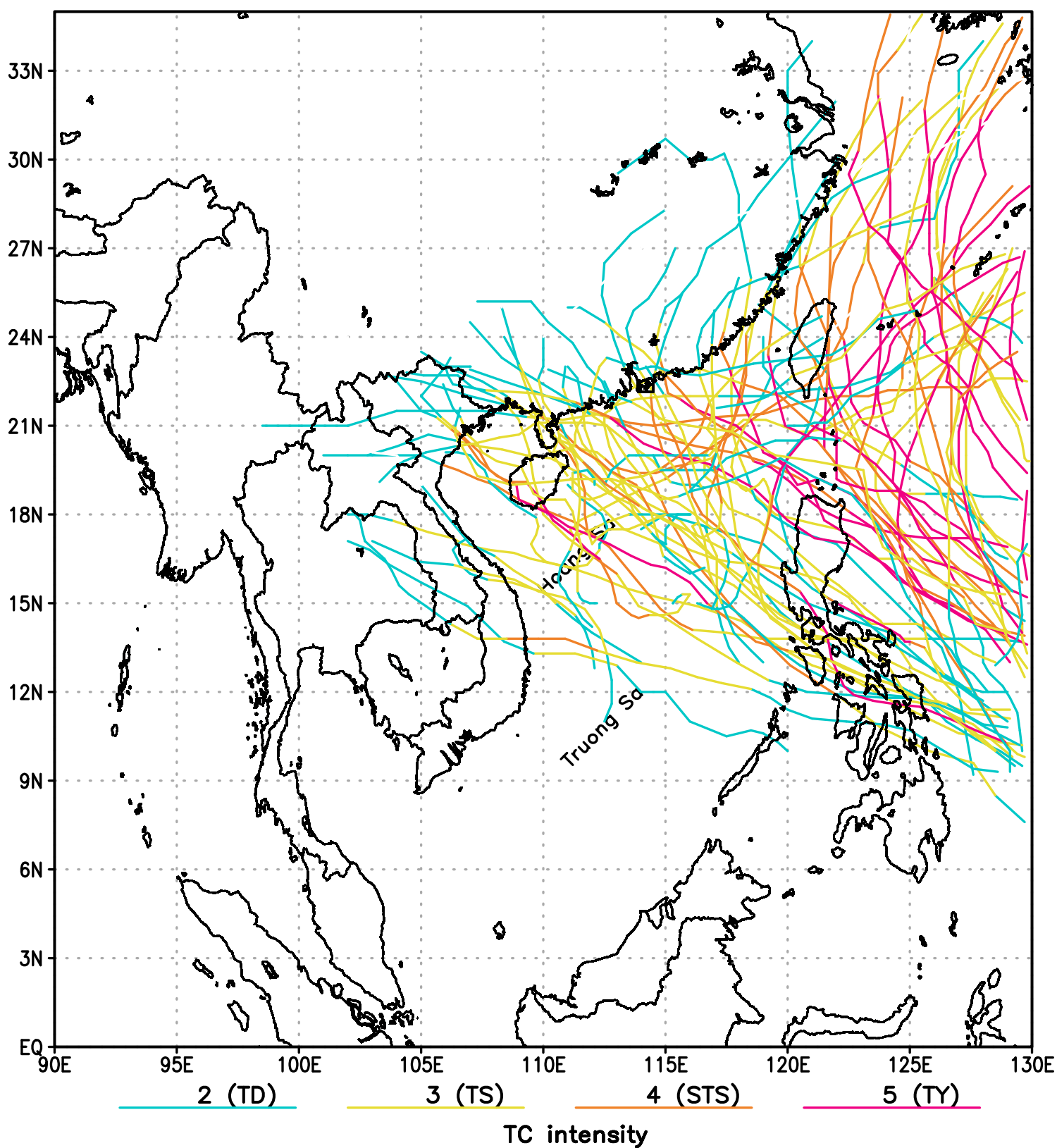
TC tracks of month 6 for period 1971–2018
