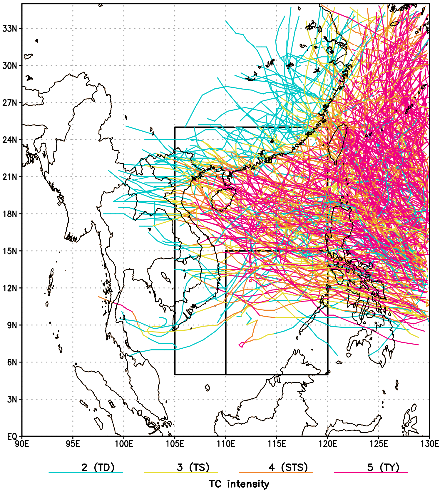
TC tracks for 1975–2014
