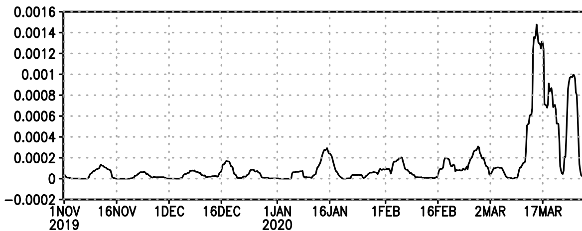
Three days running total of Rainfall (mm)
