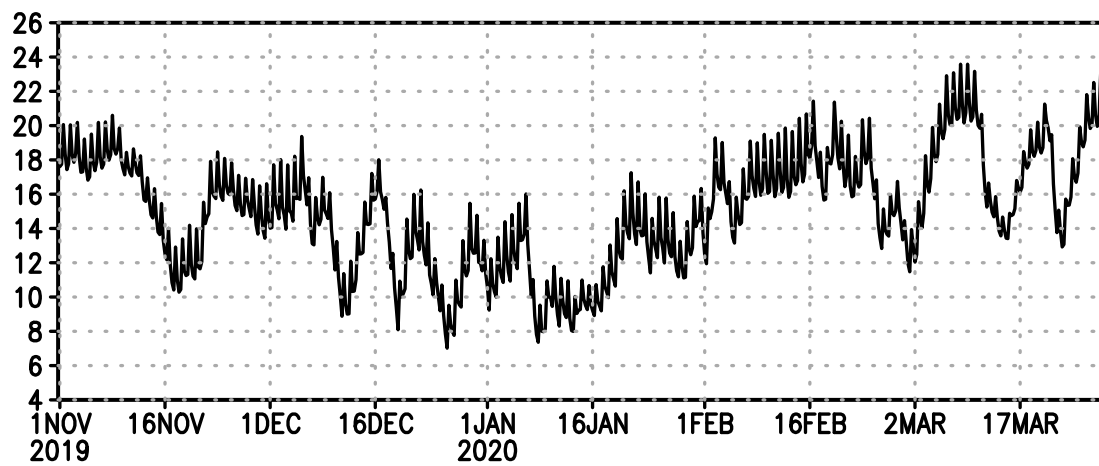
Daily 2m–Temperature (C)
