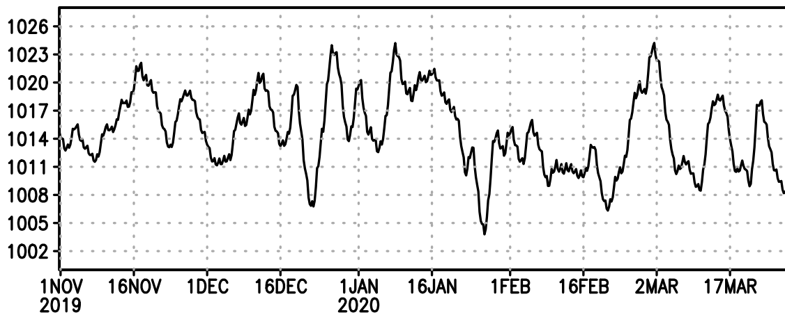
Daily Mean Sea Level Pressure (mb)
