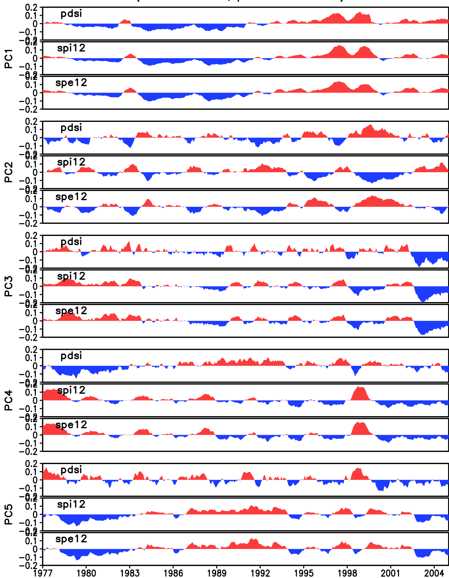
Timeseries of drought EOFs over SEA. Data from APH (APHRODITE data, period 1977–2005)
