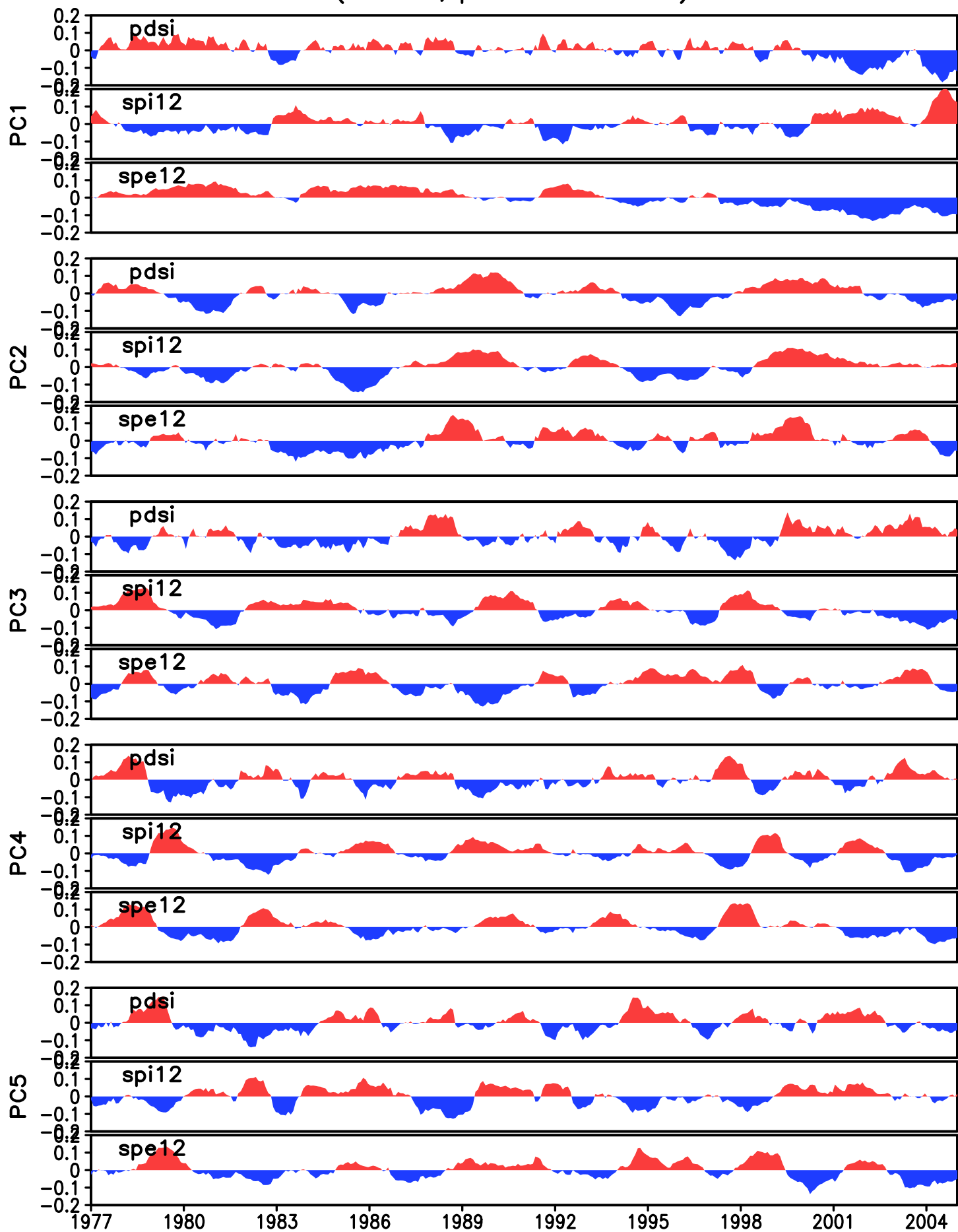
Timeseries of drought EOFs over SEA. Data from IPSL-CM5A-LR (Baseline, period 1977-2005)
