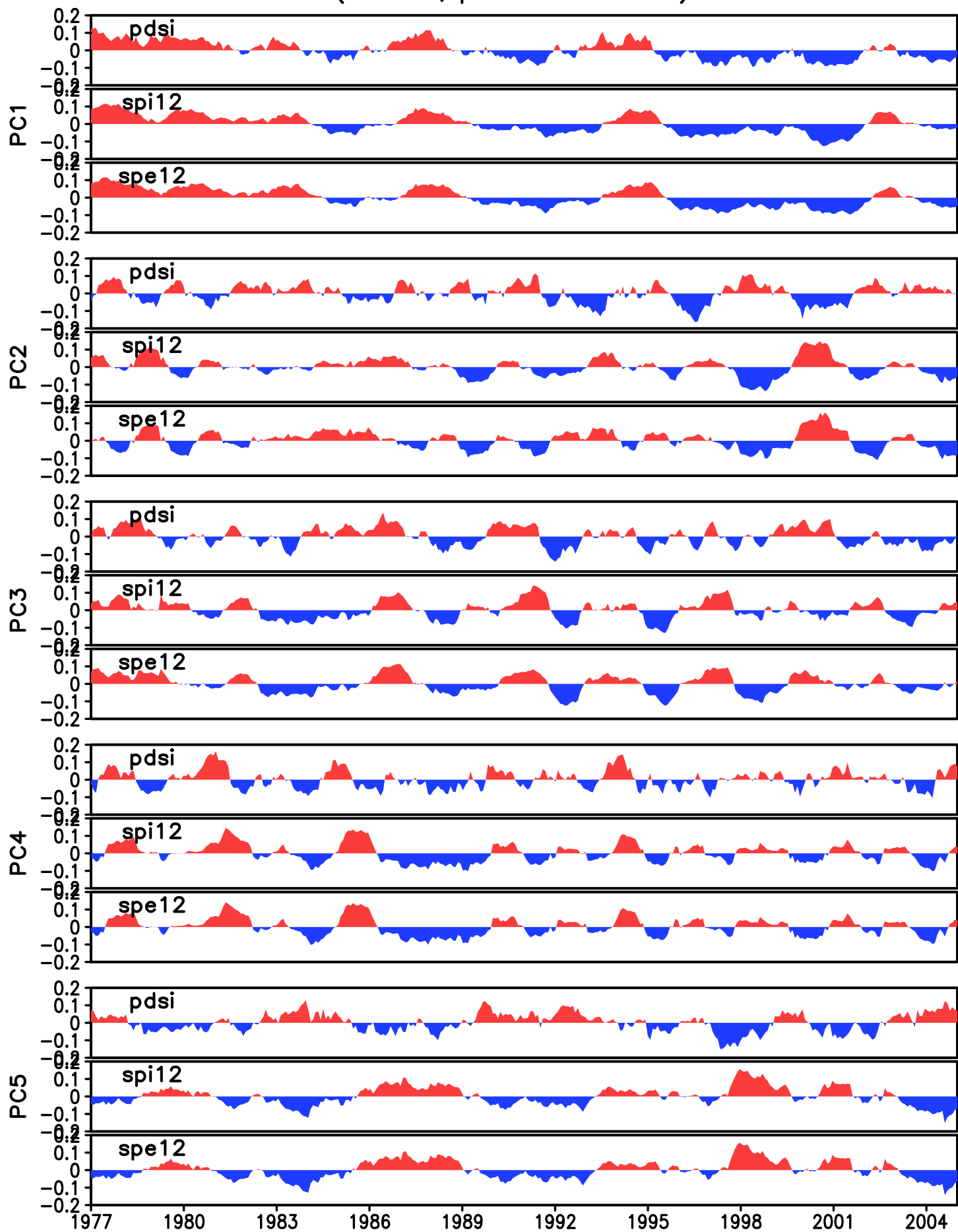
Timeseries of drought EOFs over SEA. Data from MPI-ESM-MR (Baseline, period 1977–2005)
