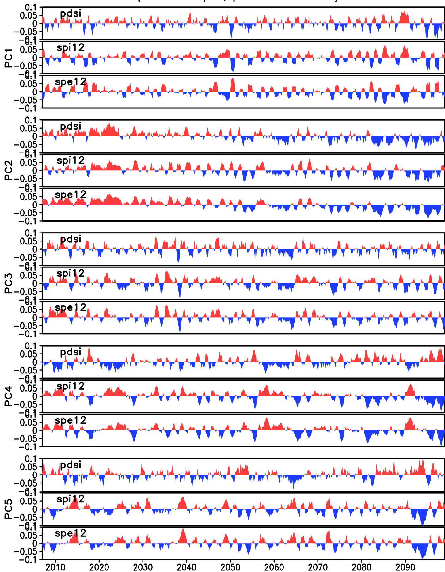
Timeseries of drought EOFs over SEA. Data from CNRM-CM5 (Scenario rcp45, period 2007–2099)
