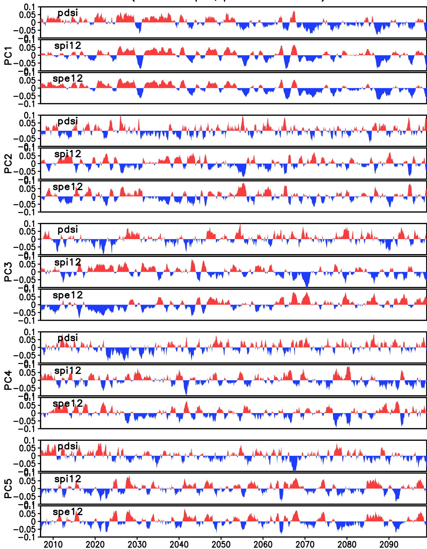
Timeseries of drought EOFs over SEA. Data from EC-EARTH (Scenario rcp45, period 2007–2099)
