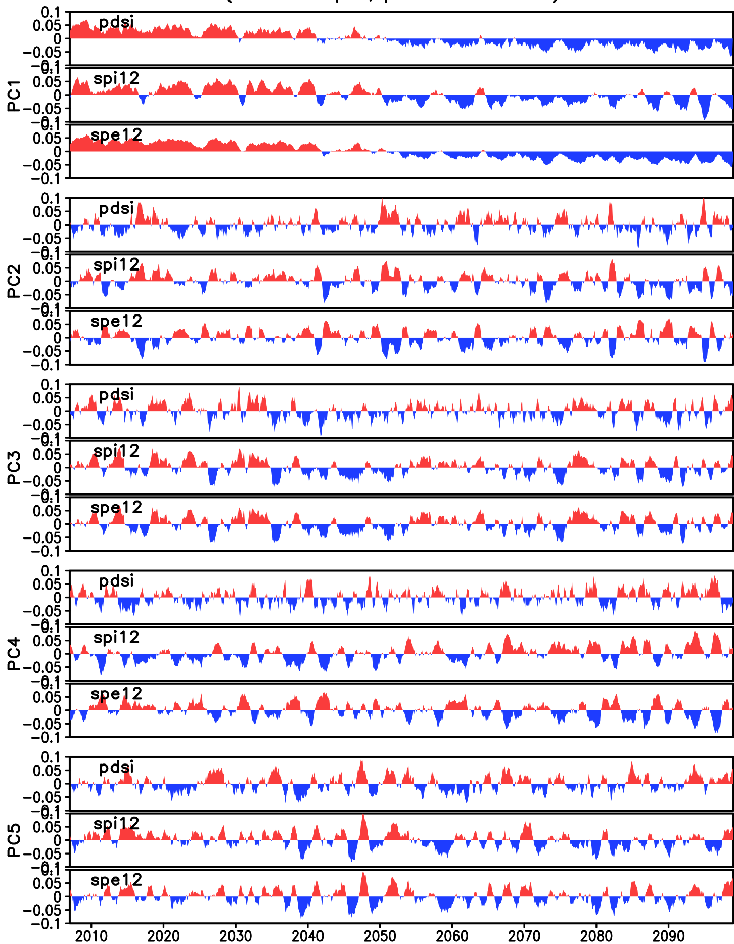
Timeseries of drought EOFs over SEA. Data from Ens (Scenario rcp45, period 2007–2099)
