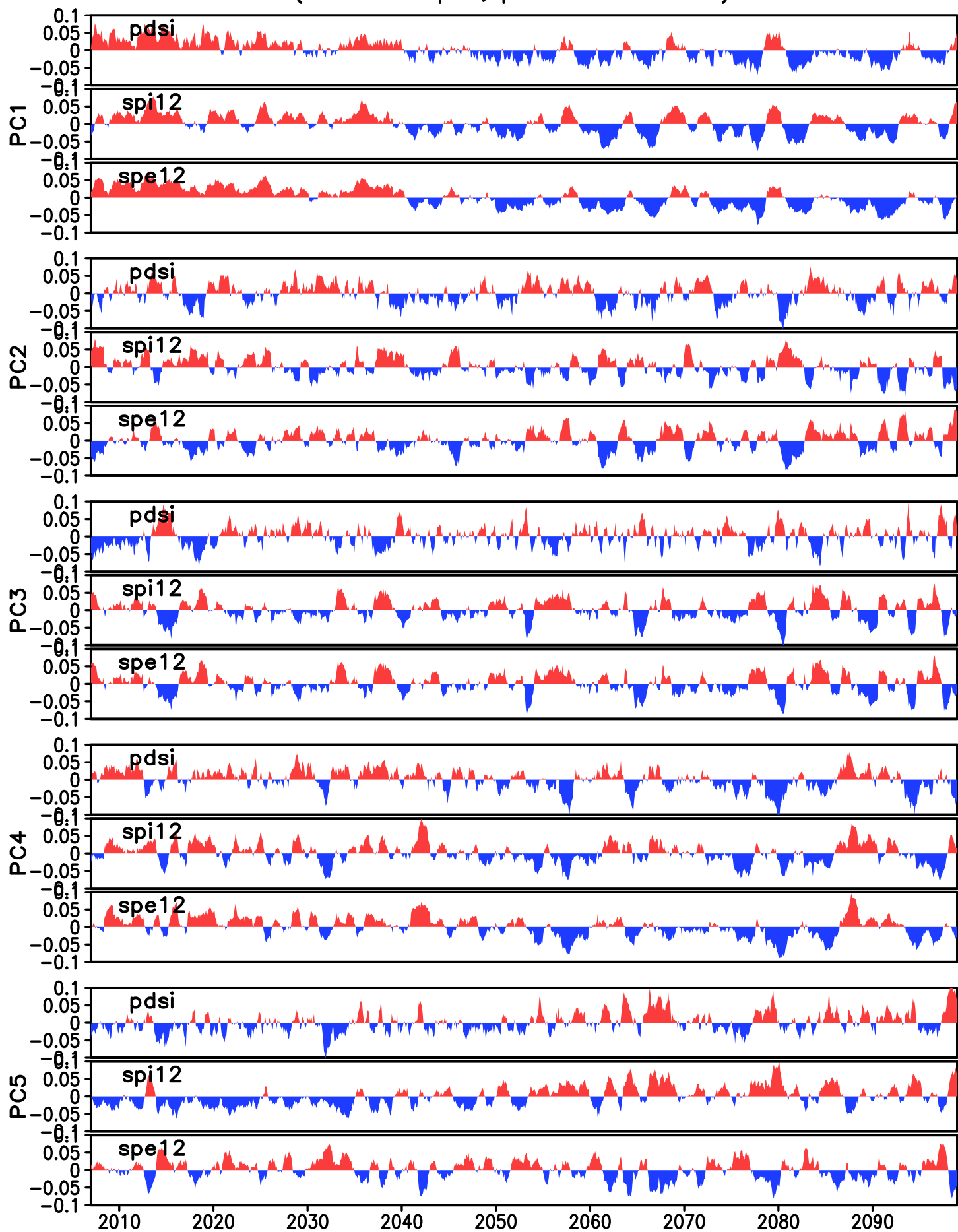
Timeseries of drought EOFs over SEA. Data from MPI-ESM-MR (Scenario rcp45, period 2007–2099)
