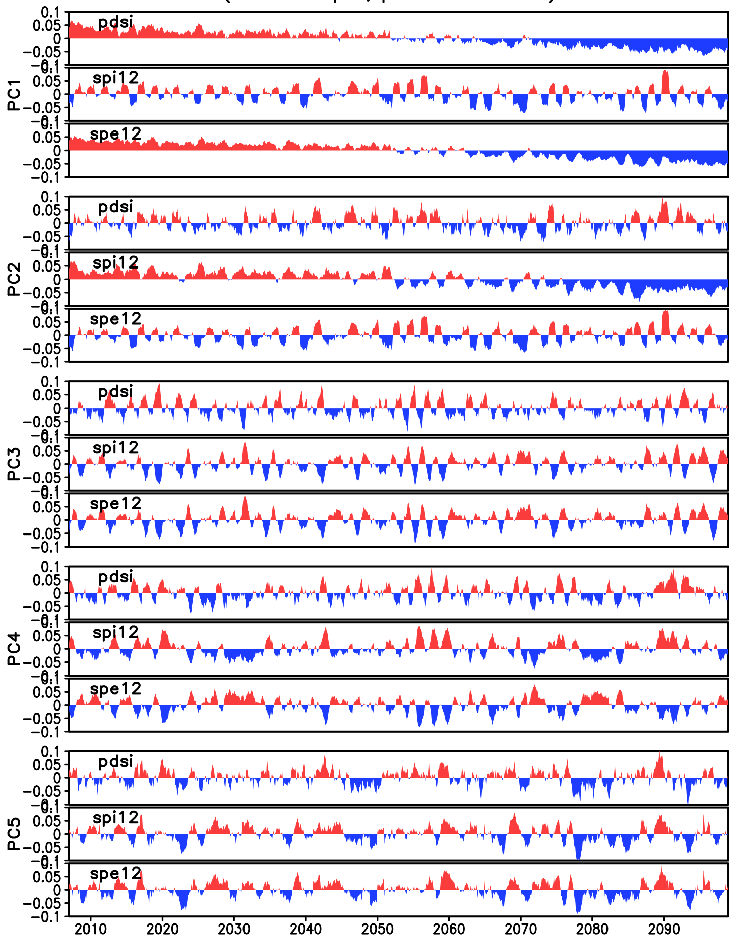
Timeseries of drought EOFs over SEA. Data from CNRM-CM5 (Scenario rcp85, period 2007-2099)
