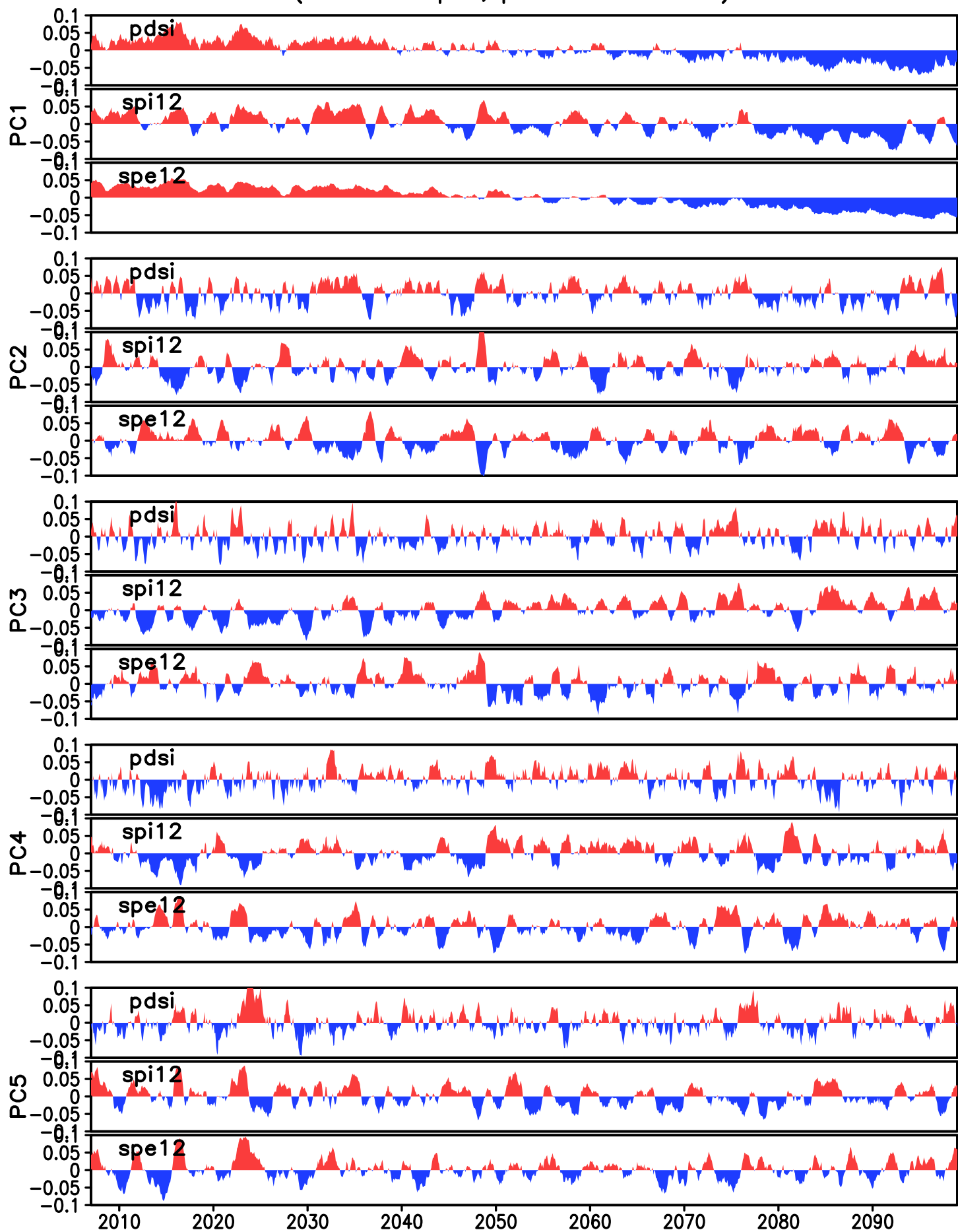
Timeseries of drought EOFs over SEA. Data from CSIRO-Mk3-6-0 (Scenario rcp85, period 2007–2099)
