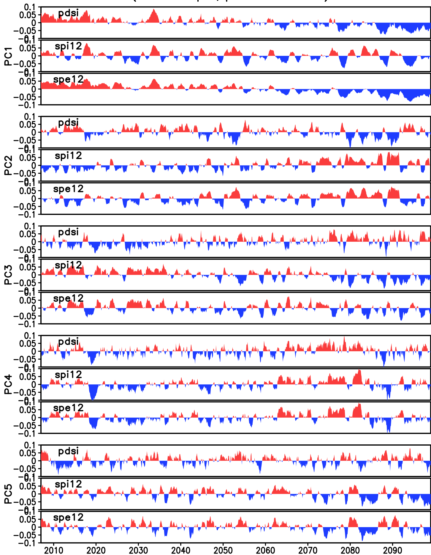
Timeseries of drought EOFs over SEA. Data from EC-EARTH (Scenario rcp85, period 2007–2099)
