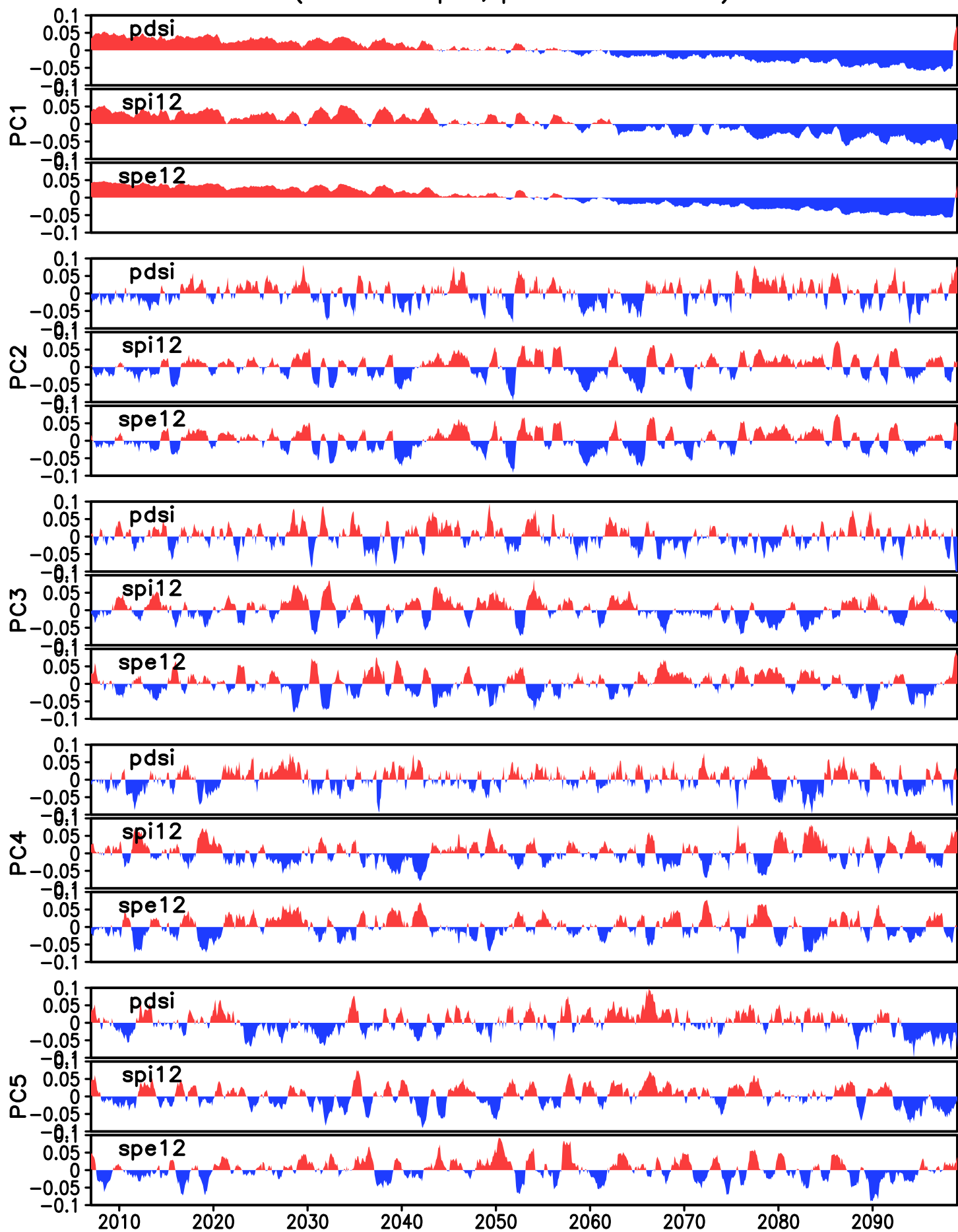
Timeseries of drought EOFs over SEA. Data from Ens (Scenario rcp85, period 2007–2099)
