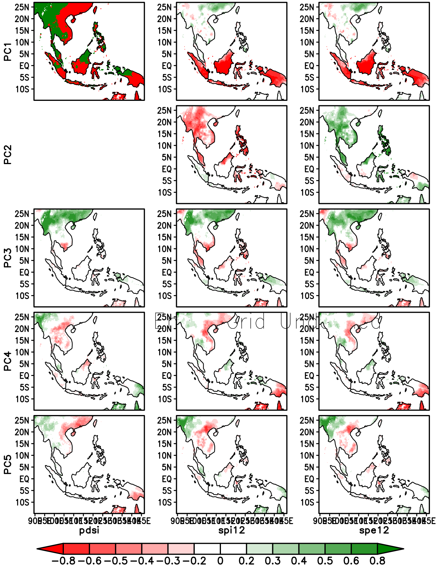
Spatial patterns of drought over SEA. Data from APH (APHRODITE data, period 1977–2005)
