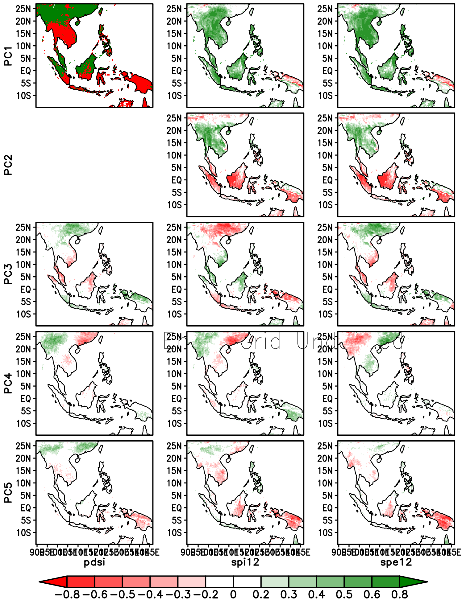
Spatial patterns of drought over SEA. Data from Ens (Baseline, period 1977–2005)
