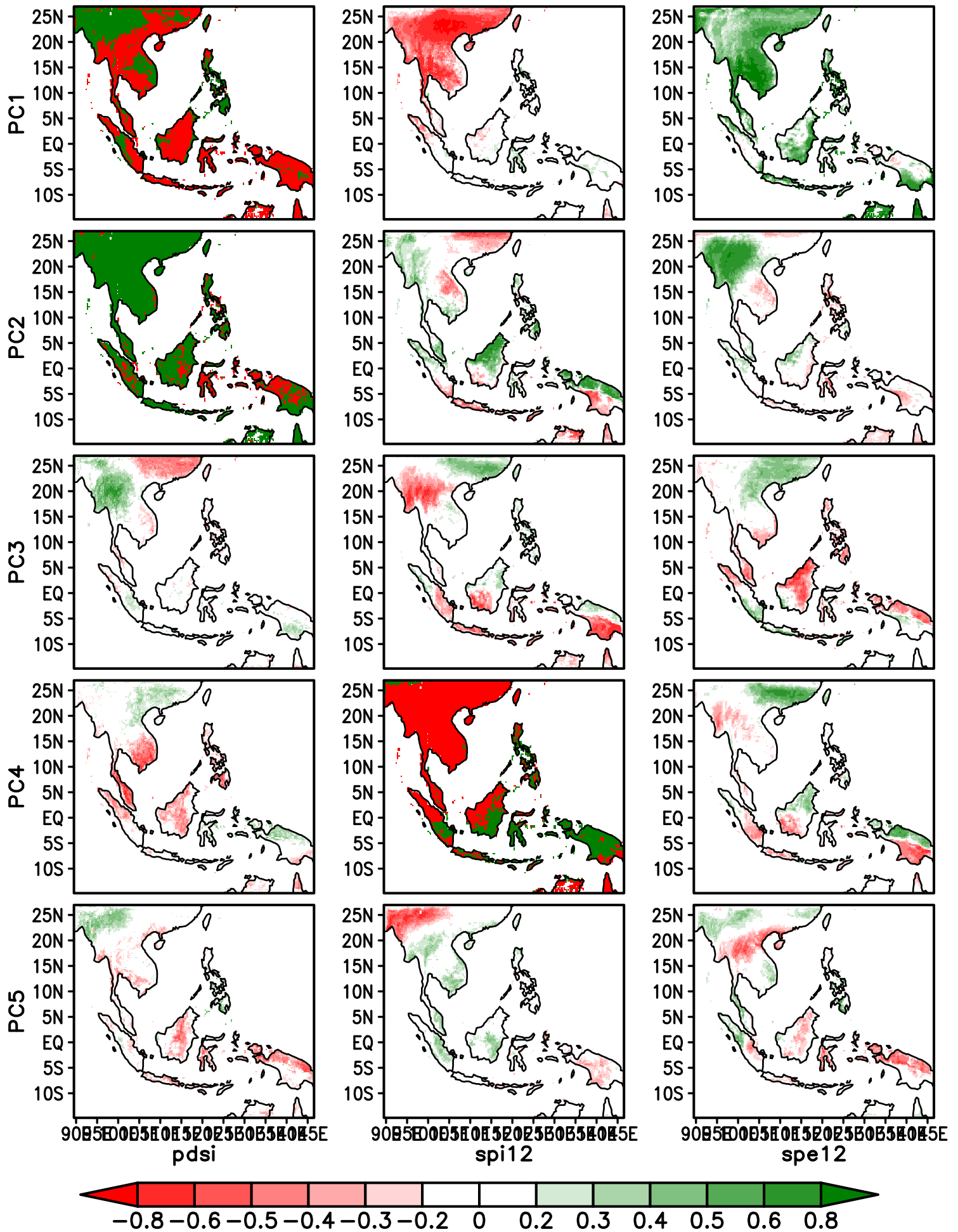
Spatial patterns of drought over SEA. Data from IPSL-CM5A-LR (Baseline, period 1977–2005)
