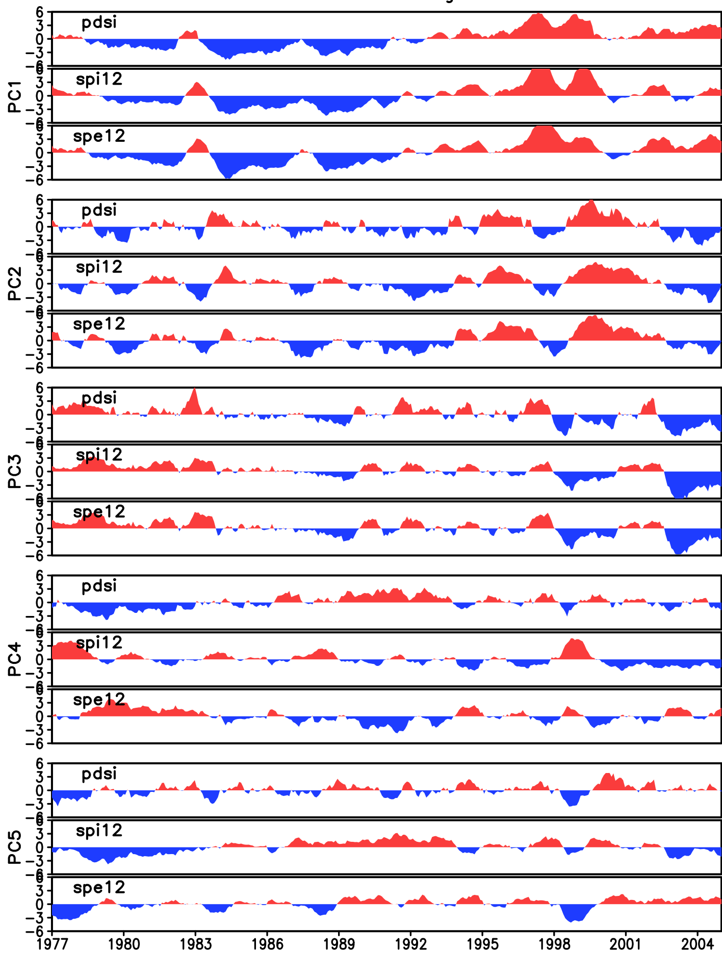
Timeseries of EOFs of drought over SEA
