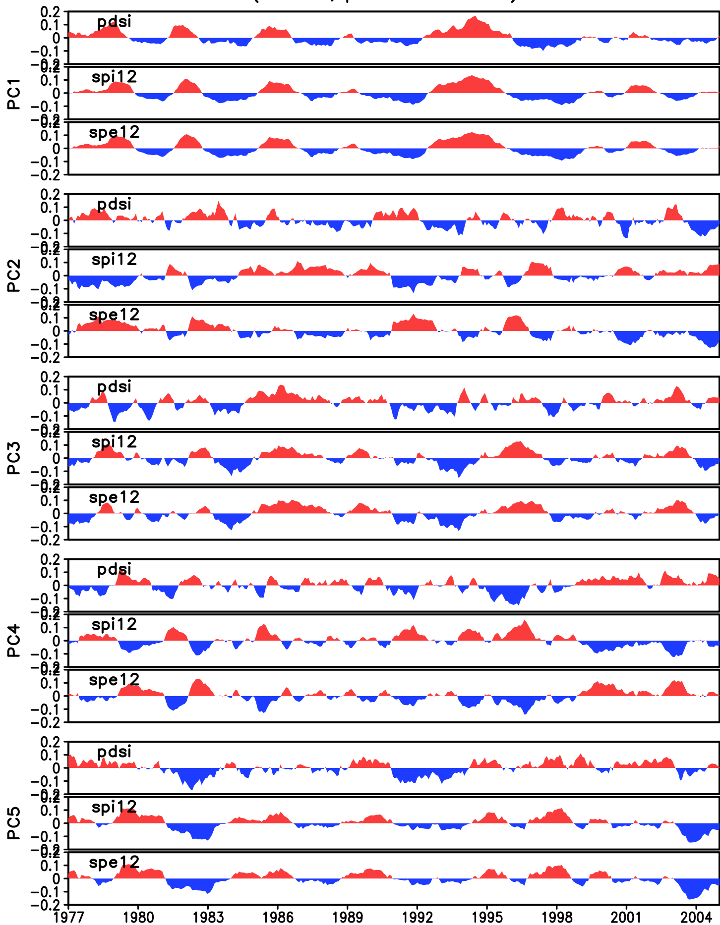
Timeseries of drought EOFs over SEA. Data from CSIRO-Mk3-6-0 (Baseline, period 1977–2005)
