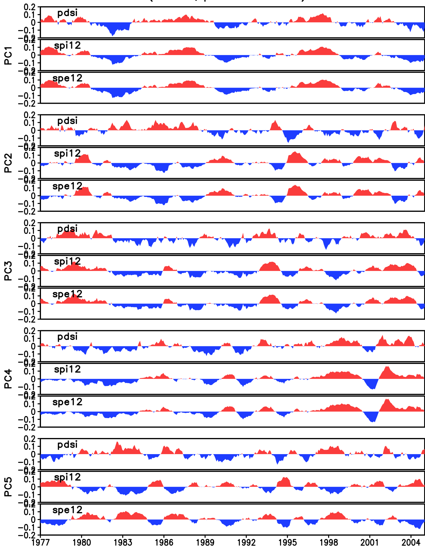
Timeseries of drought EOFs over SEA. Data from HadGEM2-AO (Baseline, period 1977–2005)
