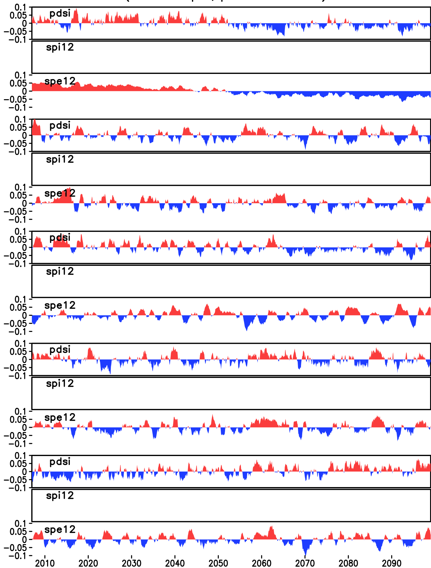
Timeseries of drought EOFs over SEA. Data from IPSL-CM5A-LR (Scenario rcp45, period 2007-2099)
