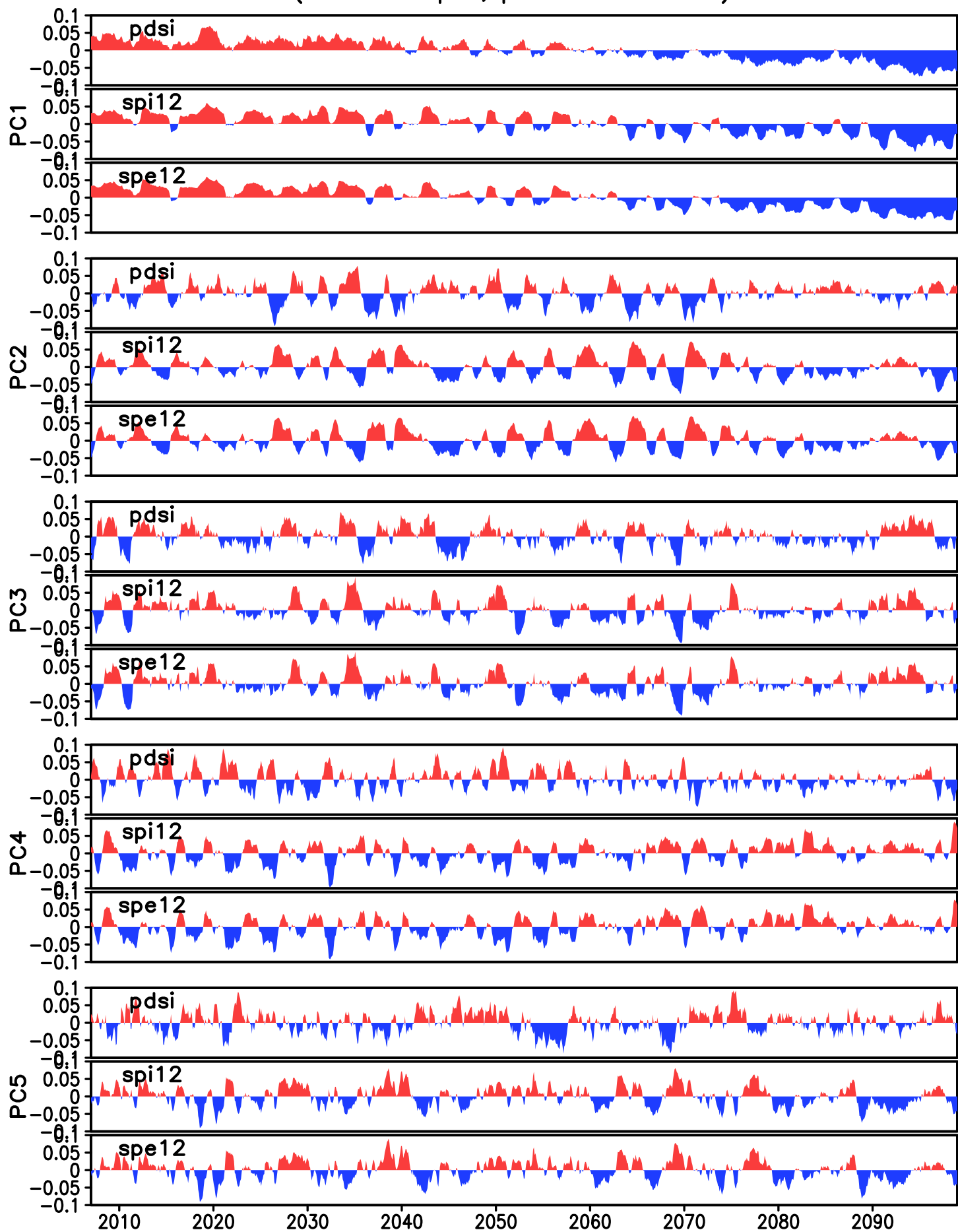
Timeseries of drought EOFs over SEA. Data from GFDL-ESM2M (Scenario rcp85, period 2007-2099)
