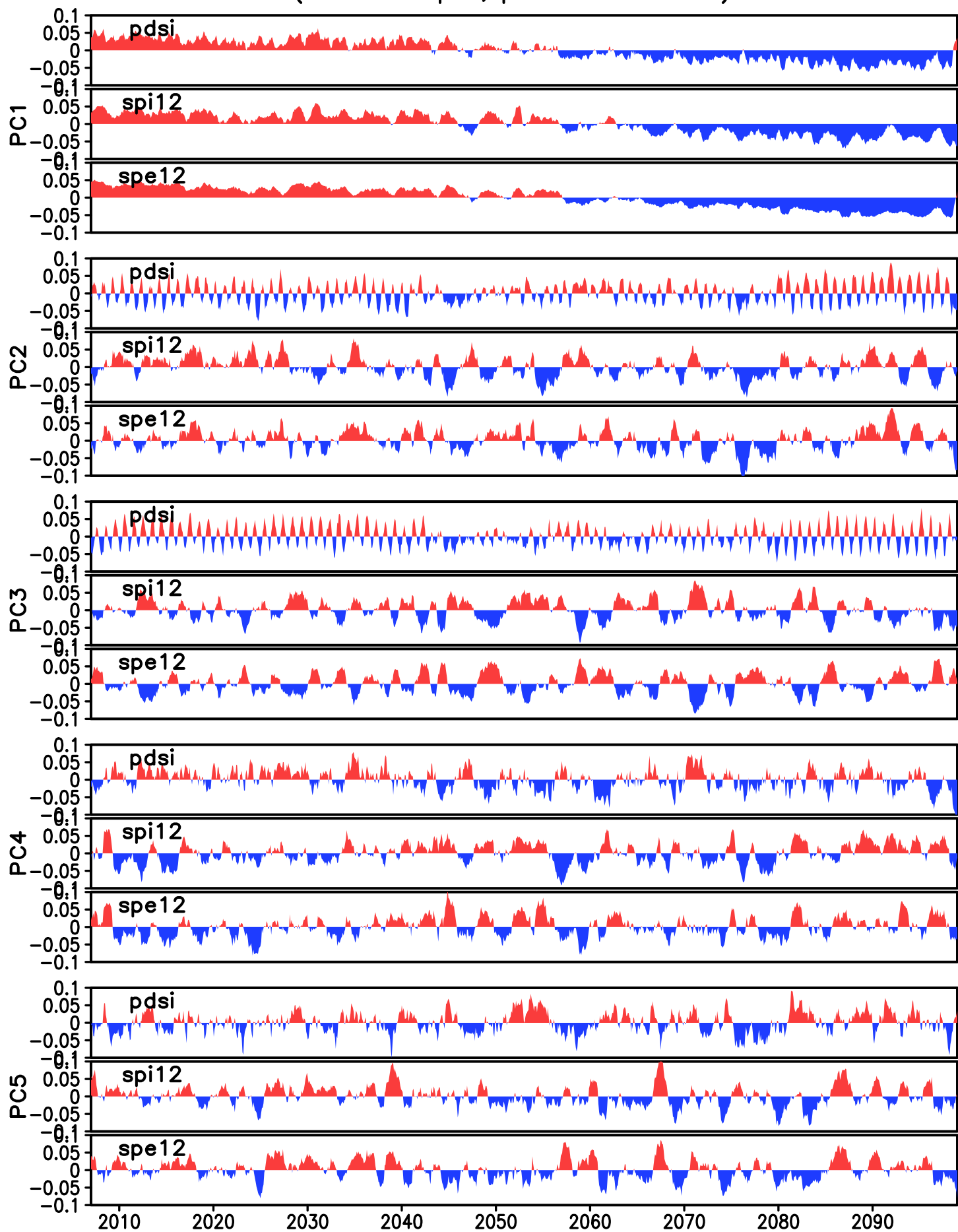
Timeseries of drought EOFs over SEA. Data from HadGEM2-AO (Scenario rcp85, period 2007–2099)
