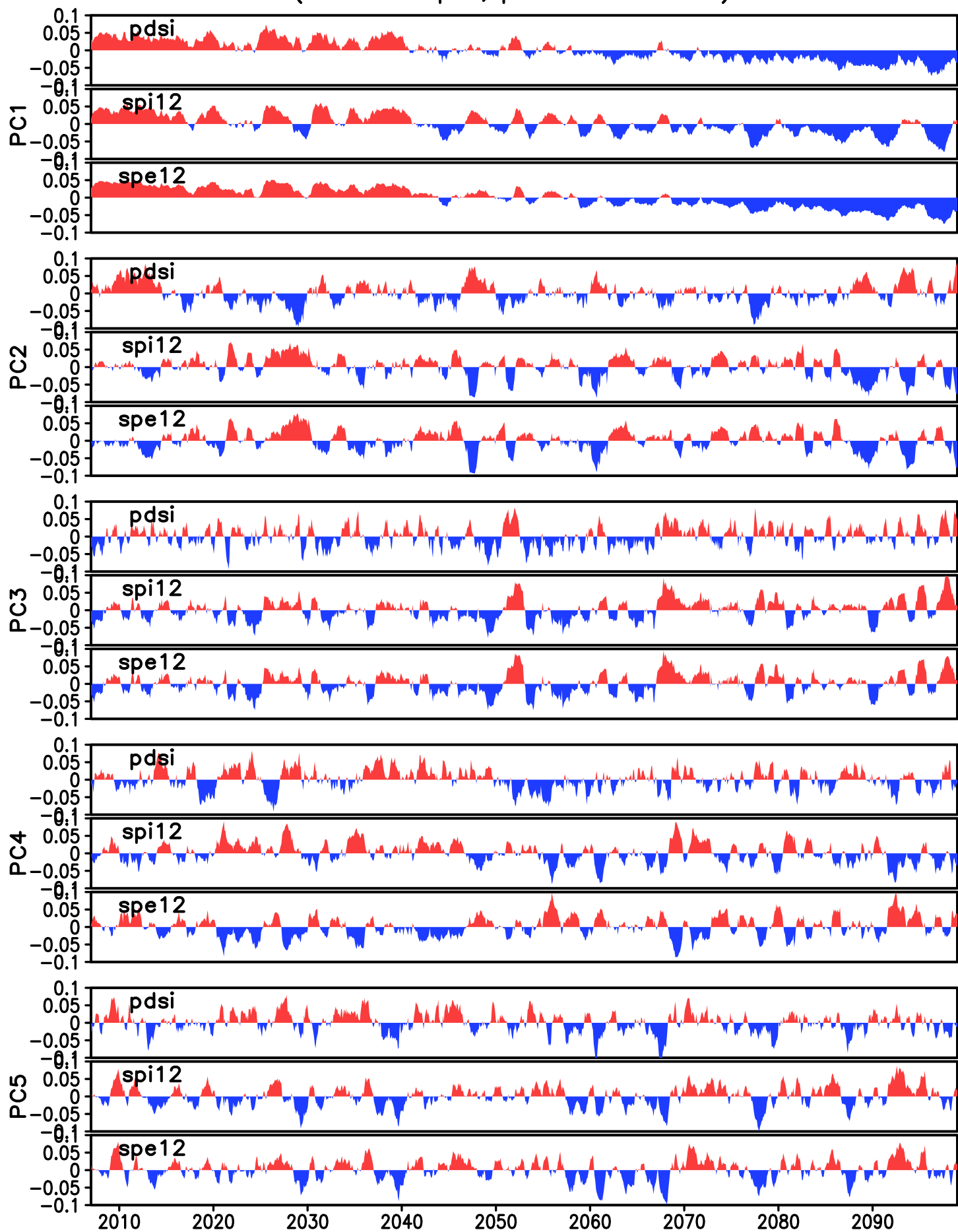
Timeseries of drought EOFs over SEA. Data from MPI-ESM-MR (Scenario rcp85, period 2007–2099)
