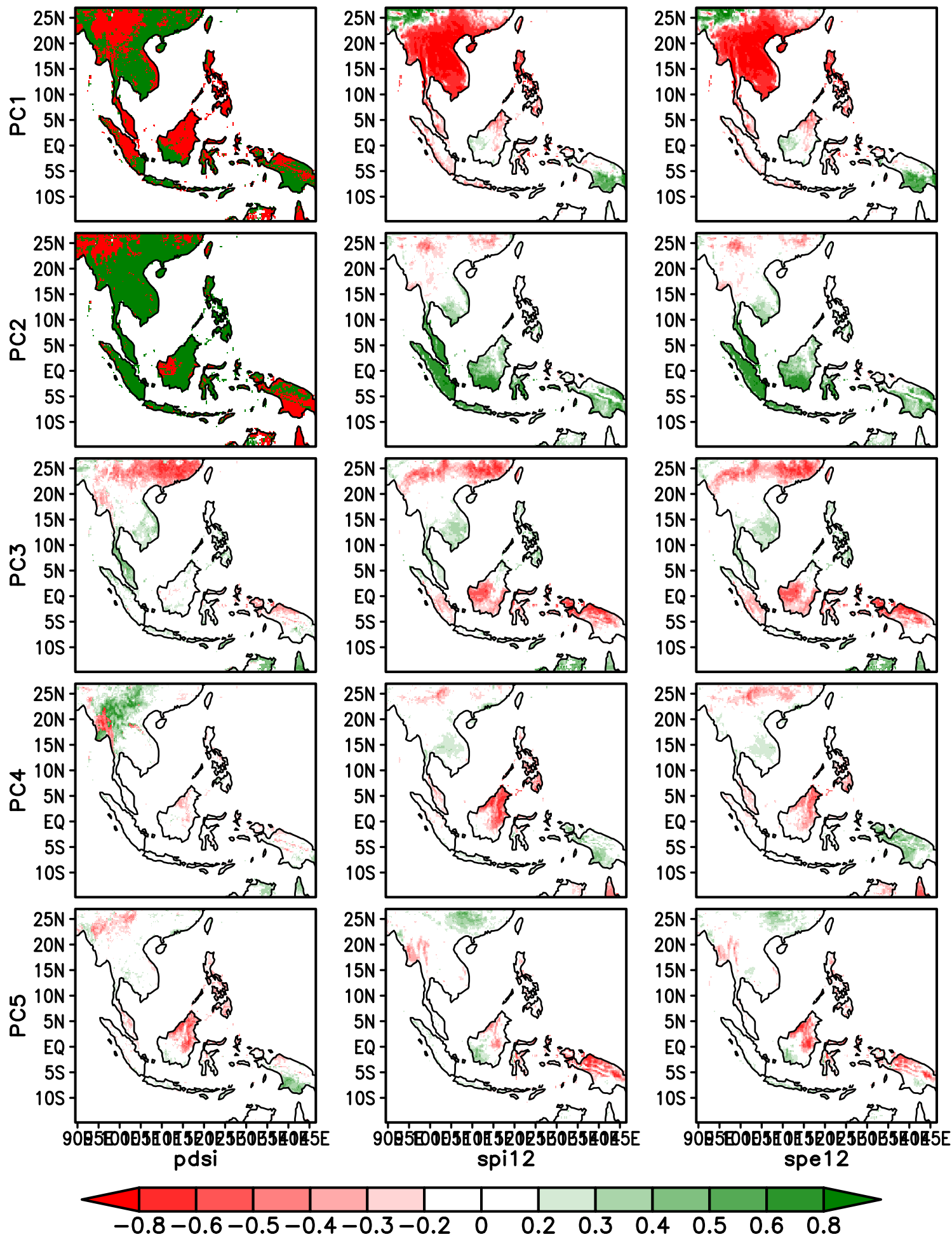
Spatial patterns of drought over SEA. Data from CNRM-CM5 (Baseline, period 1977–2005)
