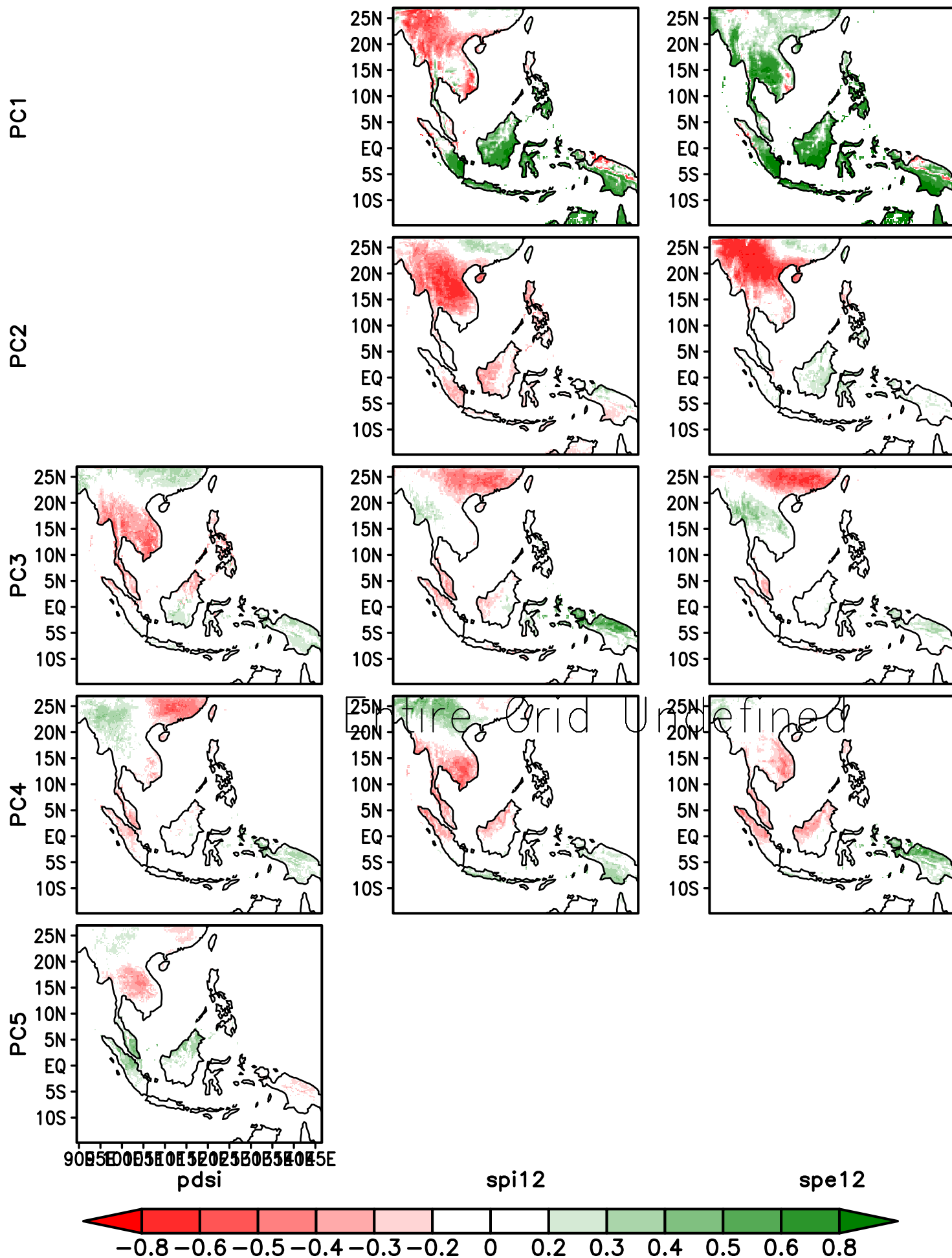
Spatial patterns of drought over SEA. Data from CSIRO-Mk3-6-0 (Scenario rcp45, period 2007–2009)
