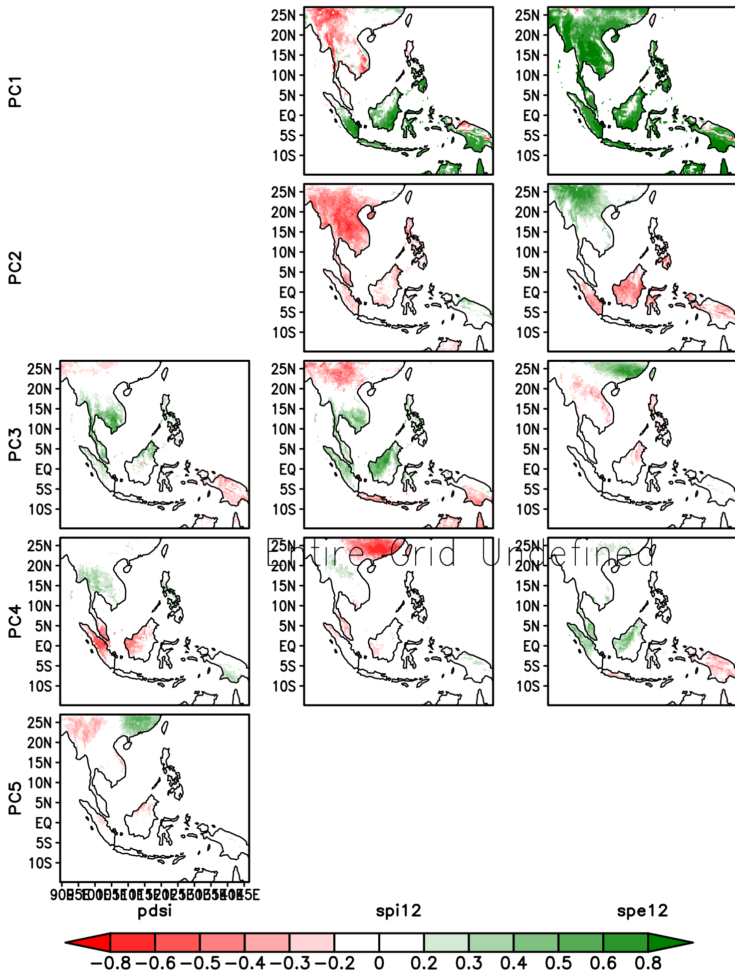
Spatial patterns of drought over SEA. Data from CSIRO-Mk3-6-0 (Scenario rcp85, period 2007–2009)
